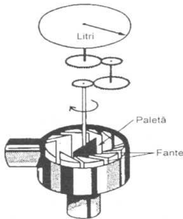
Fig.1.8 Respirometrul Wright.
