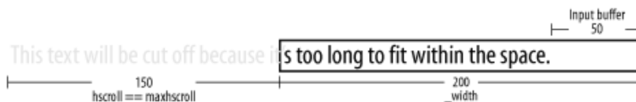
Figure 18-5. The maxhscroll property for an input text field
