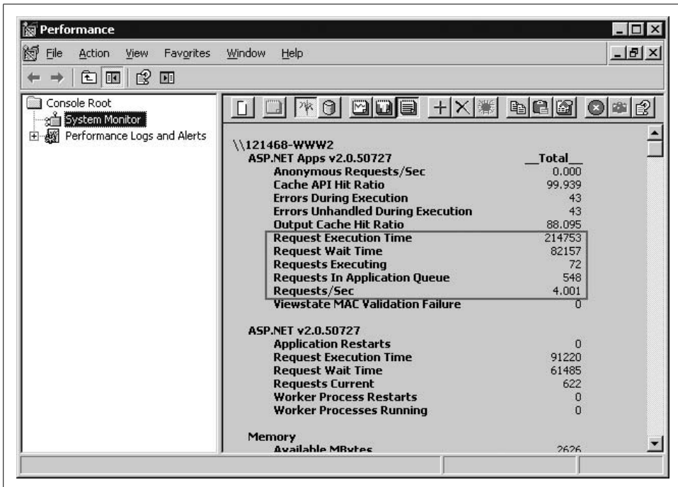
Figure 7-1. When there are too many requests for ASP.NET to handle, Requests In Application Queue starts to increase and Requests/Sec decreases. High Request Execution Time shows how long external web services requests are stuck.
