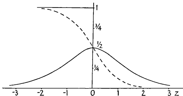
FIG. 13. The Debye functions \epsilon_2/(\epsilon_s - \epsilon_\infty) (full line), and (\epsilon_1 - \epsilon_\infty)/(\epsilon_s - \epsilon_\infty) (dotted line), according to equations 10.20.
