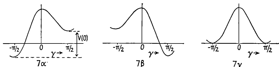
FIG. 7. Average potential energy of a dipole (due to short-range interaction) as a function of its direction for the model of Fig. 6, assuming that all the other dipoles stay in the fixed directions indicated in Fig. 6: ( \alpha ) for the central dipole of Fig. 6 b ; ( \beta ) for a corner dipole of Fig. 6 b or for any dipole of Fig. 6 a ; ( \gamma ) for the disordered case, Fig. 6 c .
