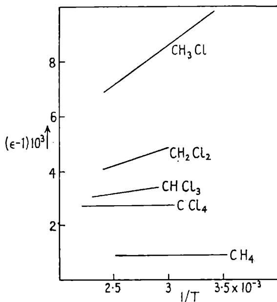
FIG. 22. Temperature-dependence of the dielectric constant of various gases according to Sanger [51].
