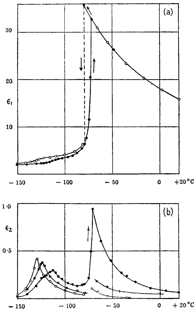
FIG. 35. (a) Dielectric constant \epsilon_1 , and (b) dielectric loss \propto \epsilon_2 of di-isopropyl ketone according to Schallamach [S4]; —○— at a frequency of 1.2 Mc./s., —●— at 4.4 Mc./s., —●— at 20 Mc./s. Melting occurs near -73^\circ\text{C} . and there is no previous transition.
