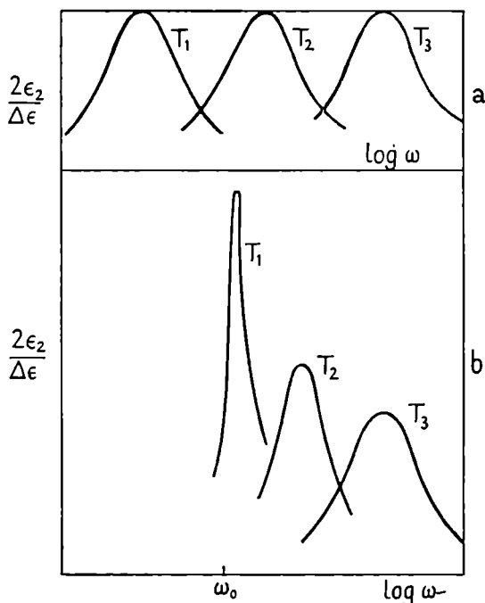
FIG. 17. Frequency dependence of dielectric loss for three different temperatures T_1 < T_2 < T_3 (schematically). (a) Debye case; (b) resonance case.
