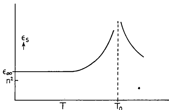
FIG. 10. Temperature-dependence of the dielectric constant of a dipolar solid showing an order-disorder transition, schematically.
