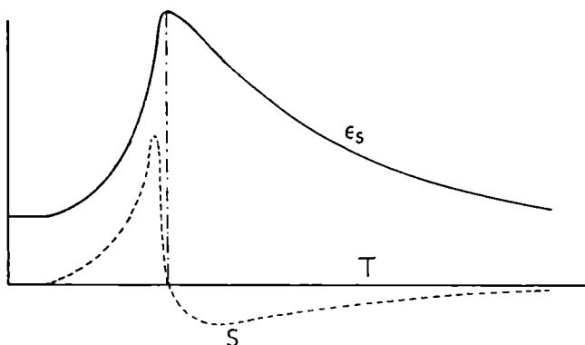
FIG. 3. Schematic temperature-dependence of the dielectric constant \epsilon_s and of the entropy change S \propto \partial\epsilon_s/\partial T due to the polarization by a field. If S > 0 the field creates disorder, if S < 0 it creates order. Near the absolute zero of temperature the substance is already perfectly ordered. Hence \partial\epsilon_s/\partial T cannot be negative near T = 0 .
