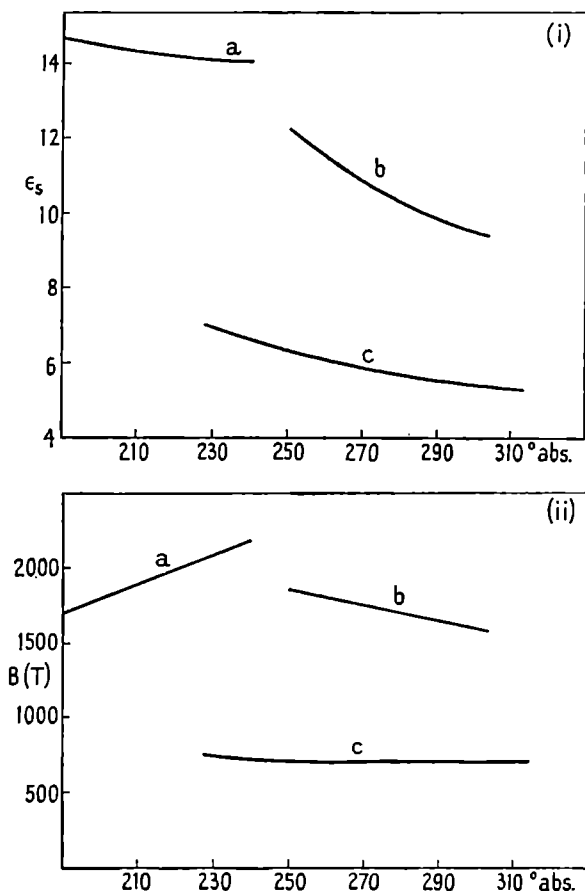
FIG. 38. Examples of \epsilon_s - T analysis. (ii) Temperature-dependence of the function B(T) obtained from \epsilon_s(T) (cf. i) with the help of equation 17.5. (a) Dichloro-propane, (\text{CH}_3)_2\text{CCl}_2 , solid, using \epsilon_s(0) = 2.23 . (b) Tertiary-butyl-chloride, (\text{CH}_3)_3\text{CCl} , liquid, using \epsilon_s(0) = 2.45 . (c) Penta methyl-chlor-benzene, (\text{CH}_3)_5\text{Cl} , solid, using \epsilon_s(0) = 2.8 . Measurements: (a), (b) Turgewich and Smyth [T2]; (c) White, Biggs, and Morgan [W3].
