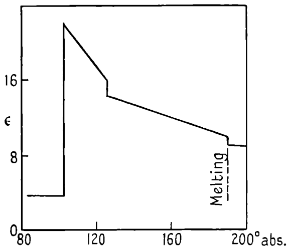
FIG. 33. Temperature-dependence of the dielectric constant of solid hydrogen sulphide according to Smyth and Hitchcock [ S9 ] showing an order-disorder transition near 103^\circ abs. A further transition and melting are of little influence.
