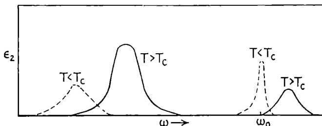
FIG. 36. Frequency-dependence of dielectric loss, ——— above and ---- below the transition temperature T_c (schematically). \omega_0/2\pi represents the lowest resonance frequency which is usually in the far infra-red or in the ultra-high electric frequency region.
