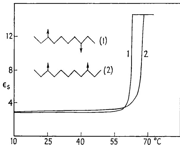
FIG. 47. Temperature-dependence of the dielectric constant of the two diketones C_{10}H_{18}O_2 (1) and C_{11}H_{20}O_2 (2) according to Muller [M8]. The molecular chains in the untwisted state are shown as zigzags, the arrows indicating the directions of the dipolar ketone groups.
