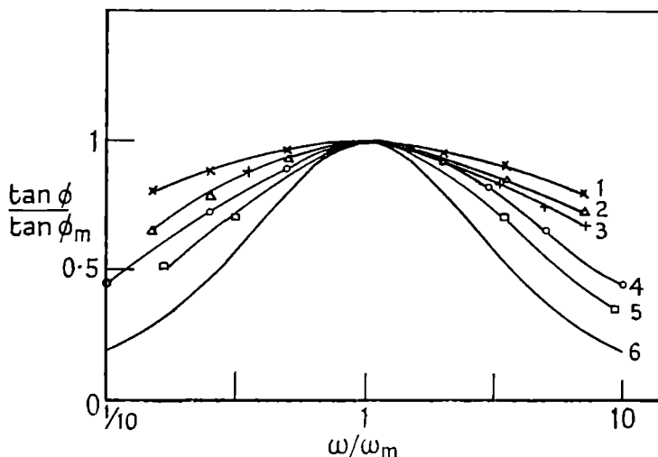
FIG. 37. Frequency-dependence of loss angle according to Hartshorn, Megson, and Rushton [H1] for various materials.
