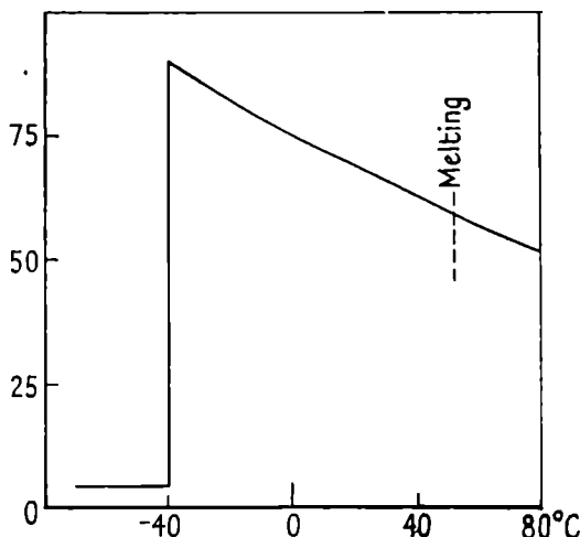
FIG. 34. Temperature-dependence of the dielectric constant of solid ethylene cyanide according to White and Morgan [W4] showing an order-disorder transition near -40^\circ\text{C} . without a discontinuity at melting.
