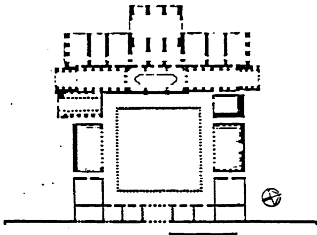
5 The Harbor Bath-Gymnasium, Ephesus. Plan (redrawn by the author from Keil, JOAI, Beiblatt , xxviii, 1933, fig. 9)
