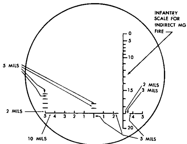
Figure 112. The binocular reticle.
