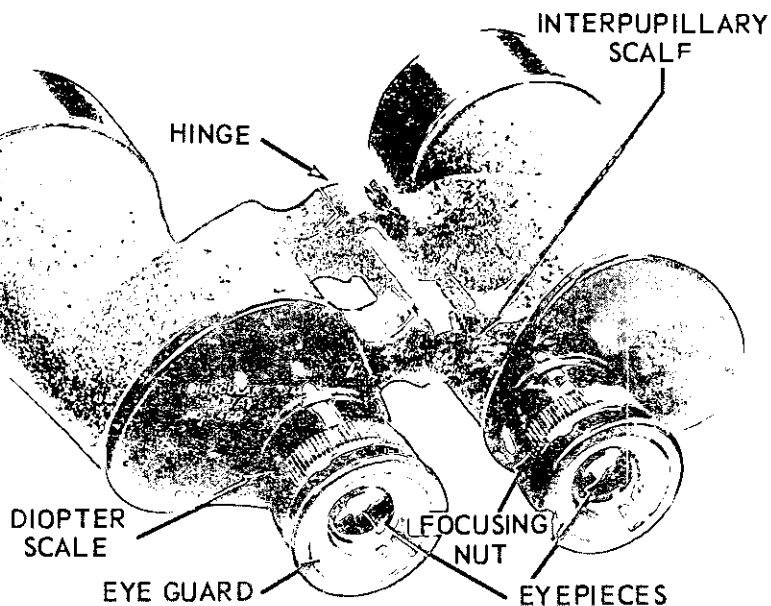
Figure 111. The binocular.
