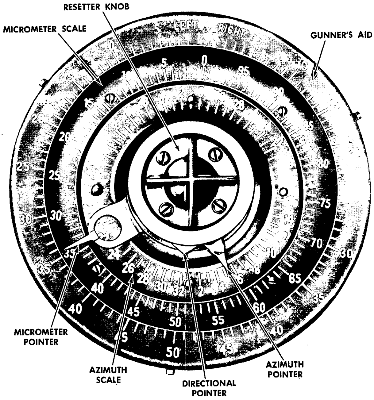
Figure 37. Azimuth indicator.
