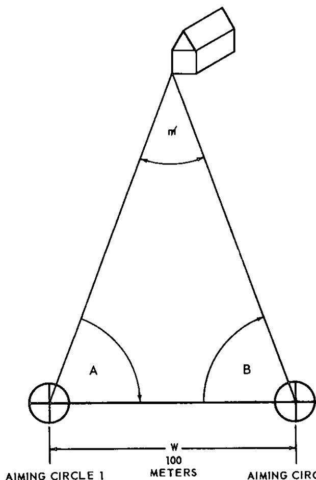
Figure 108. Determining range by intersection—summation of angles method.
