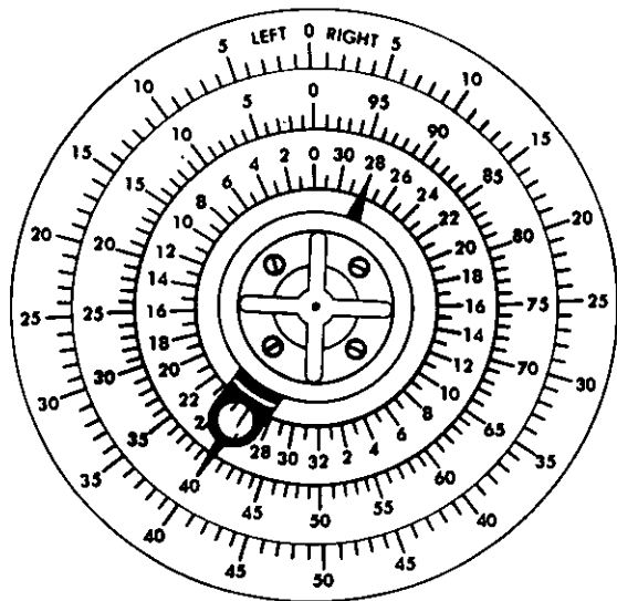
Figure 63. Azimuth indicator.
