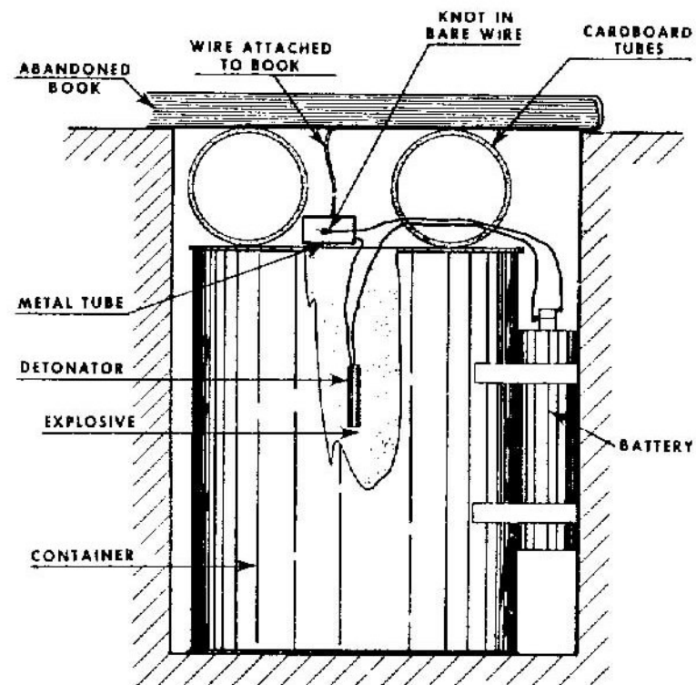
Figure 44 (UNCLASSIFIED). FLN book boobytrap (U).
