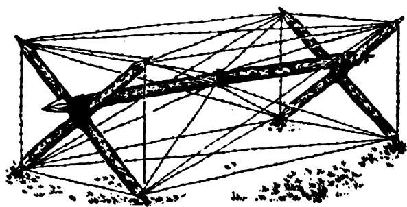
Figure 6-38. Knife rest.
