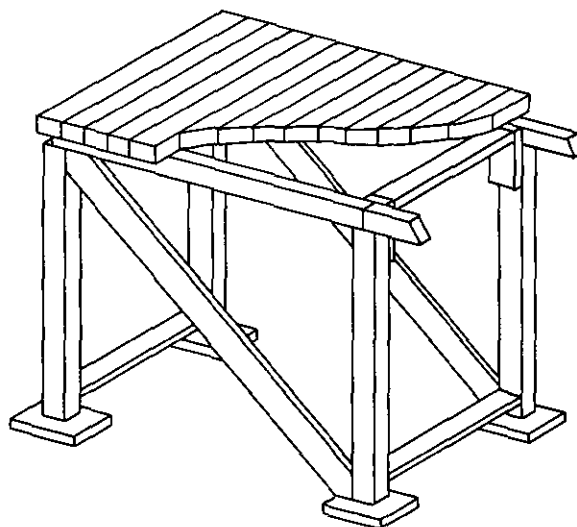
TYPICAL TRENCH COVER SECTION
