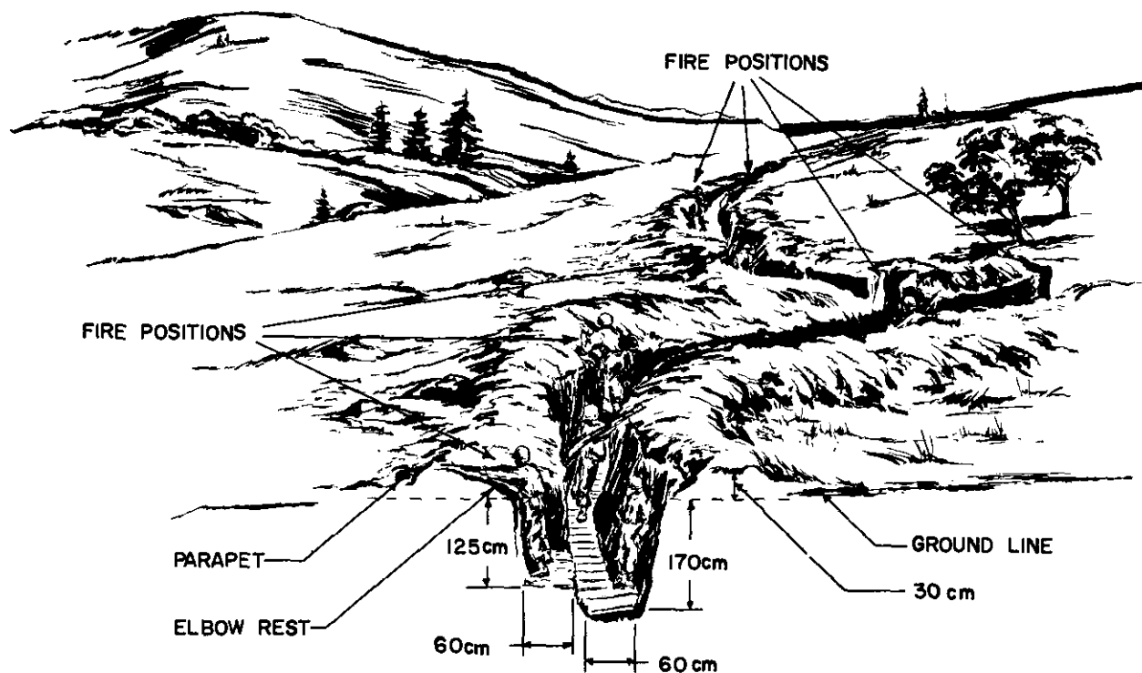
Figure 4-3. Standard trench.
