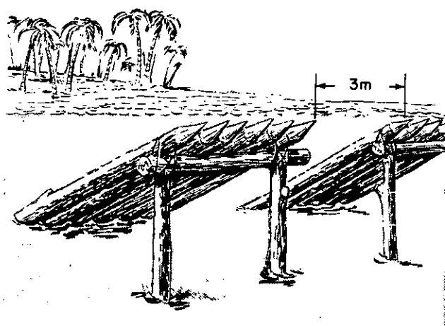
Figure 8-7. Log ramps.
