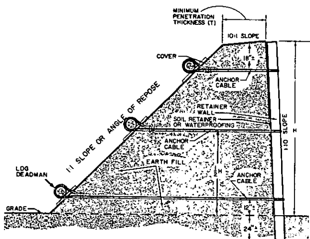
Figure 2-29. Gravity revetment.
