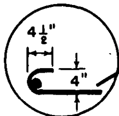
180° HOOK DETAIL
