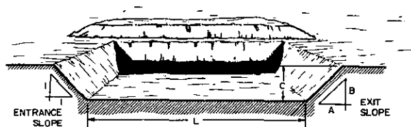
Figure 2-24. Typical vehicle pit.
