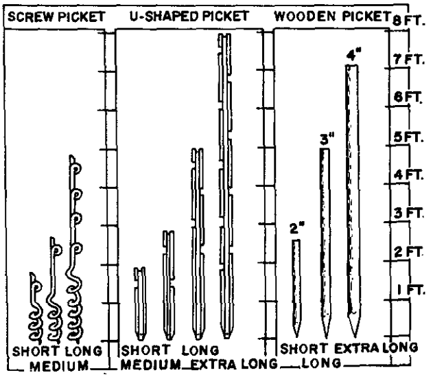
Figure 6-10. Pickets for use with barbed wire.
