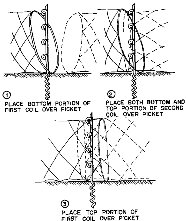
Figure 6-28. Joining concertina.
