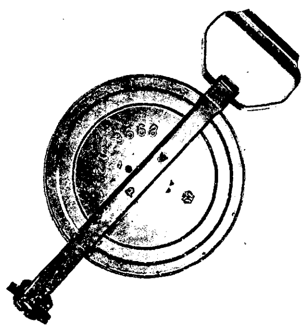
Figure 6-9. Barbed tape dispenser with 50-meter reel of tape.
