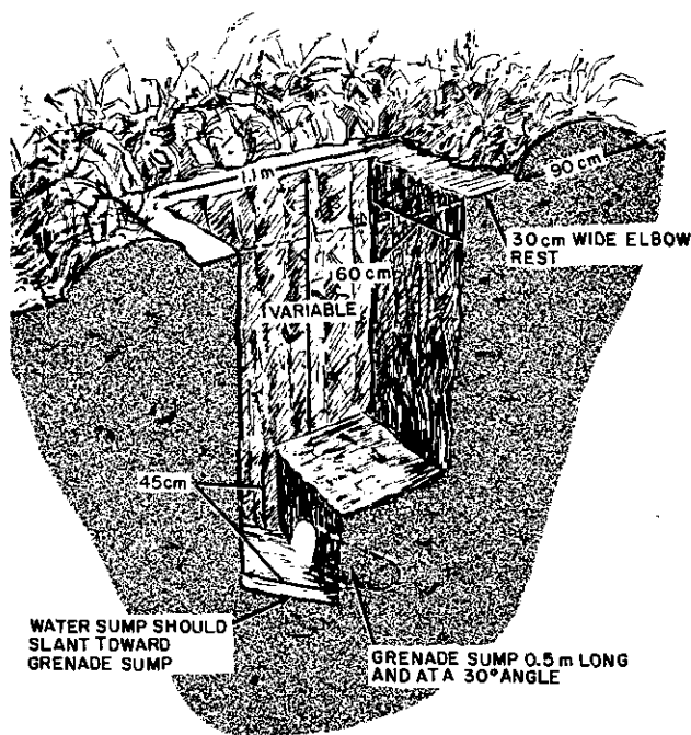
Figure 2-8. One-man foxhole.
