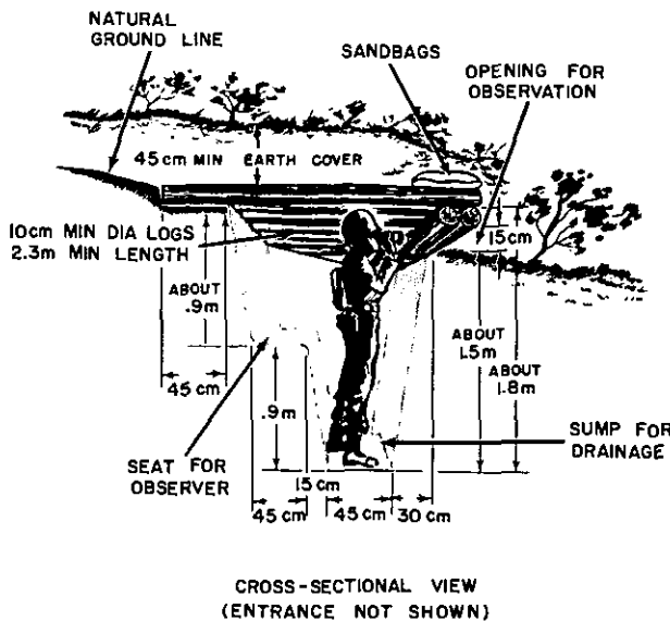
Figure 3-15. Observation post.
