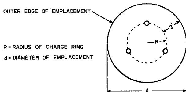
Figure D-4. Layout of boreholes when diameter of emplacement exceeds 1½ but not more than 3 times the depth of the boreholes.
