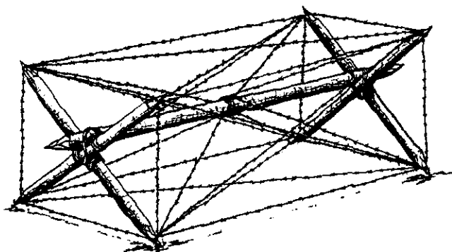
Figure 6-33. Knife rest.
