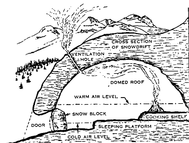
Figure 3-5. Snow cave.
