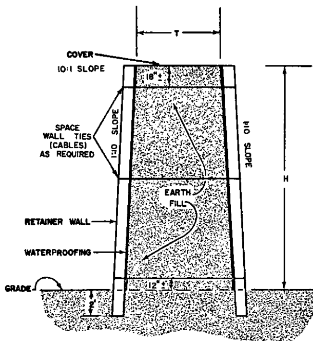
Figure 2-31. Bulkhead revetment.
