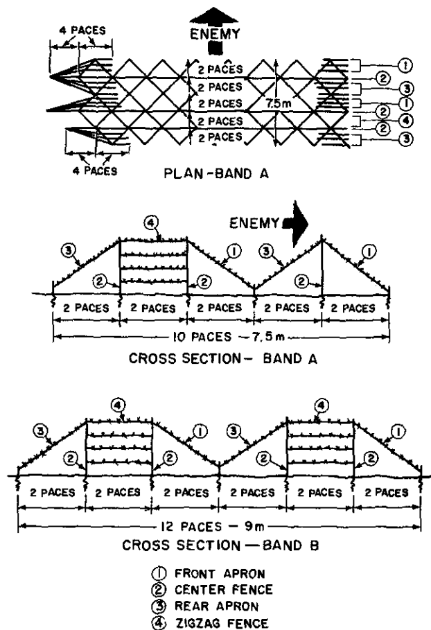
Figure 6-35. Combination bands of wire obstacles.
