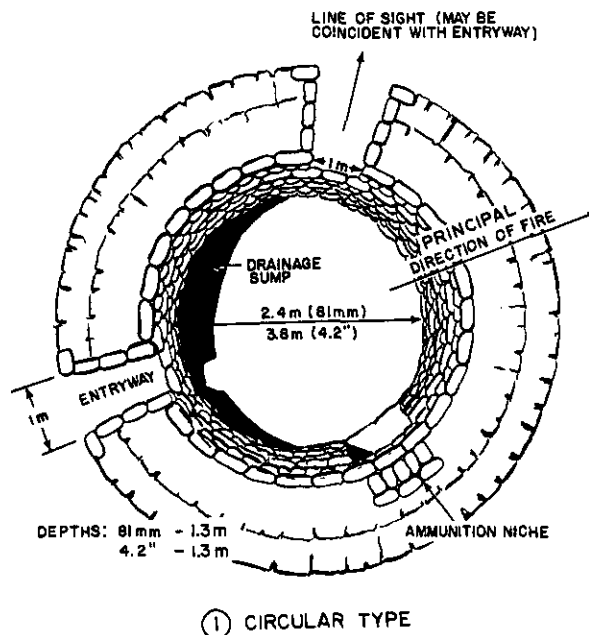
Figure 2-22. Mortar emplacements.
