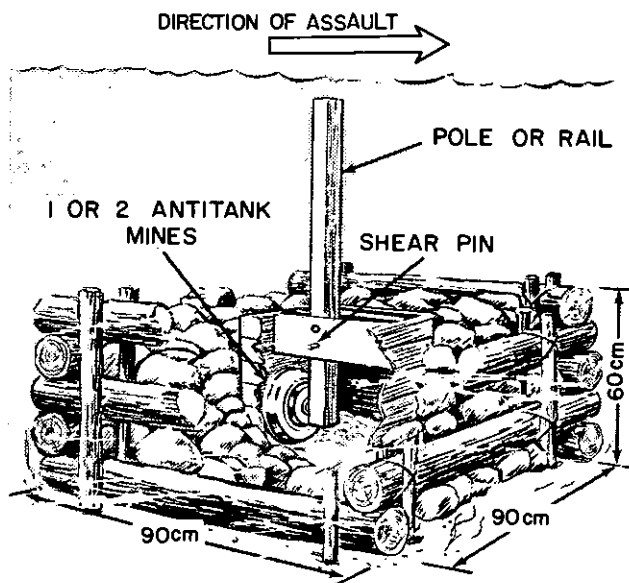
Figure 8-8. Nutcracker.
