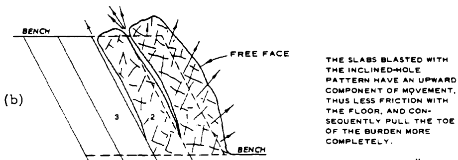
Fig. 5-7. Bench-slab movement during blast with vertical (a) and inclined (b) holes (after Langefors and Kihlström 14 )
