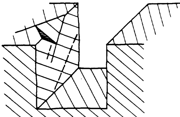
Fig. 6-4: Adverse dip of joints into excavation (left side)
