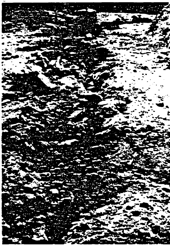
Fig. 5-18. Presplit fracture
