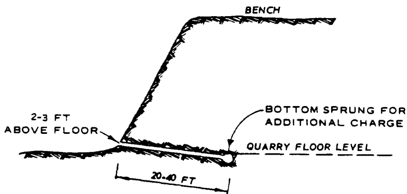
Fig. 5-8. Typical placement of snake hole
