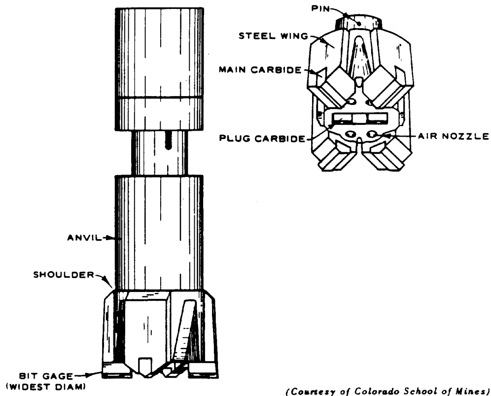
Fig. 4-14. Rotary-percussive drill bit (after Liljestr nd 13 )
