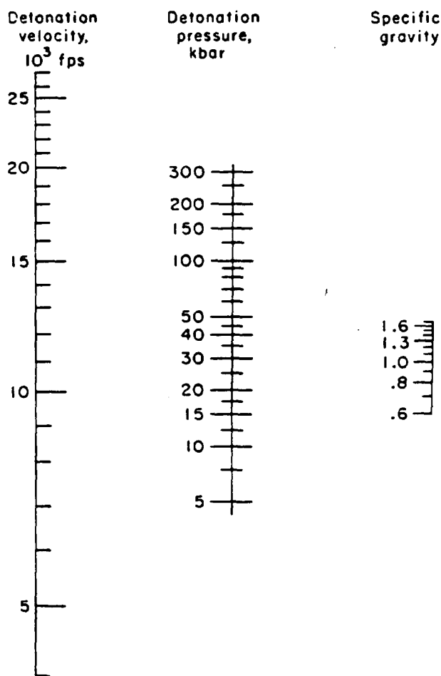
Fig. 3-4. Nomograph for finding detonation pressure 6
