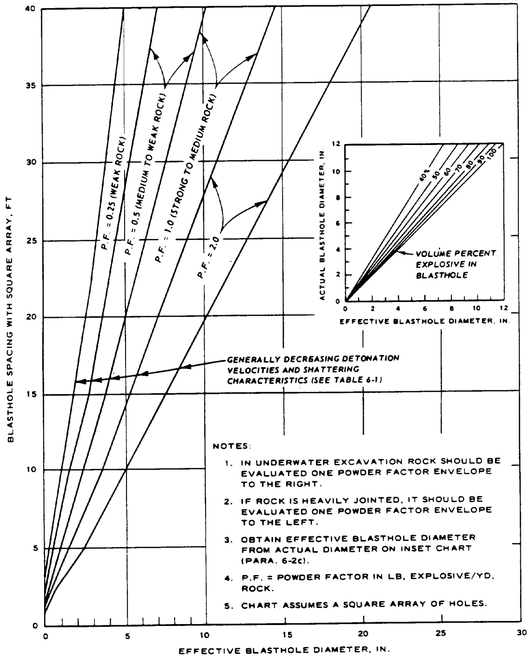
Fig. 6-2. Empirical relation: blasthole spacing and diameter and powder factor for multiple-row blast pattern in rocks of different strengths
