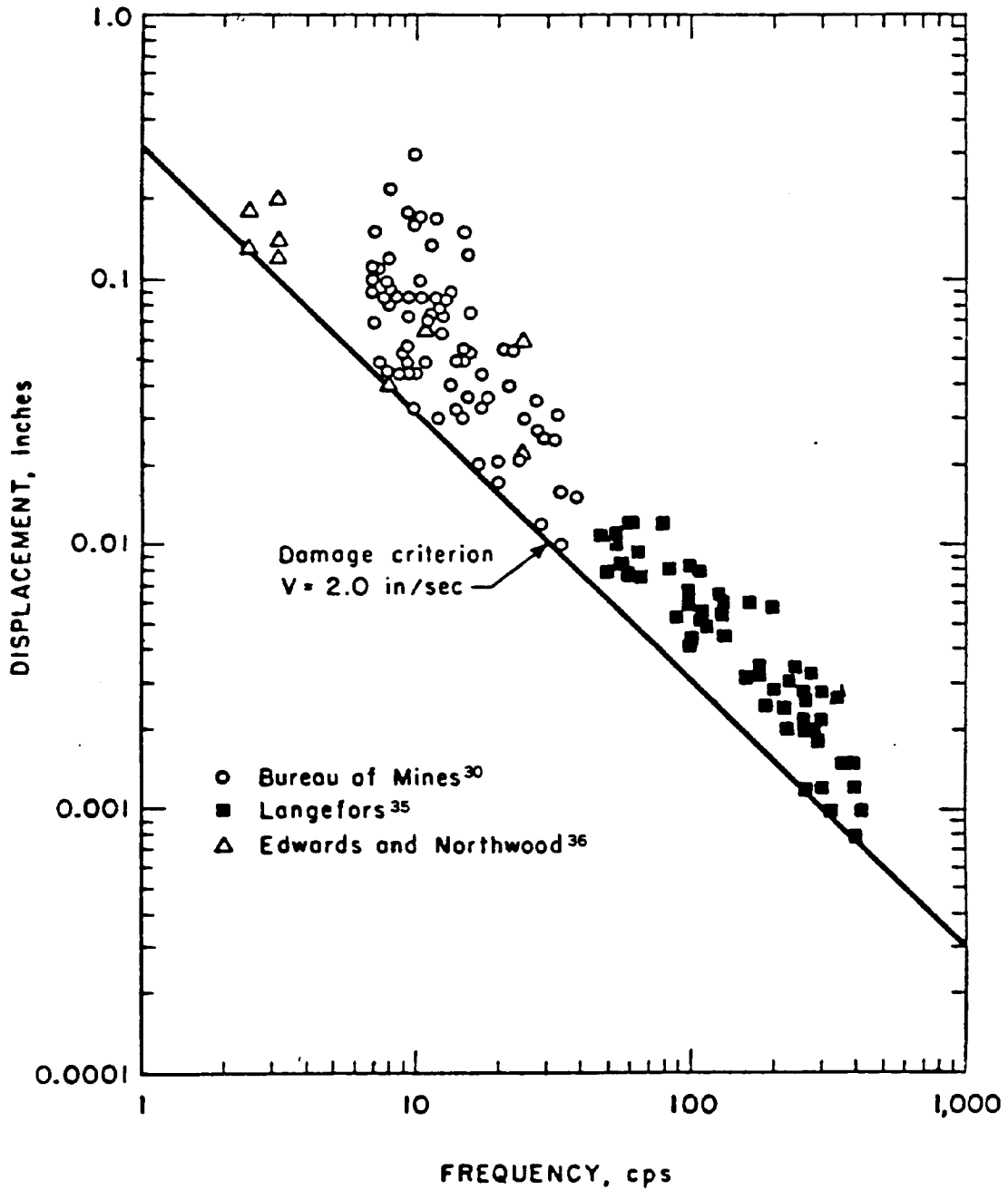
Fig. 7-3. Summary of nondamaging data above recommended safe vibration level for frame structures (modified from ref 37)
