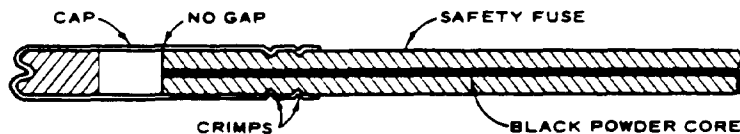
b. FUSE PROPERLY INSERTED IN CAP (SECTION)
