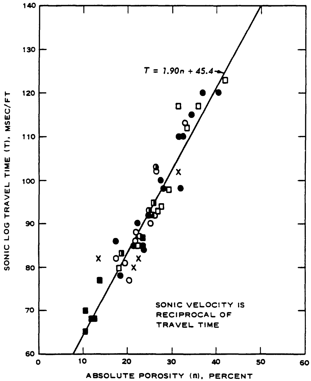
Fig. 6-3. Sonic log travel time as a function of porosity for a suite of volcanic sedimentary rocks and lava (after Carroll 26 )
