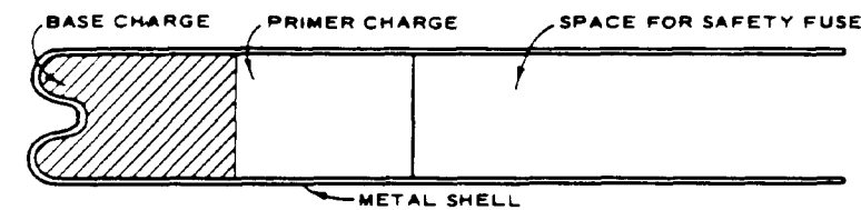
a. CAP (SECTION)
