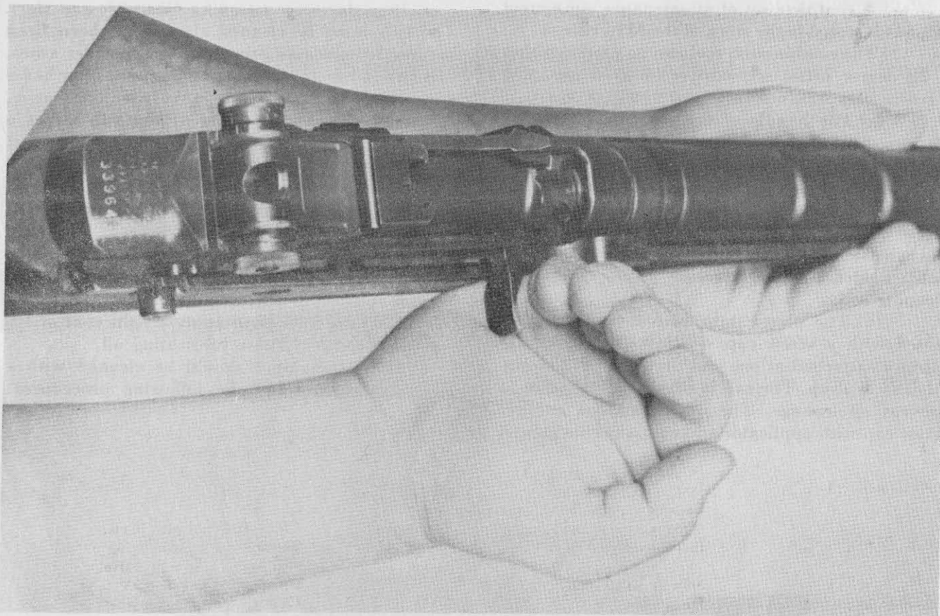
Figure 39. Applying immediate action.
