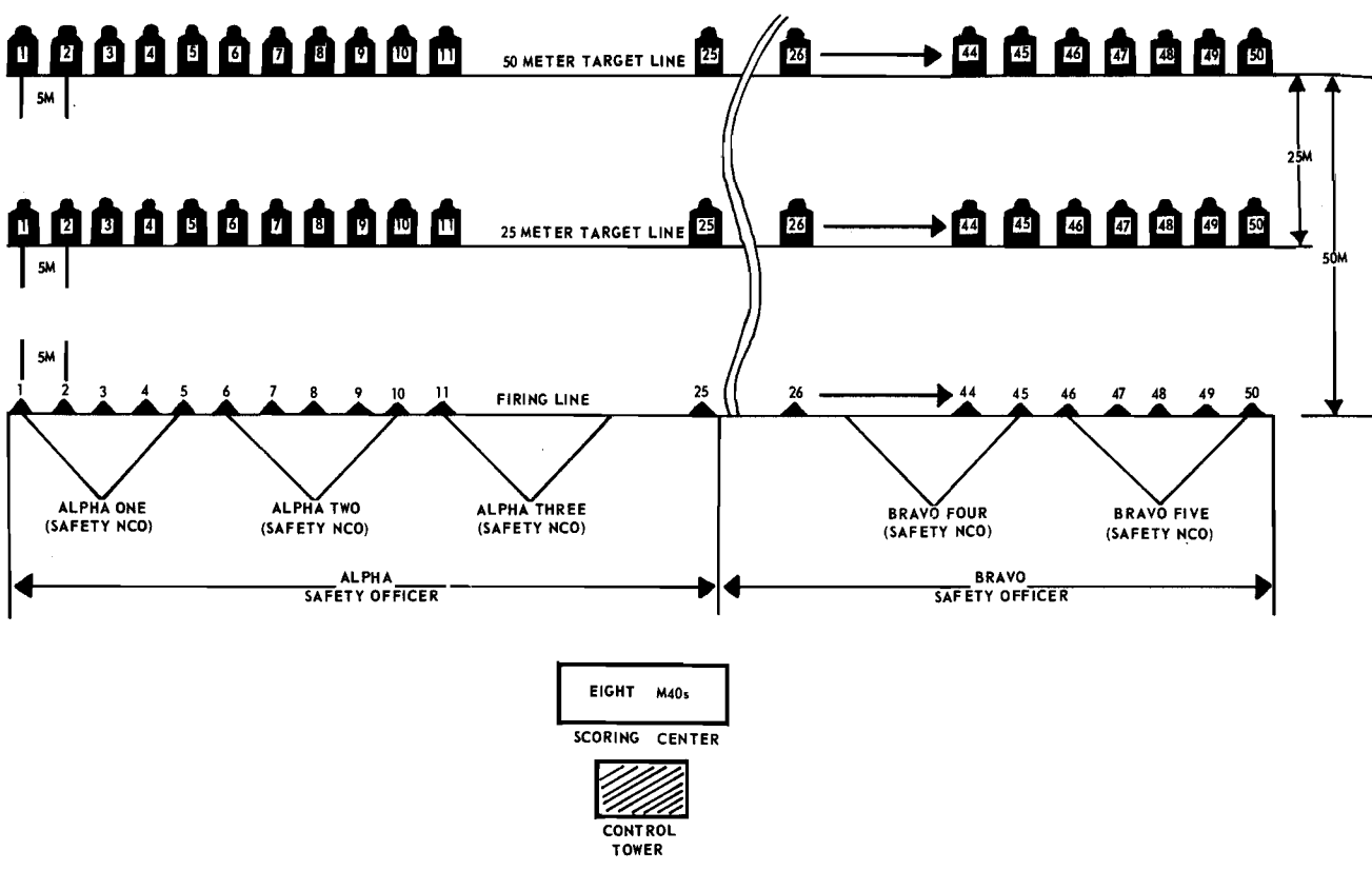
Figure 121. Night firing range (no troop movement required).
