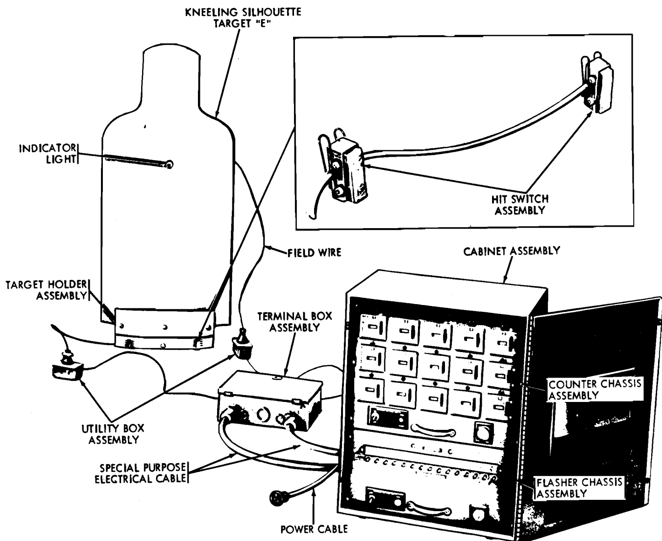
Figure 126. Night firing target mechanism M40—components and assemblies.
