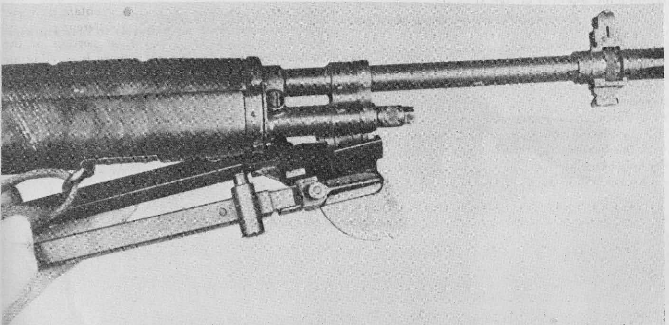
Figure 51. Installation of M2 bipod.
