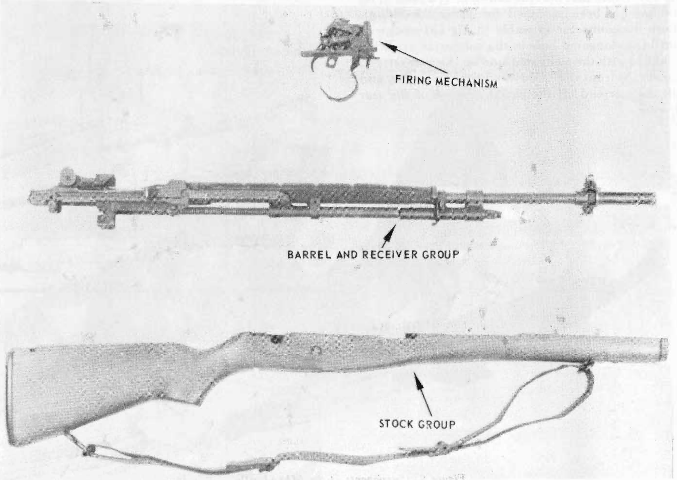
Figure 7. Components of the M14 rifle.
