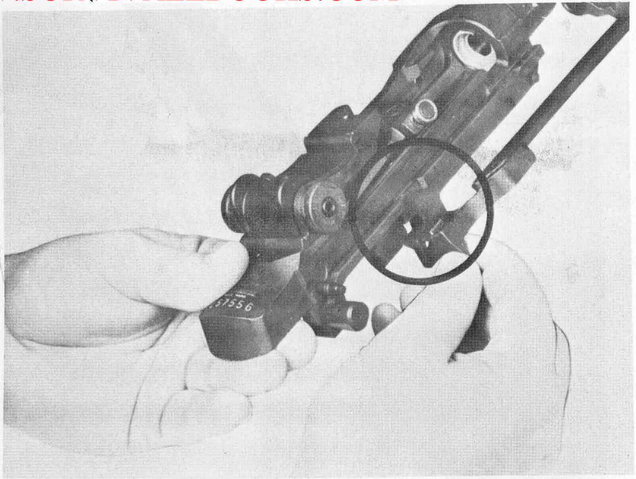
Figure 12. Removing operating rod.
