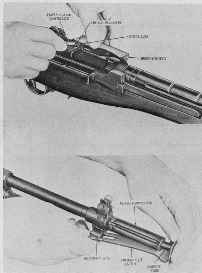
Figure 58. Installation of blank firing attachment and breech shield.
