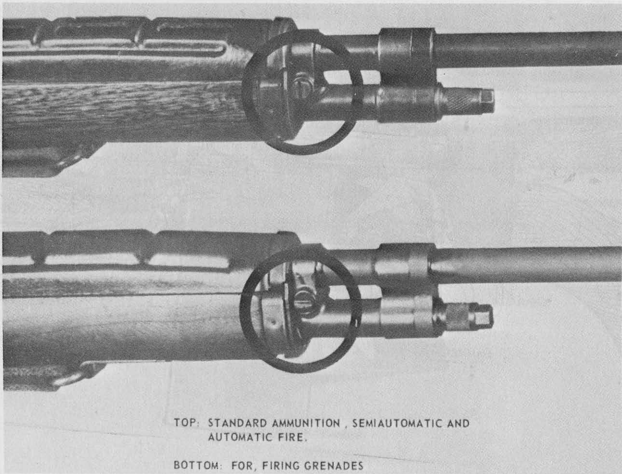
Figure 32. Positions of the spindle valve.
