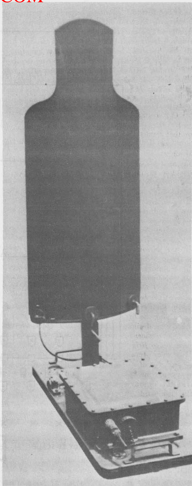
Figure 84. Automatic target device (M31A1) with E-type silhouette.
