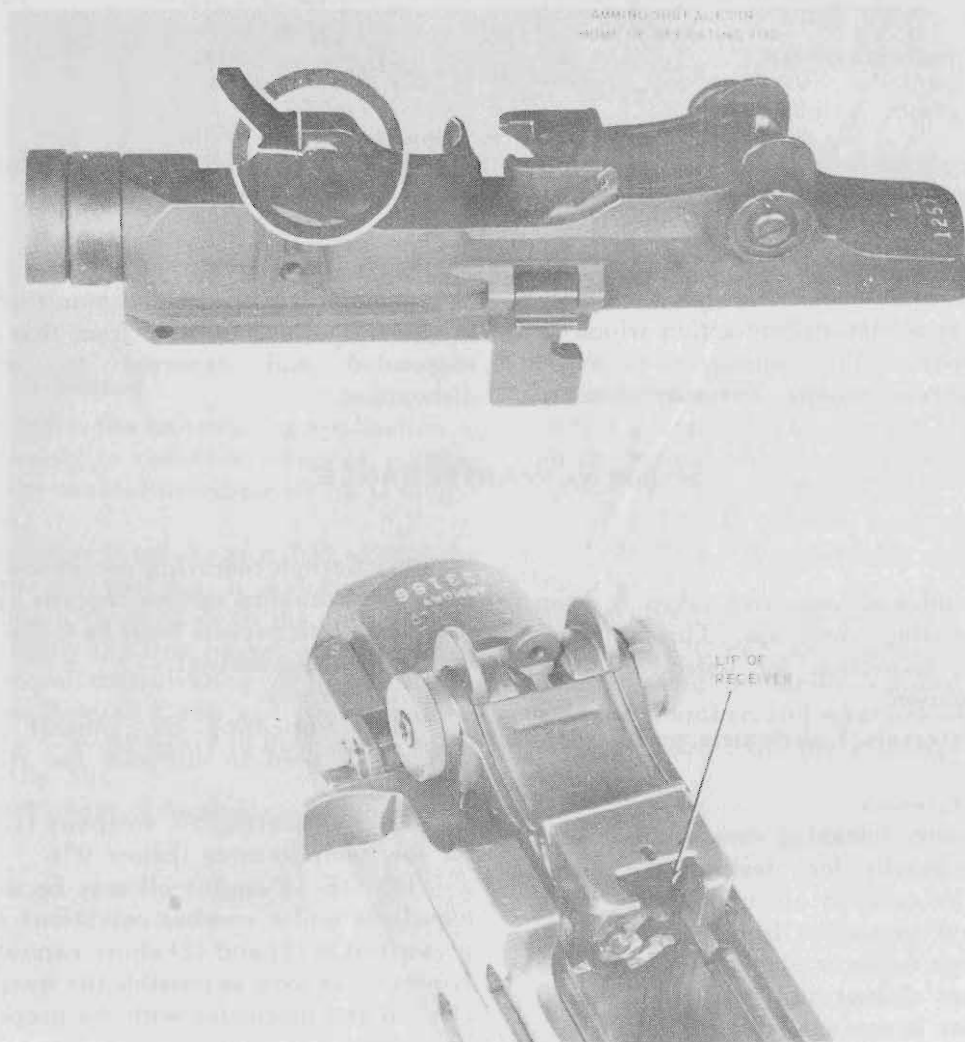
Figure 40. Points to apply rifle grease.
