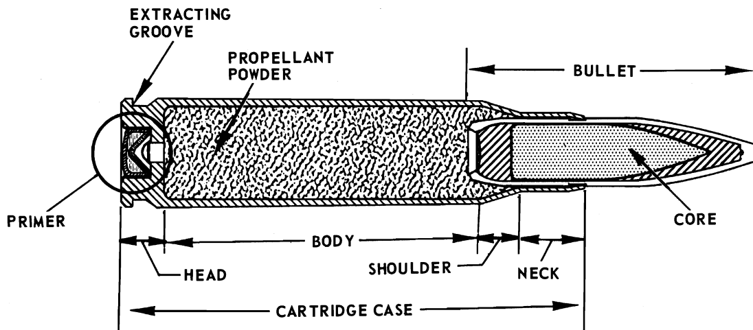
Figure 48. Parts of a cartridge.
