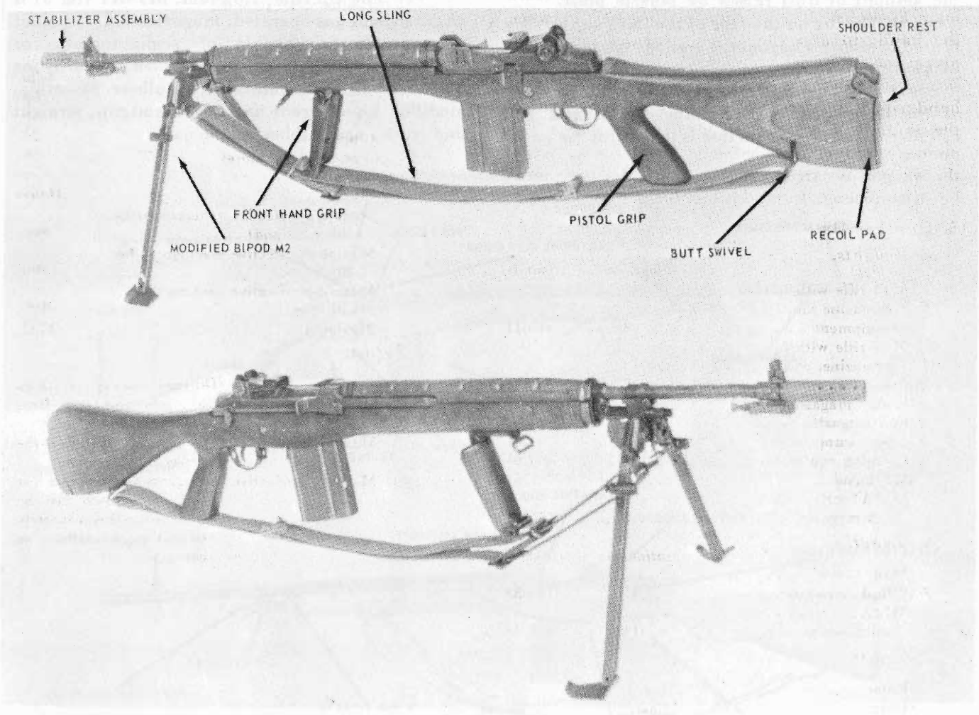
Figure 3. M14A1 rifle.
