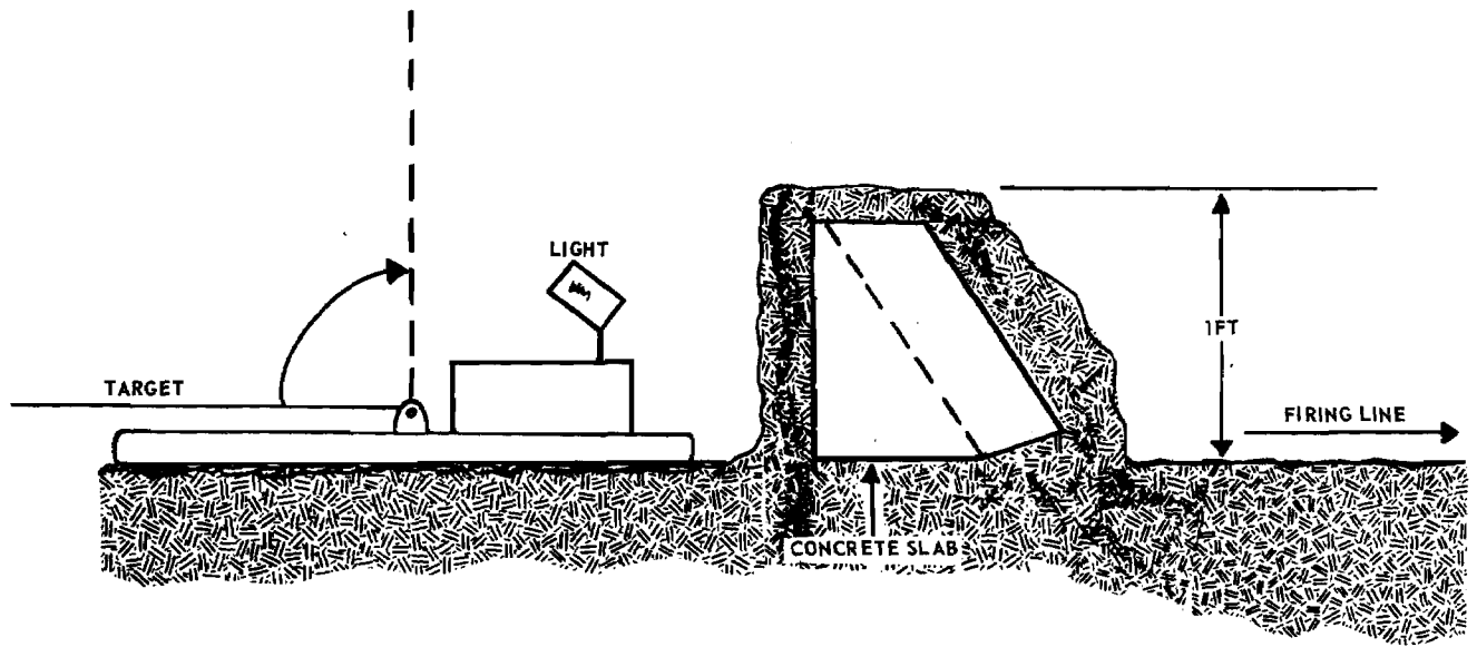
Figure 124. M31A1 target holding mechanism with berm.
