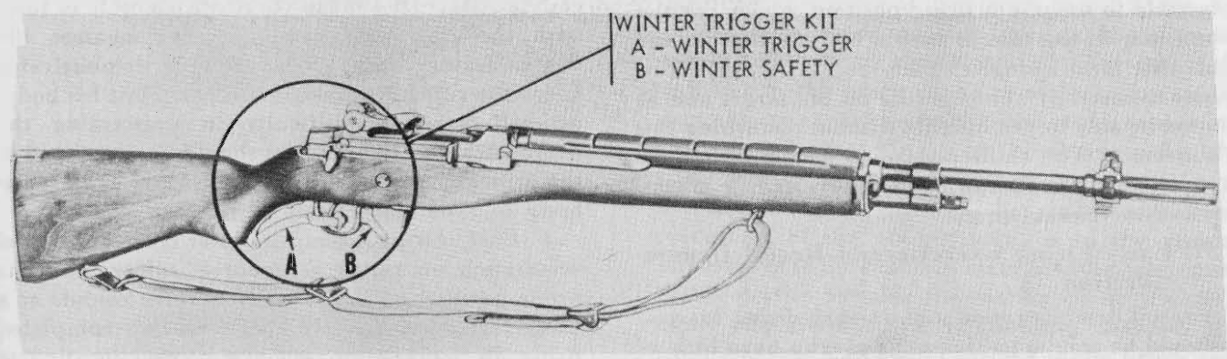
Figure 60. M14 rifle with winter trigger kit installed.
