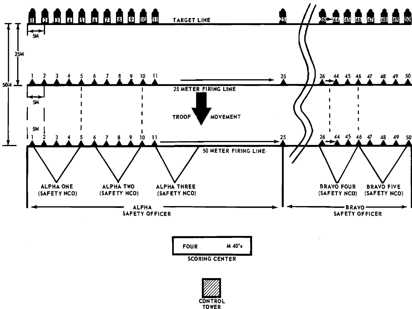
Figure 120. Night fire range (troop movement to rear).
