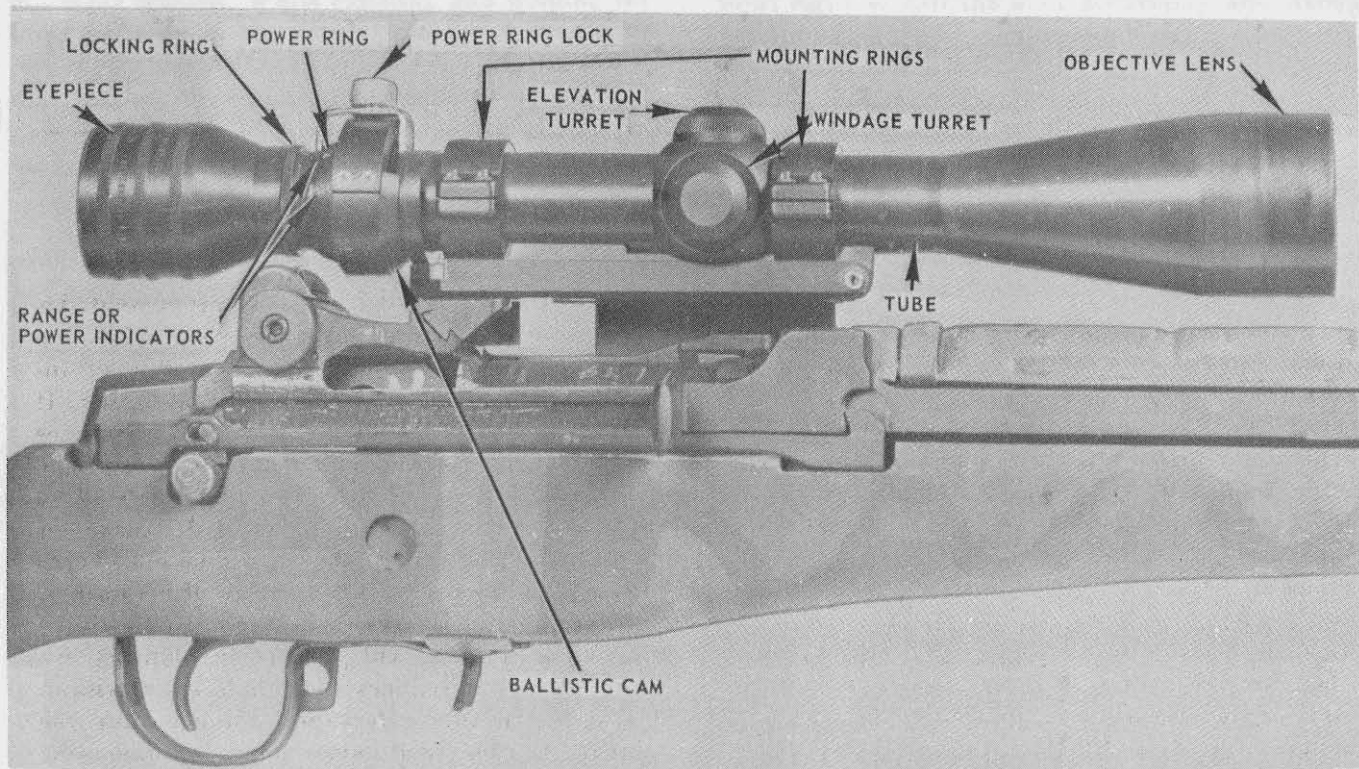
Figure 131. Sniperscope with mount.
