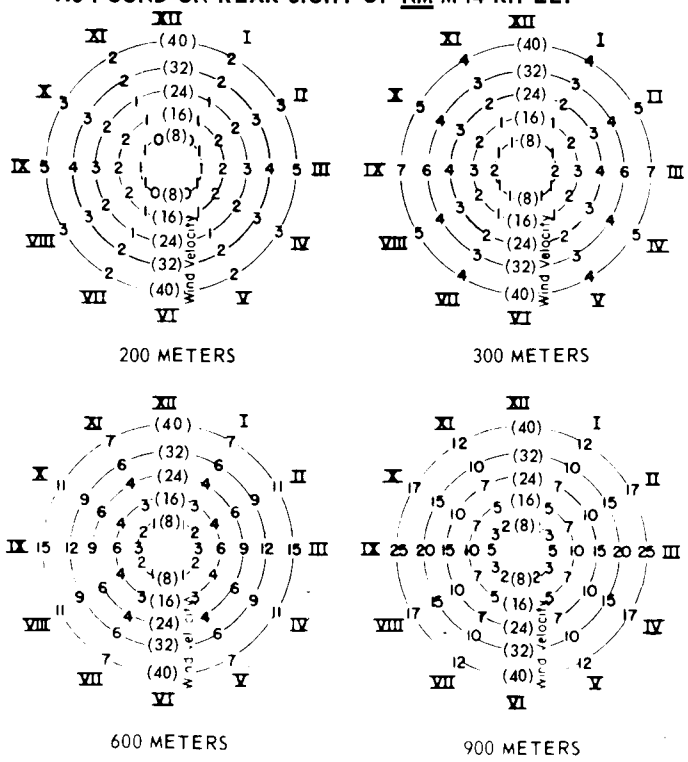
Figure 148. National match M14 windage diagram.
