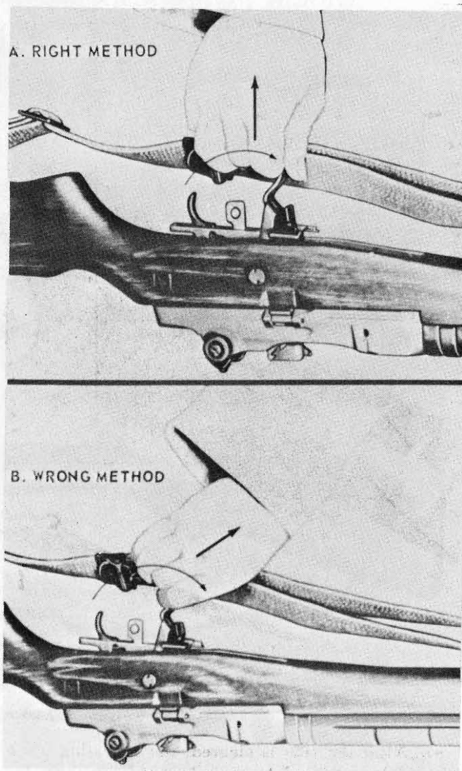
Figure 6. Removing the firing mechanism.
