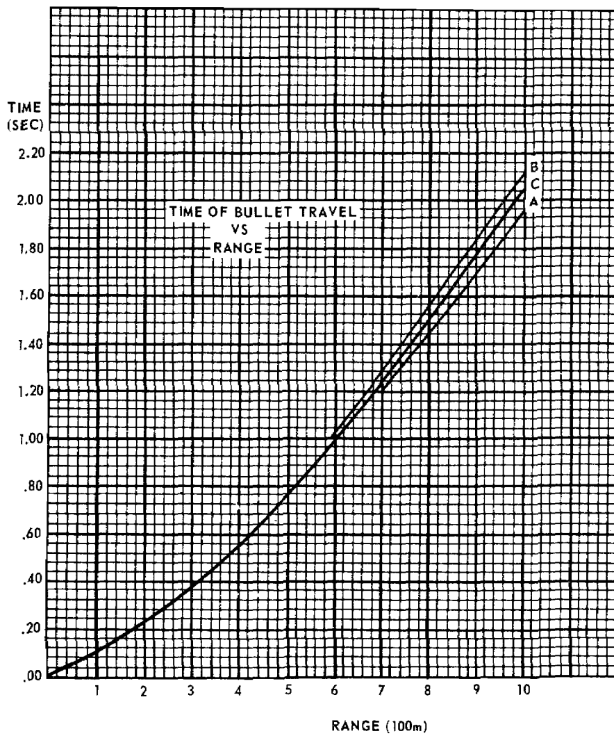
Figure 152. Chart 4. time of bullet travel versus range.
