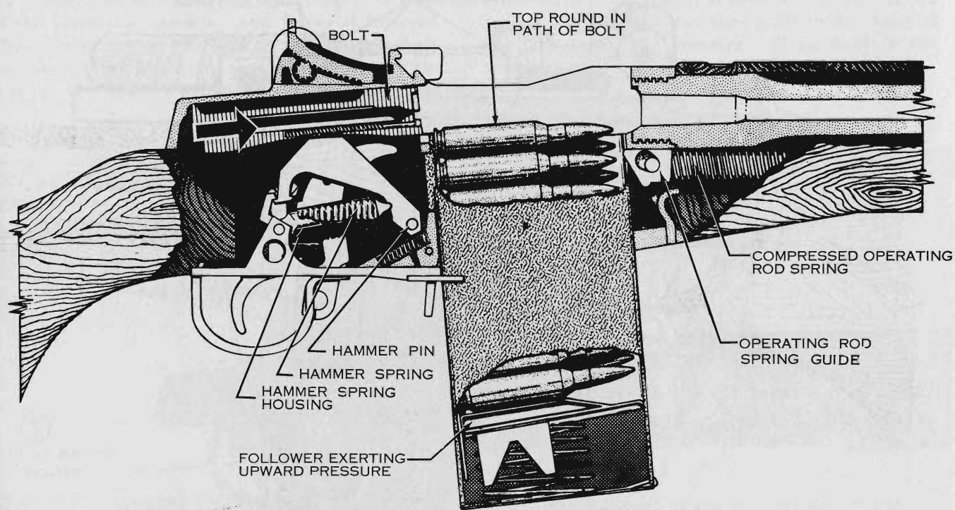
Figure 35. Feeding.
