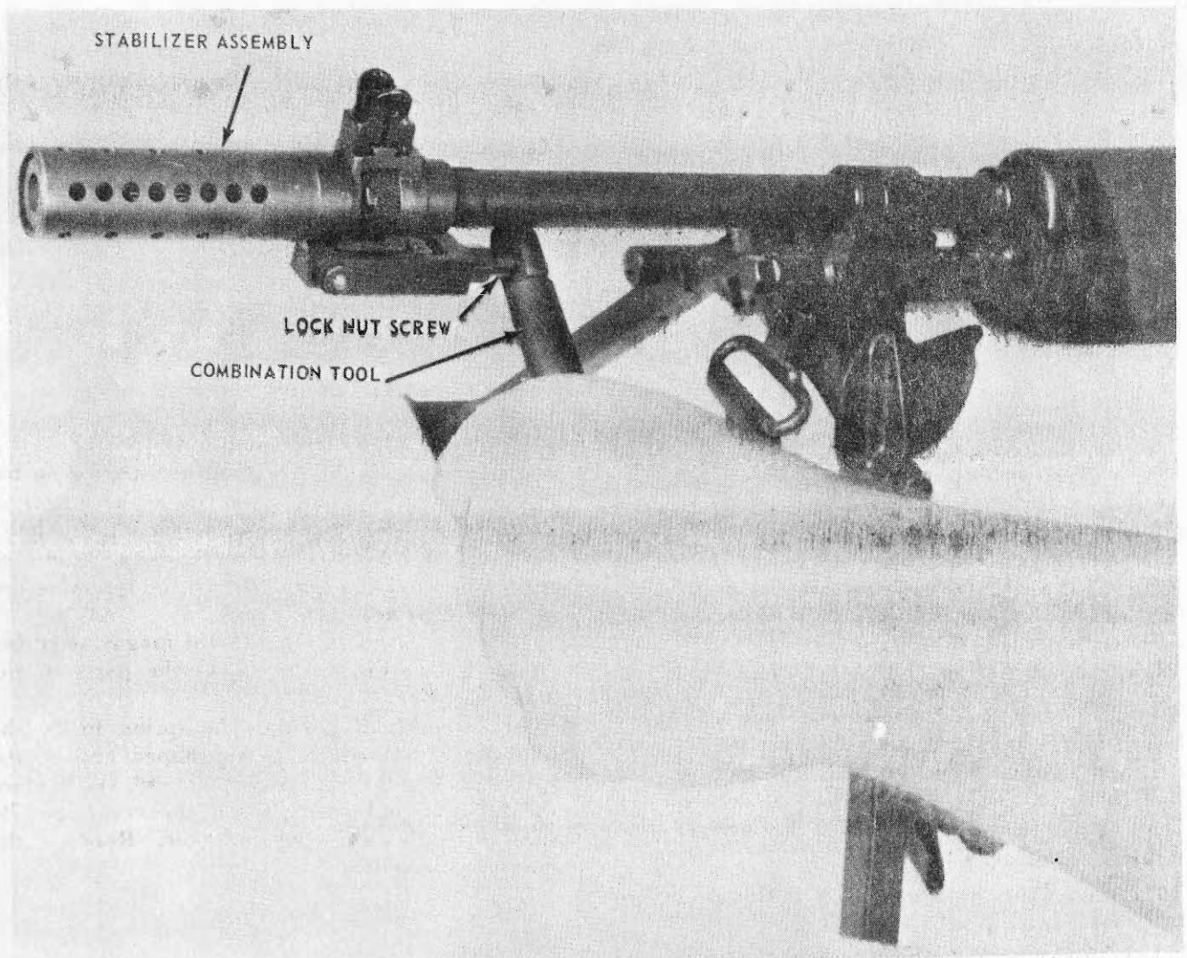
Figure 20. Removing the stabilizer assembly.
