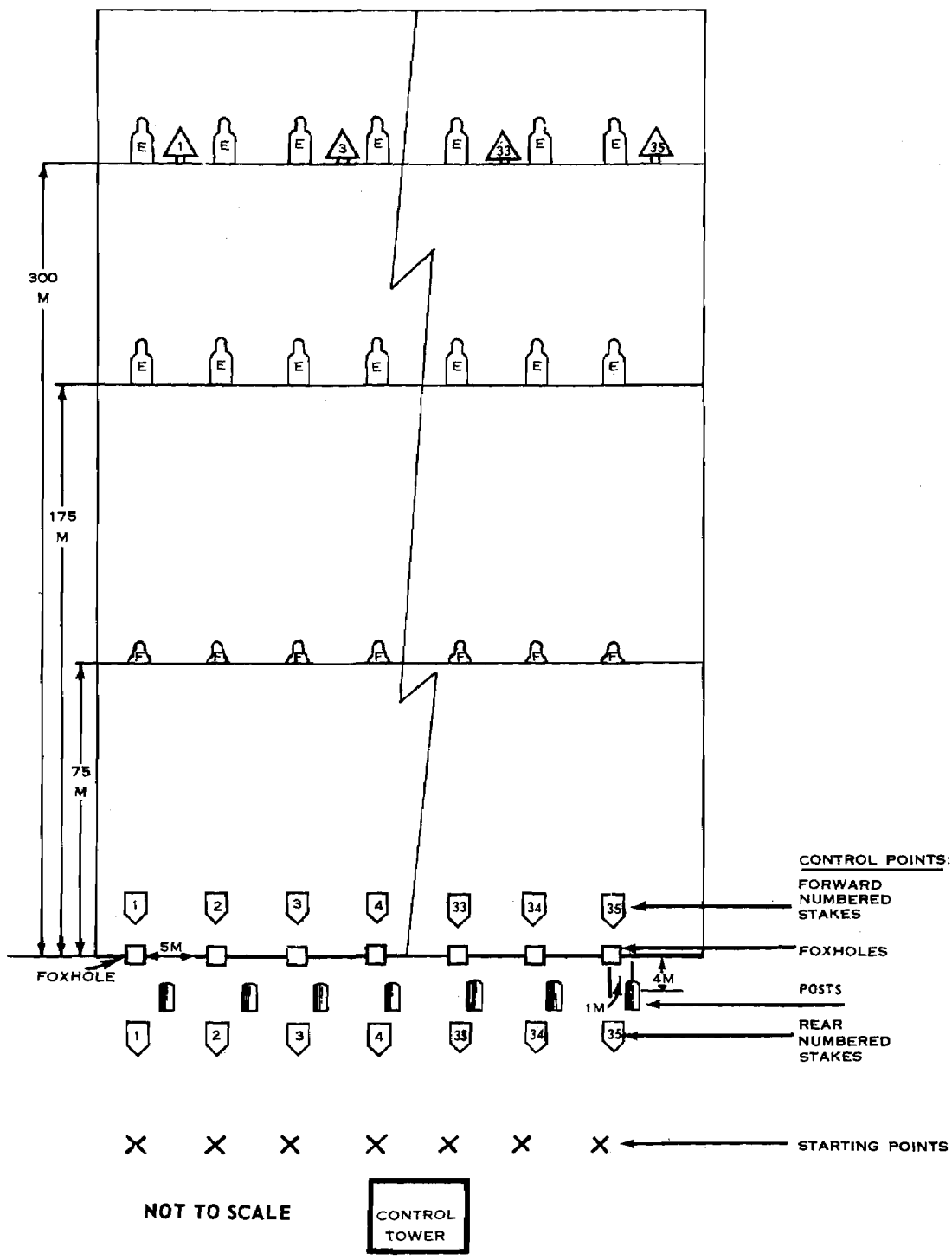
Figure 83. Standard rifle marksmanship field firing range.
