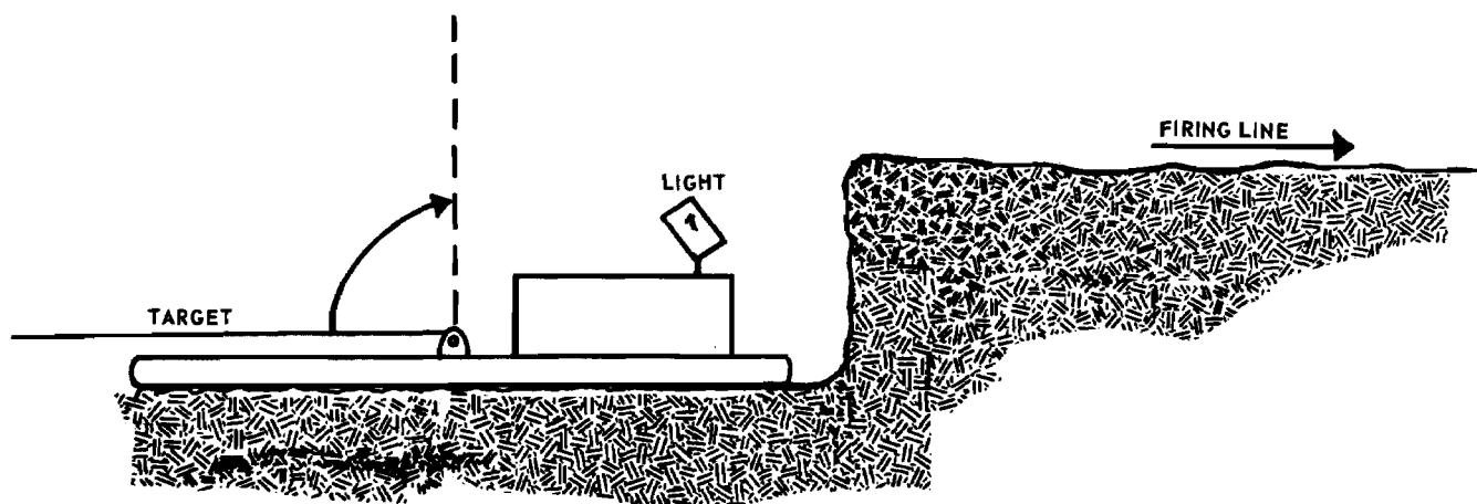
Figure 123. Countersunk M31A1 target holding mechanism.
