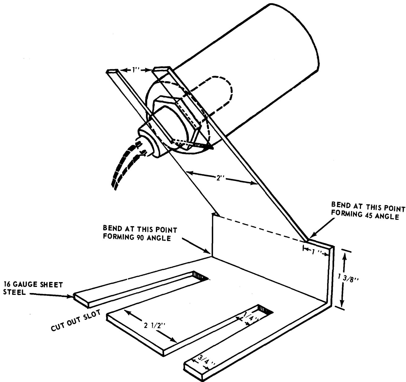
Figure 130. Indicator light bracket (locally fabricated).
