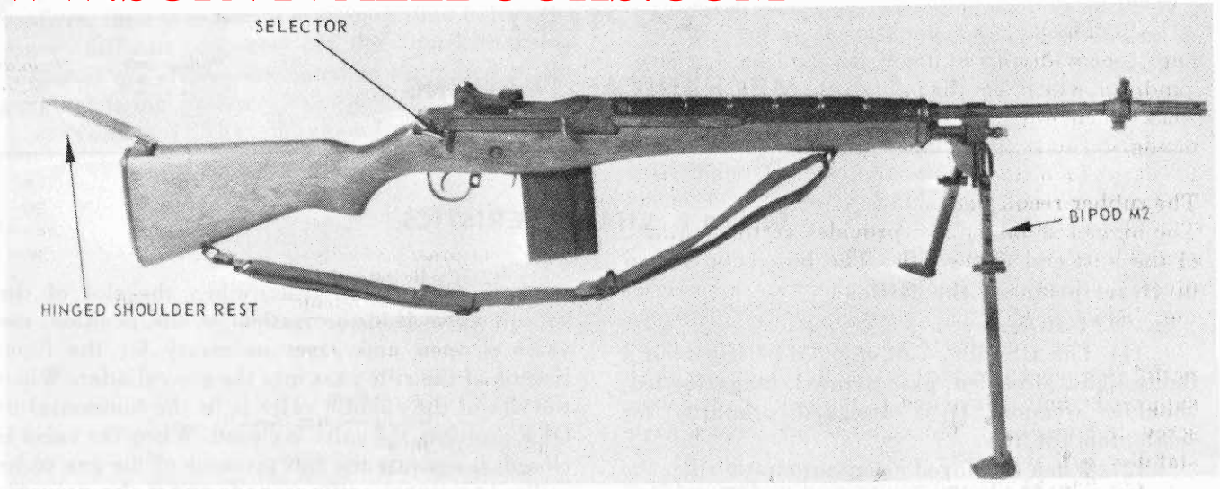
Figure 2. M14 rifle with selector and M2 bipod.
