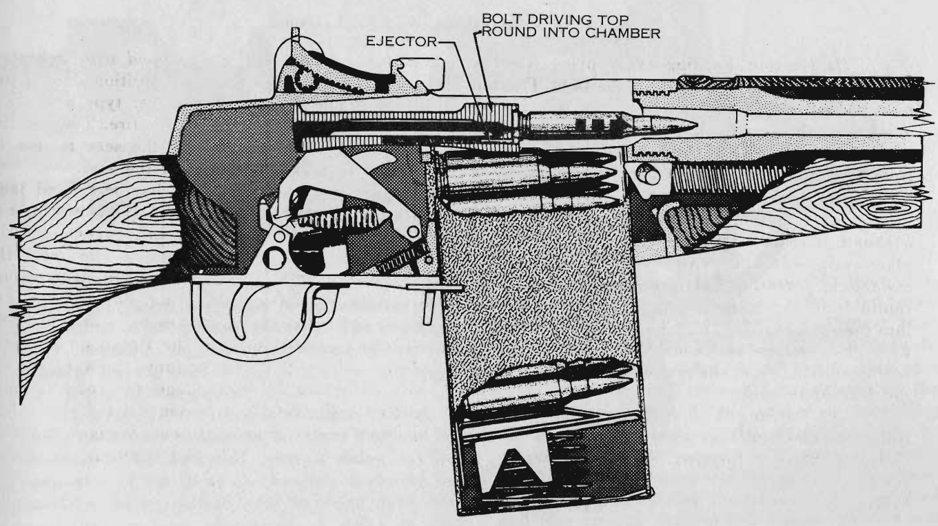
Figure 36. Chambering.
