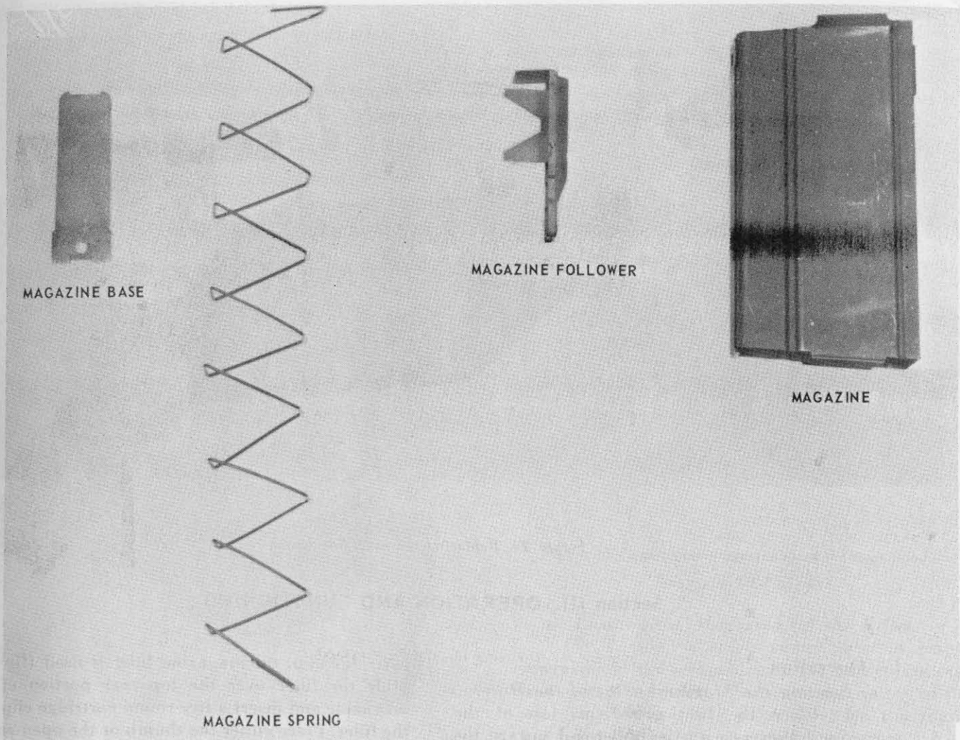
Figure 23. Parts of the magazine.
