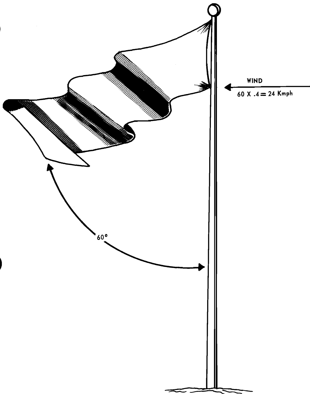
Figure 145. The flag method of wind estimation.
