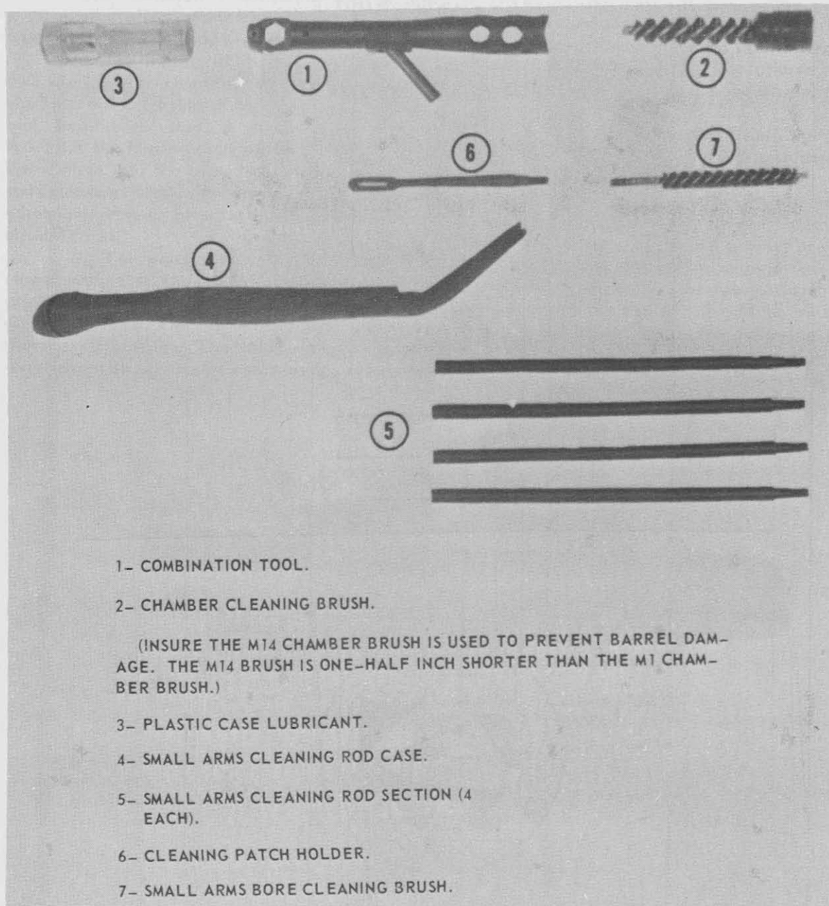
1 Figure 41. Maintenance equipment.
