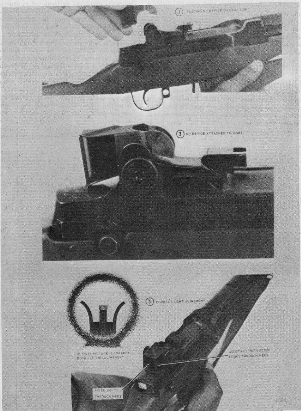
Figure 77. M2 aiming device.
