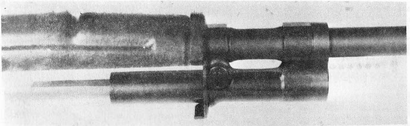
Figure 19. Gas piston properly seated.
