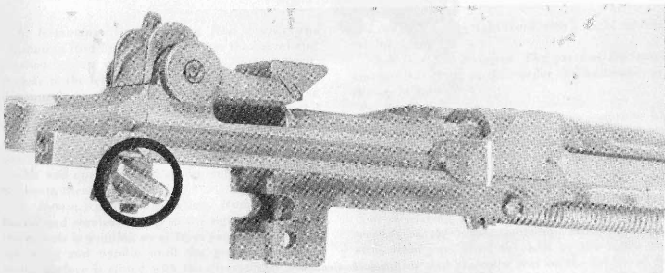
Figure 9. Position of the selector for removing the connector assembly (rifle modified for selective firing).
