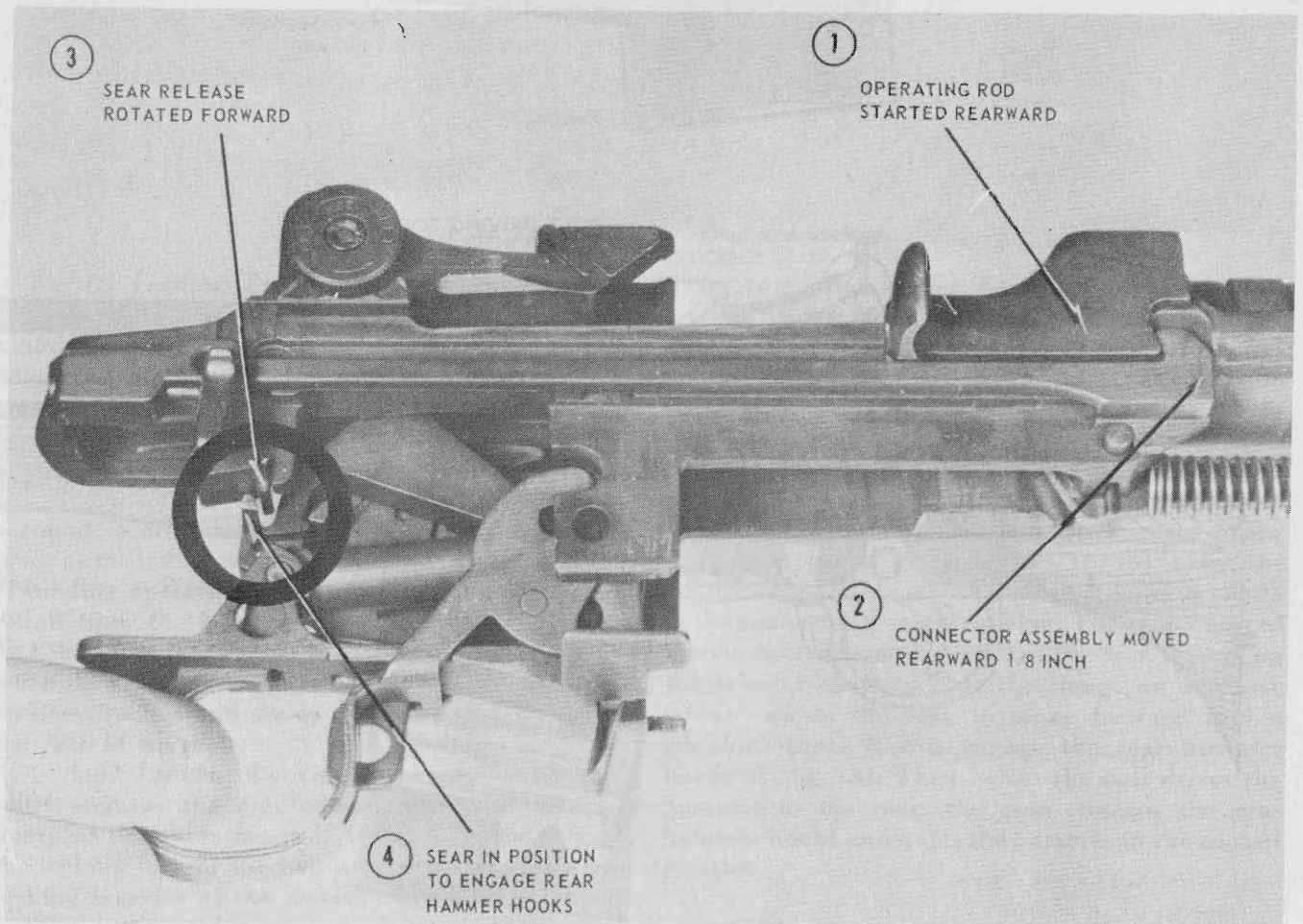
1 Figure 38. Actions of the connector assembly and its effects on the firing mechanism during automatic firing.
