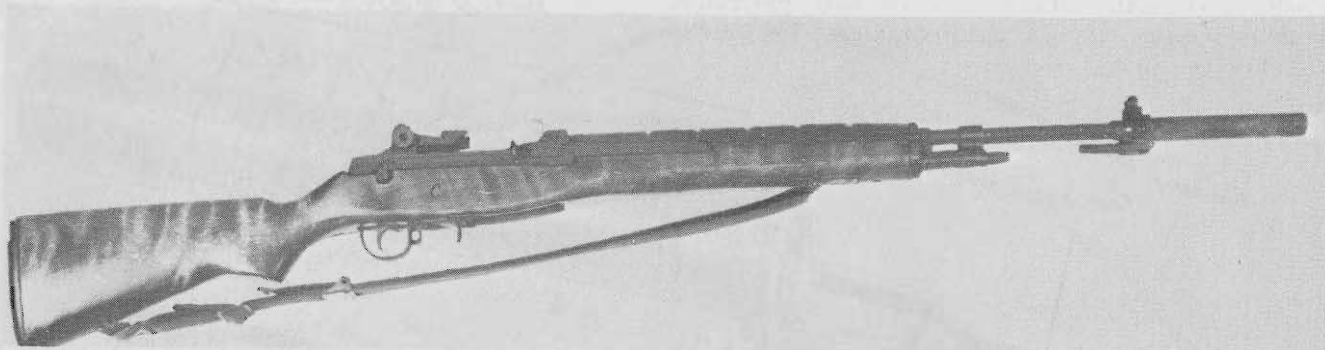
Figure 55. M14 rifle with M76 grenade launcher.
