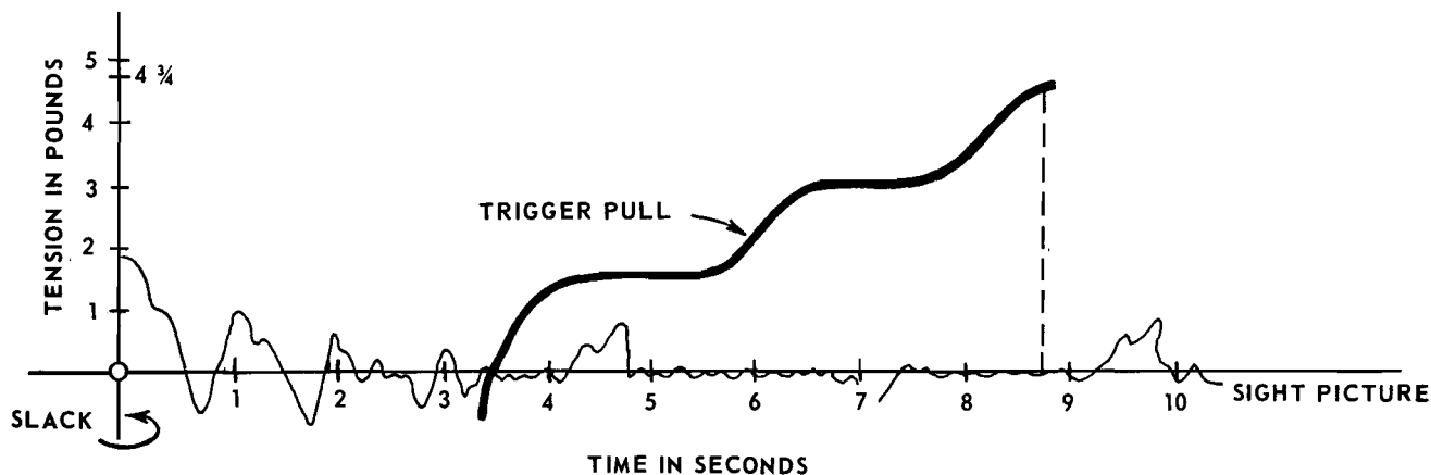
Figure 143. Interrupted trigger pull.
