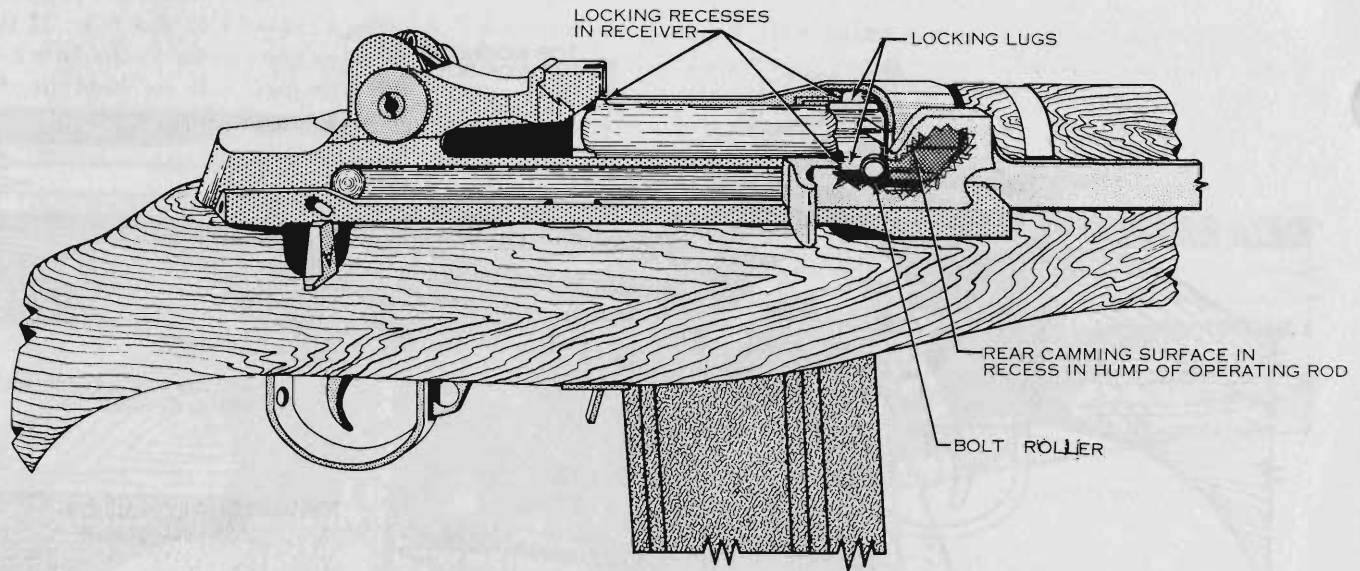
Figure 37. Locking.
