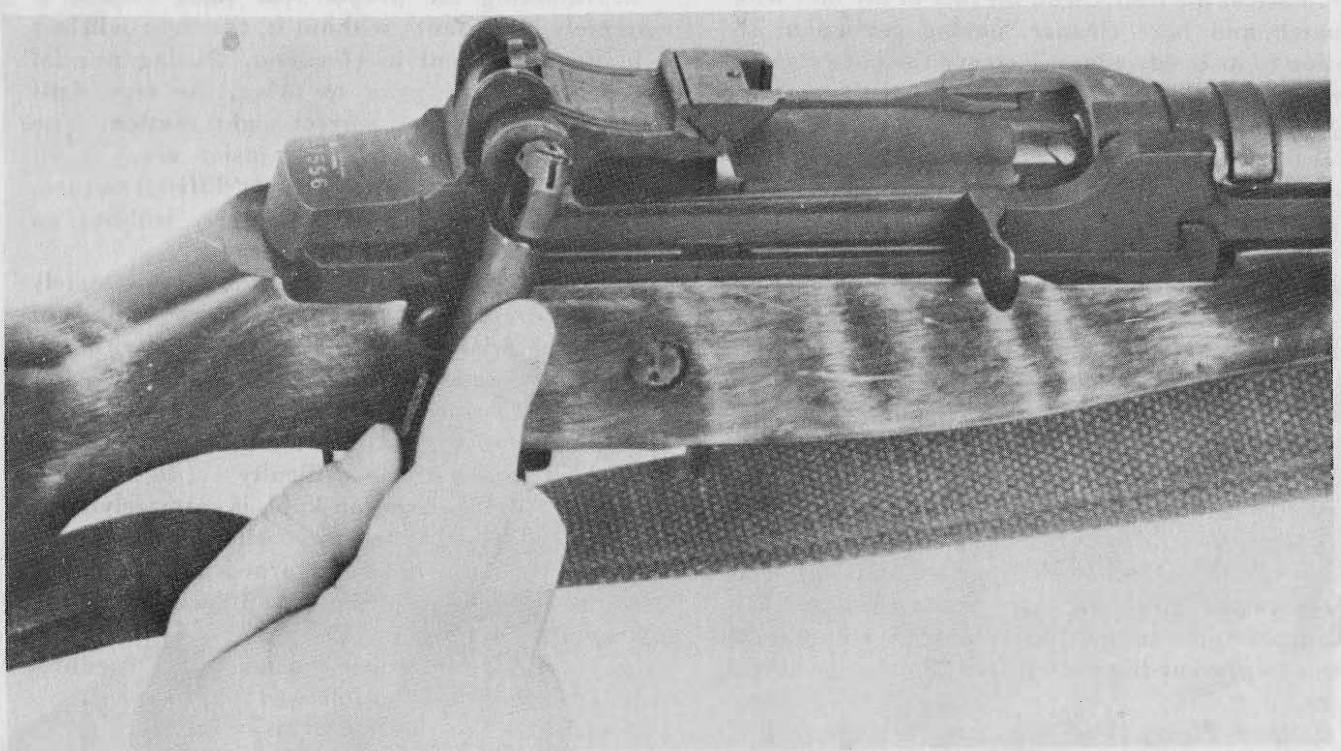
1 Figure 47. Adjusting sight tension.
