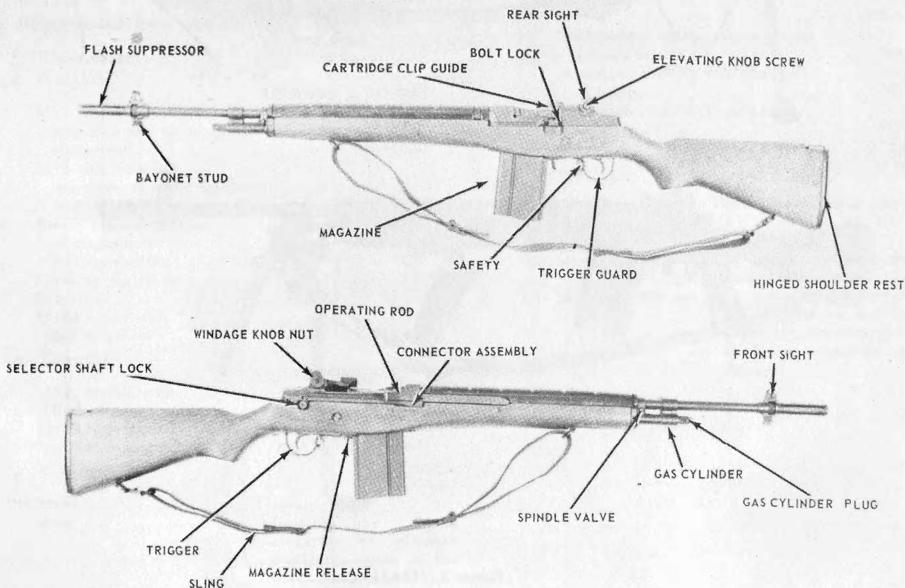
Figure 1. M14 rifle.
