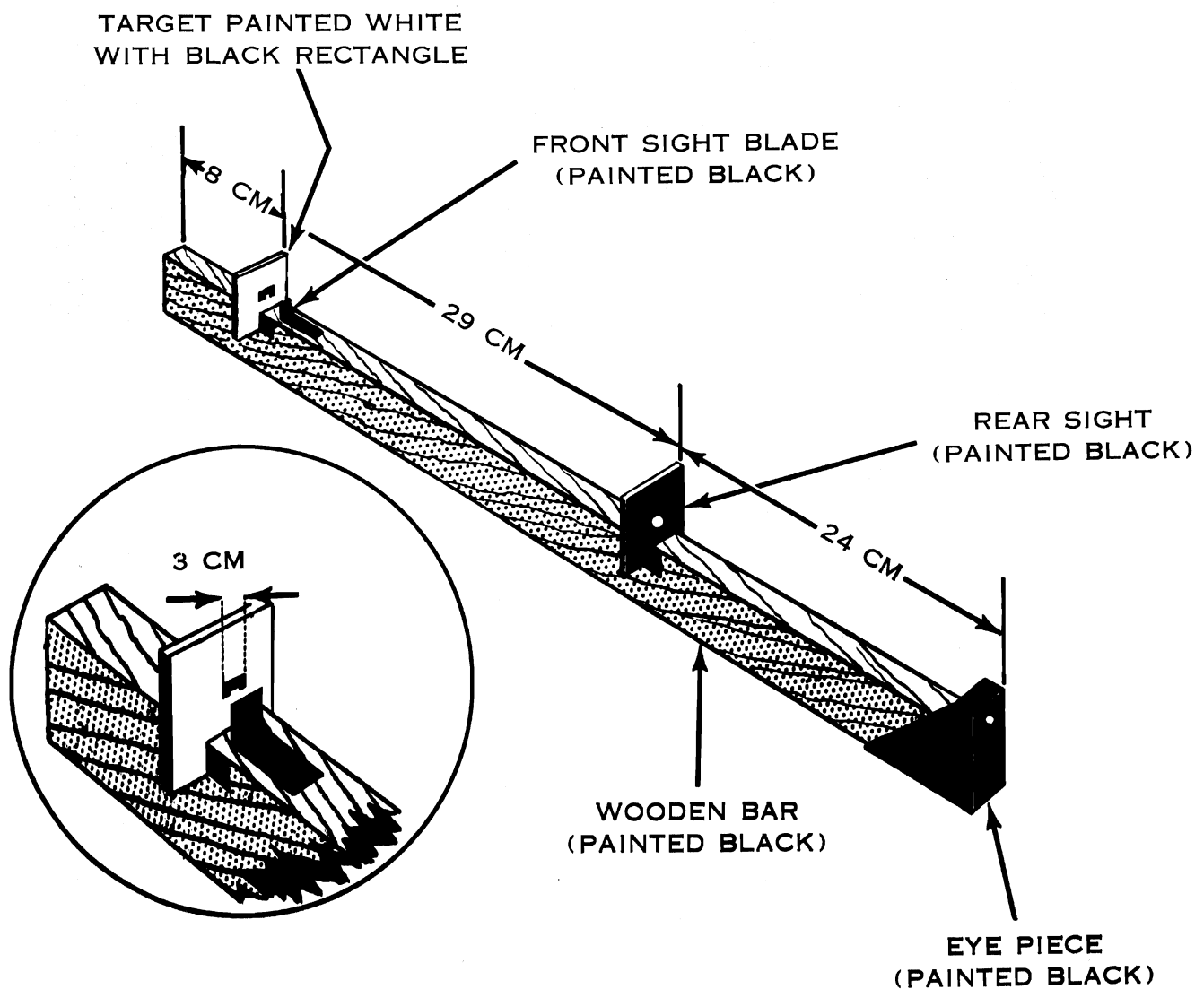
Figure 78. Aiming bar.
