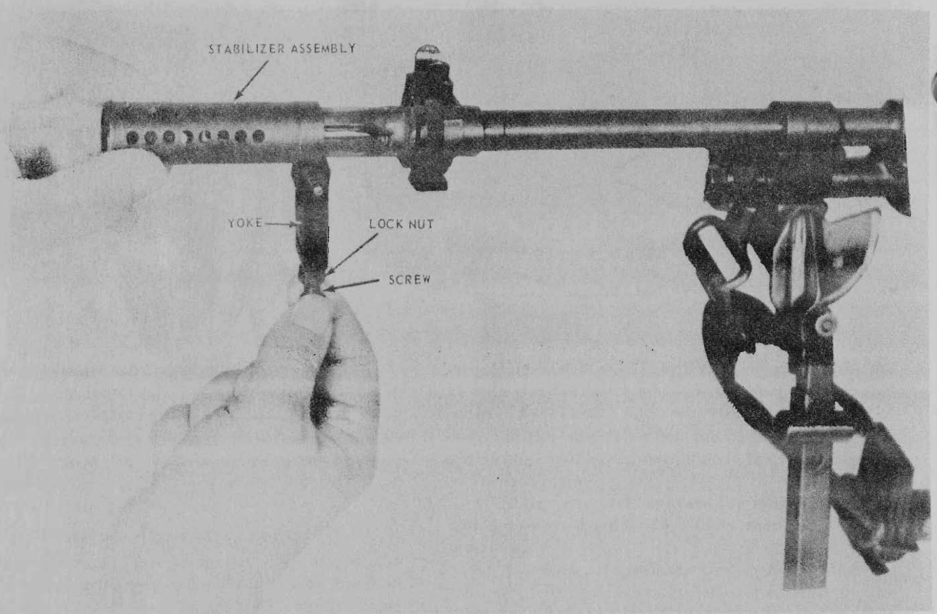
Figure 21. Replacing the stabilizer assembly.
