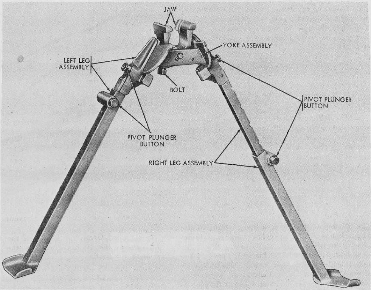
Figure 50. M2 bipod.
