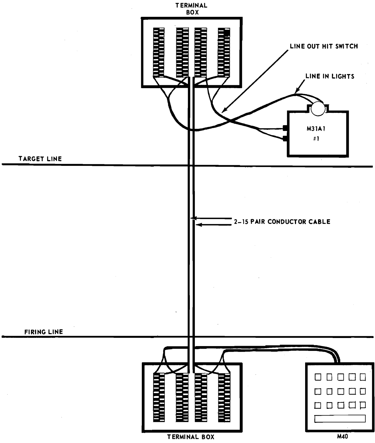
Figure 129. Wiring diagram—firing line to target line.
