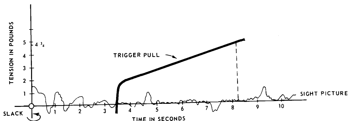
Figure 142. Smooth trigger pull.
