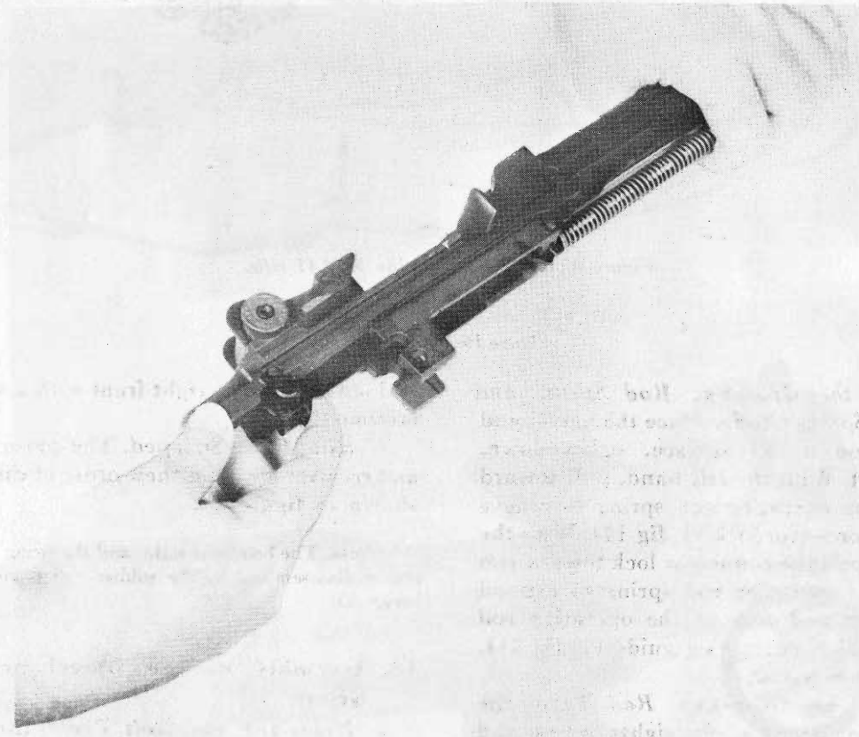
Figure 10. Removing the connector assembly.
