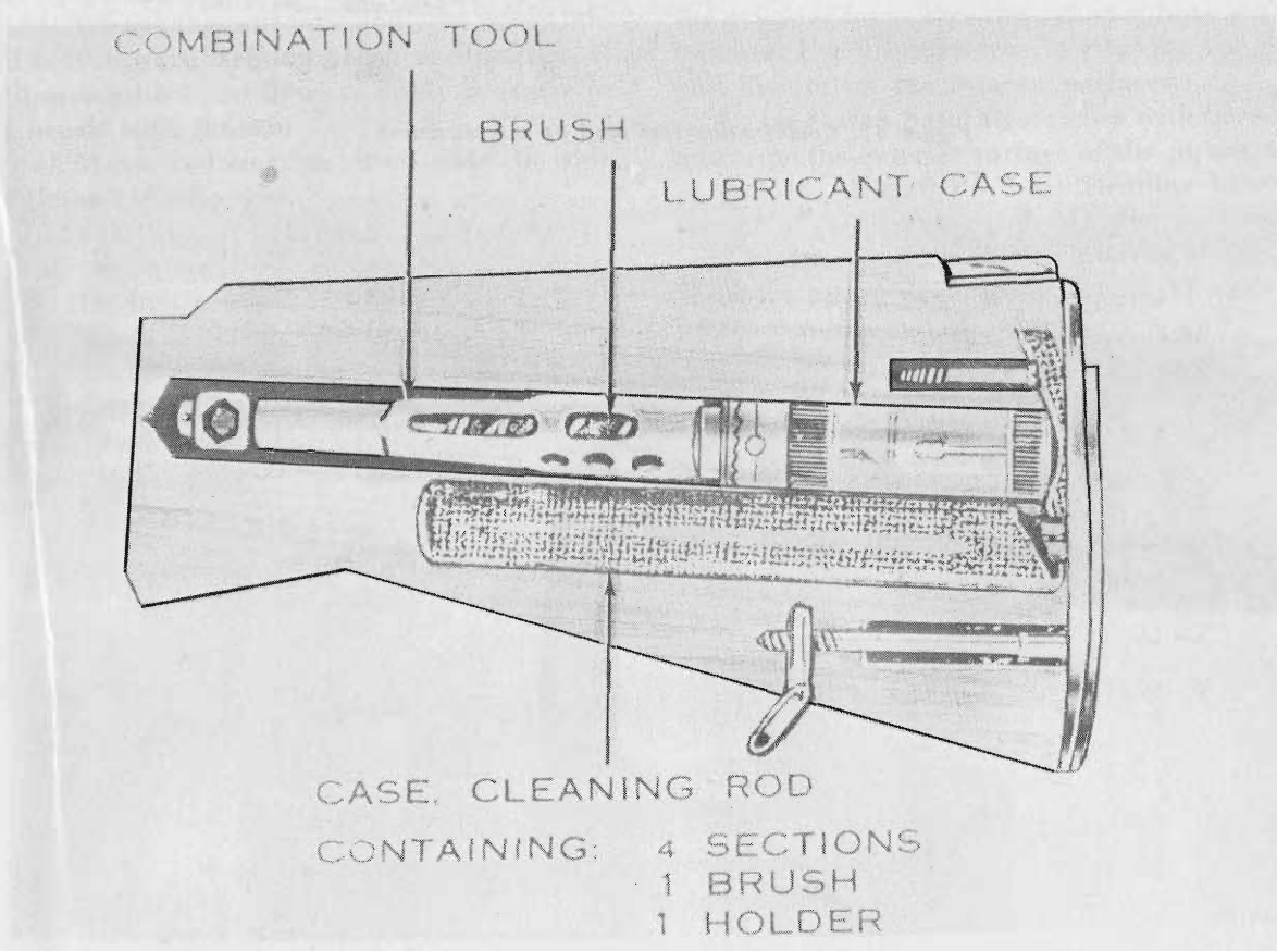
3 Figure 41—Continued.
