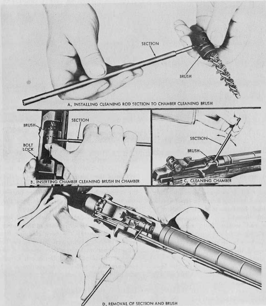
Figure 45. Cleaning the chamber.
