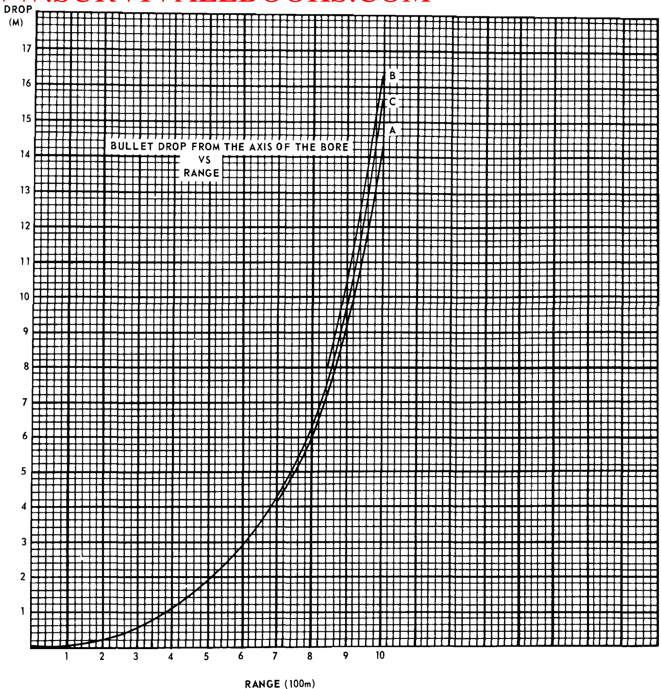
Figure 153. Chart 5. bullet drop versus range.
