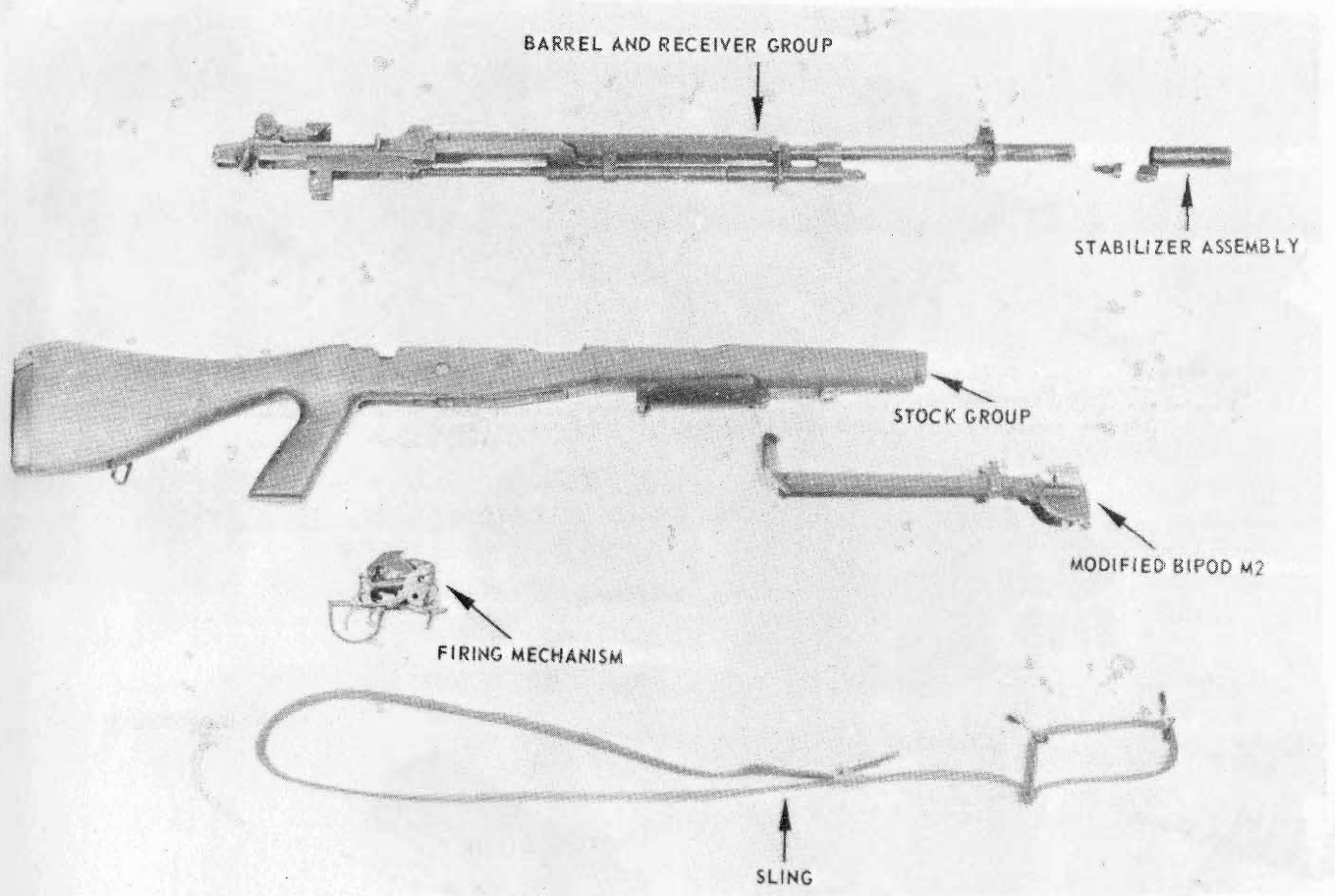
Figure 8. Components of the M14A1 rifle.
