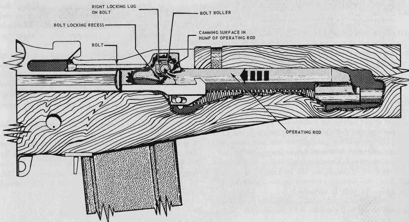
Figure 31. Unlocking.
