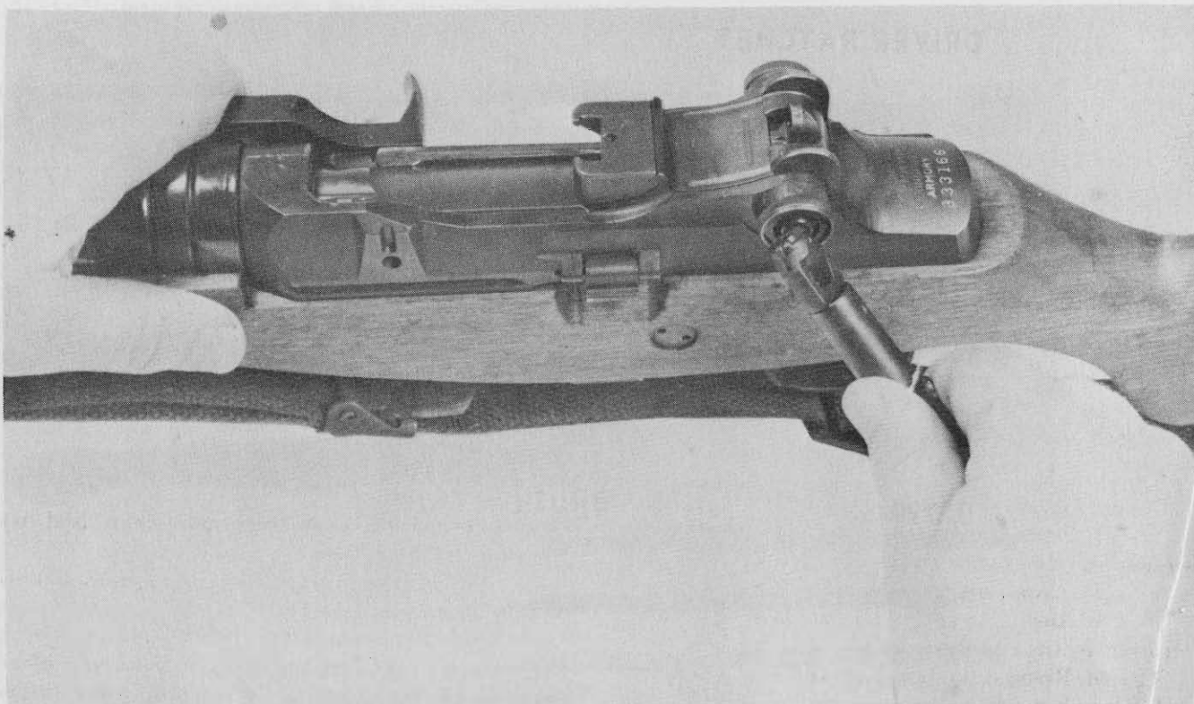
Figure 42. Combination tool used as a screwdriver.
