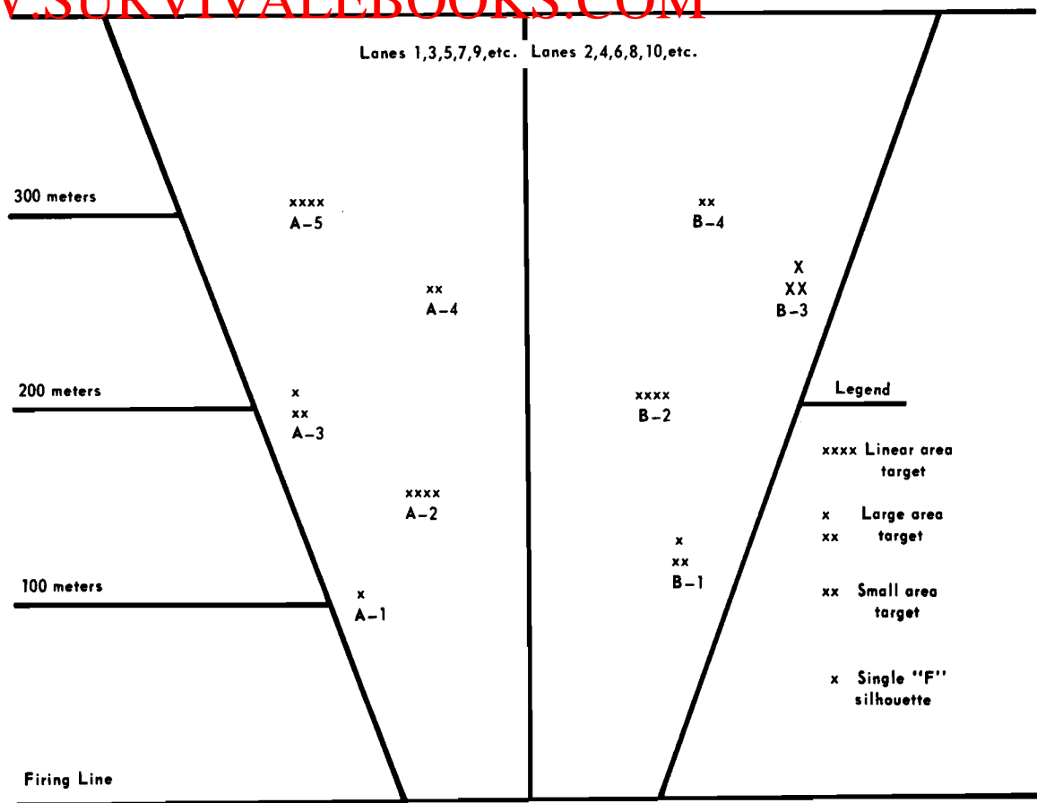
Figure 108. Standard automatic rifle range.
