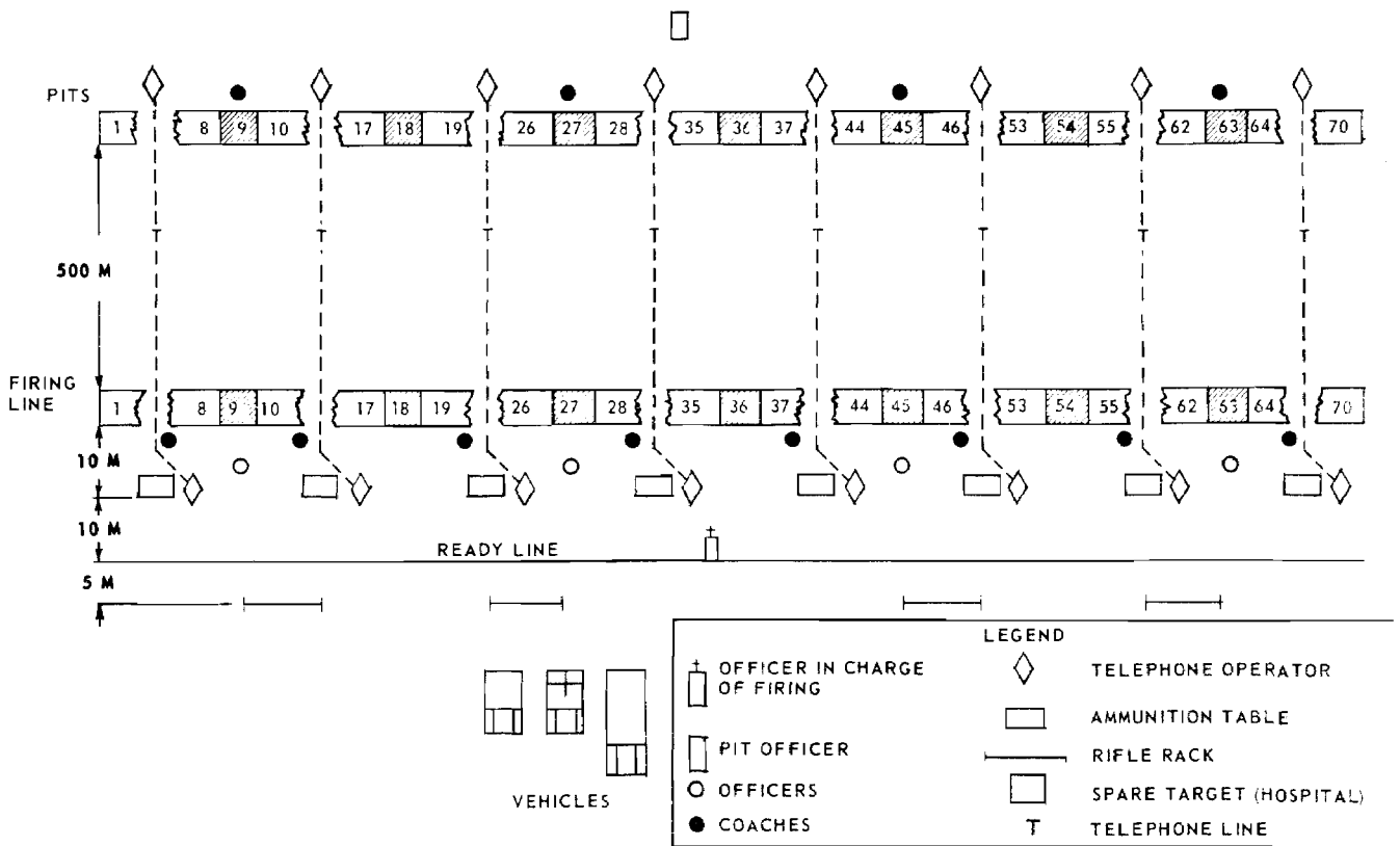
Figure 158. Known distance range construction.
