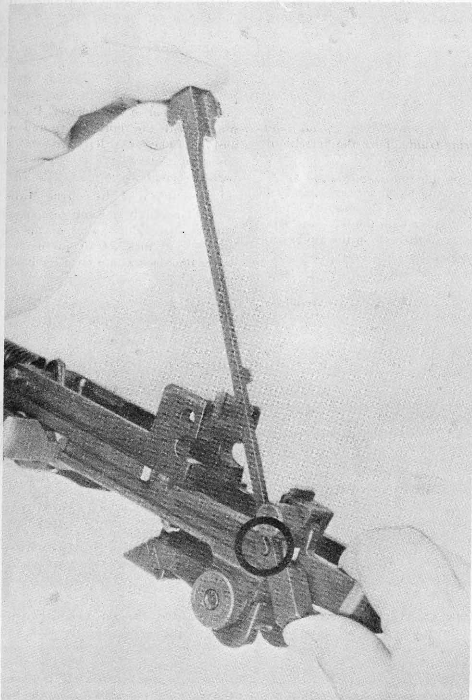
Figure 16. Replacing the connector assembly.
