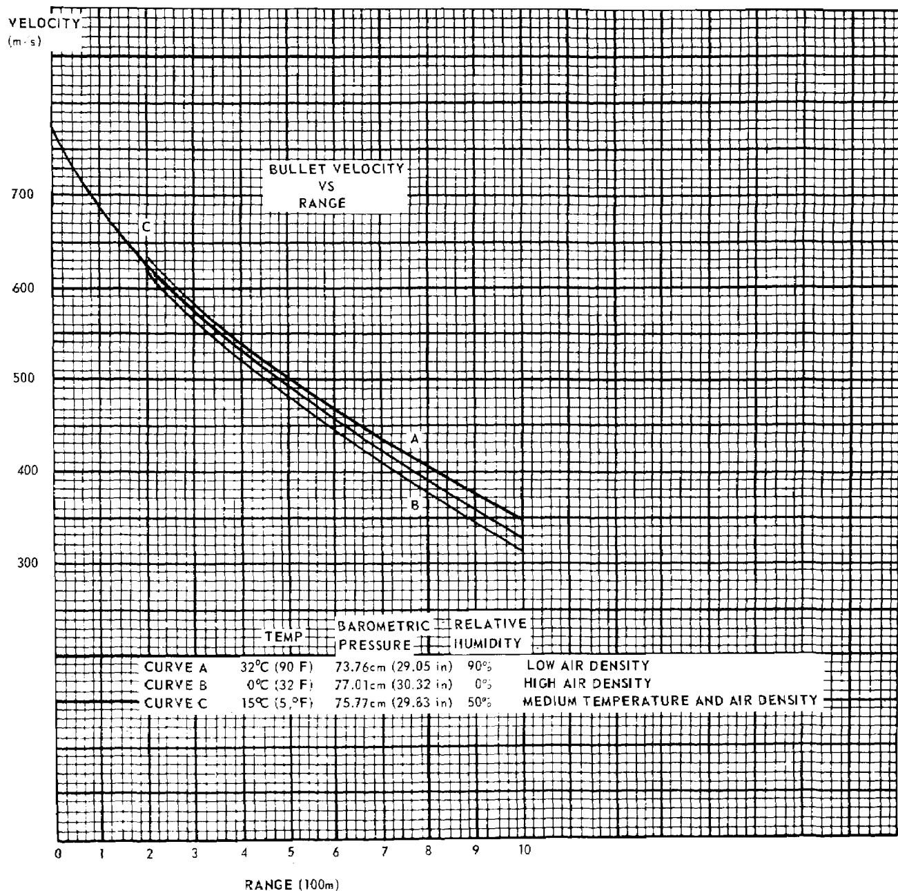
Figure 151. Chart 3. bullet velocity versus range.
