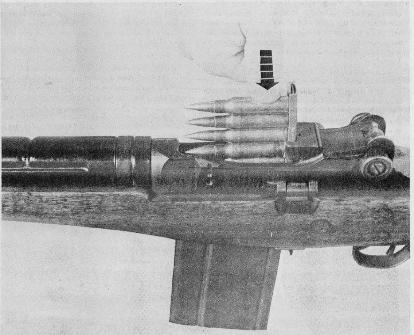
Figure 28. Loading the magazine with a five-round cartridge clip (magazine IN rifle).
