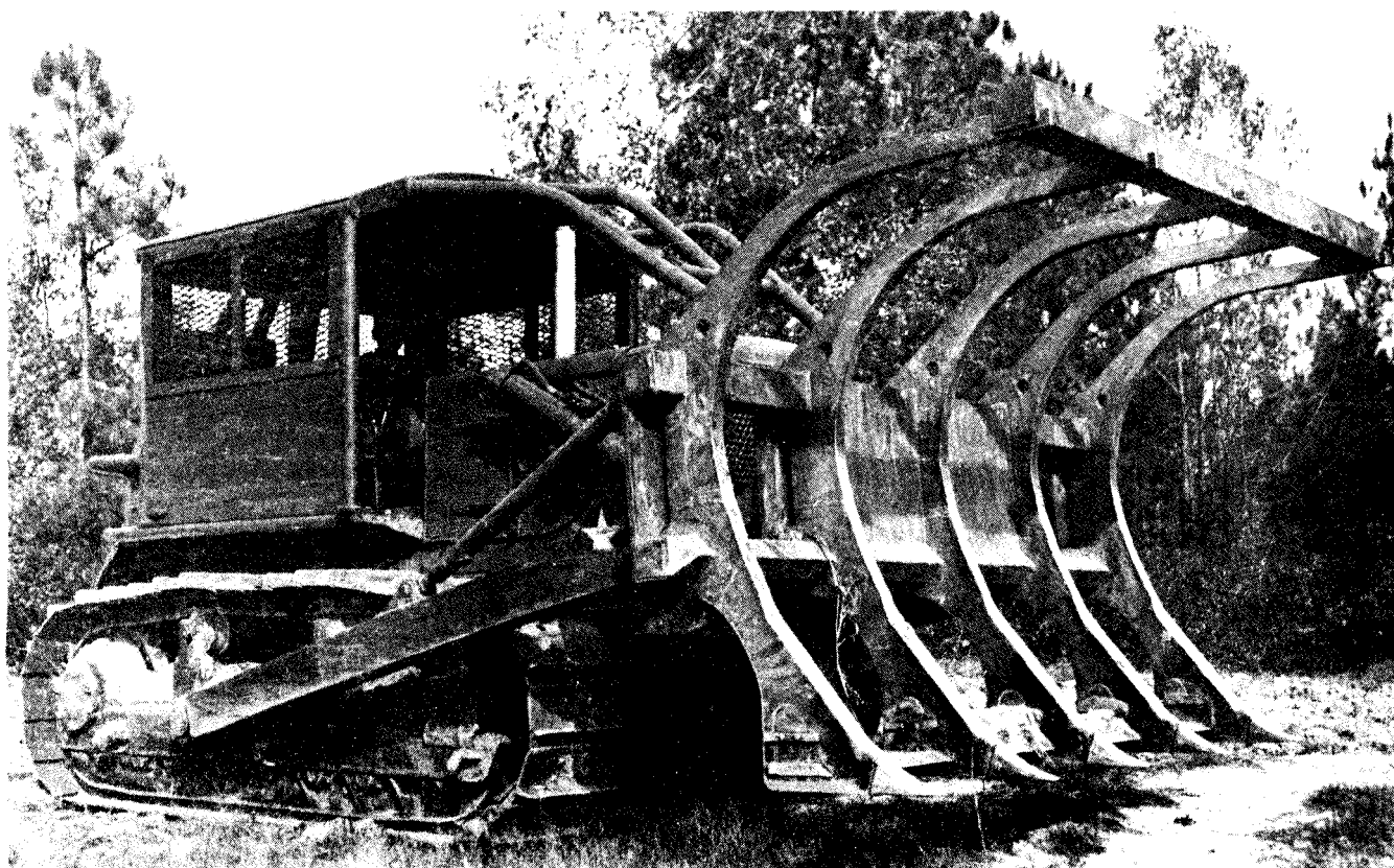
Figure 3-9. Spade plow. Note horizontal knockdown beam on top and cutting blade on bottom.
