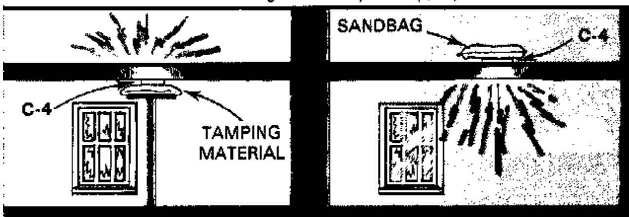
Figure E-2b Breaching with Claymore (C-4)
