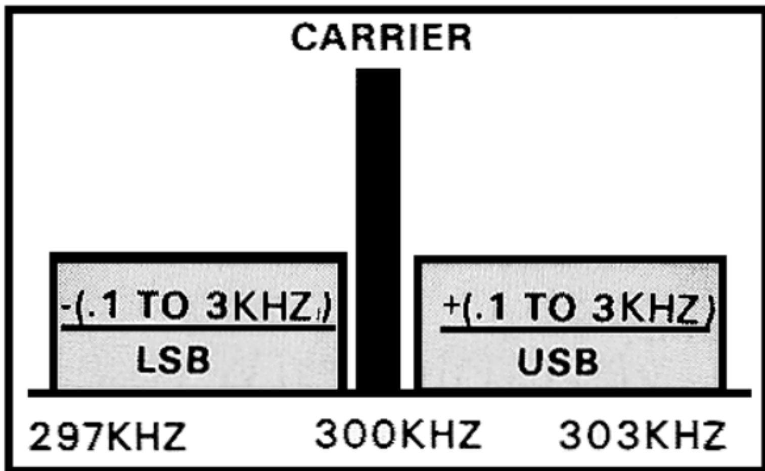
Figure 2-18. Amplitude-modulated system.
