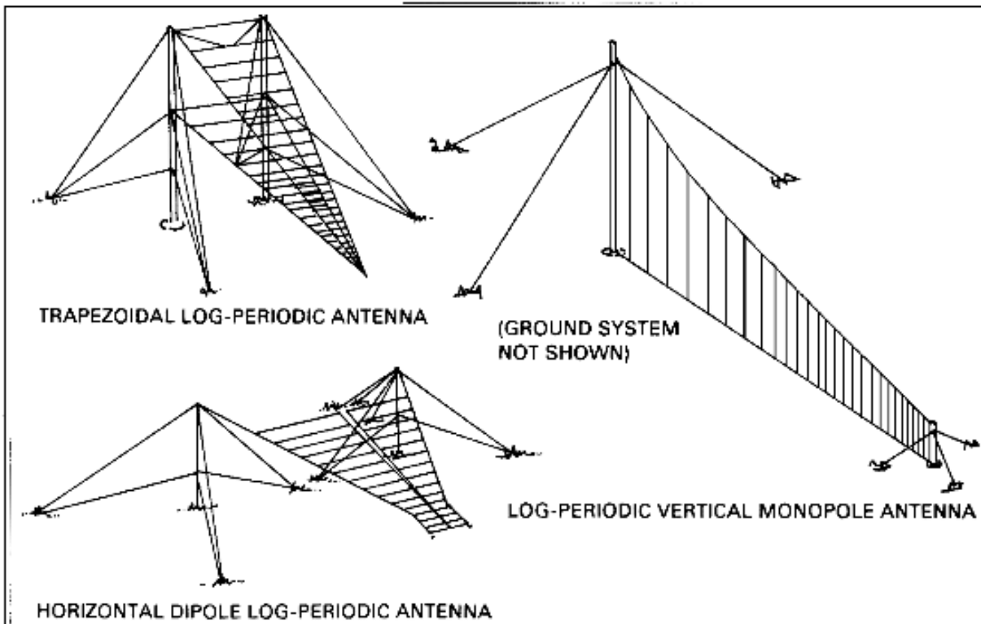
Figure 3-20. Log periodic antenna.
