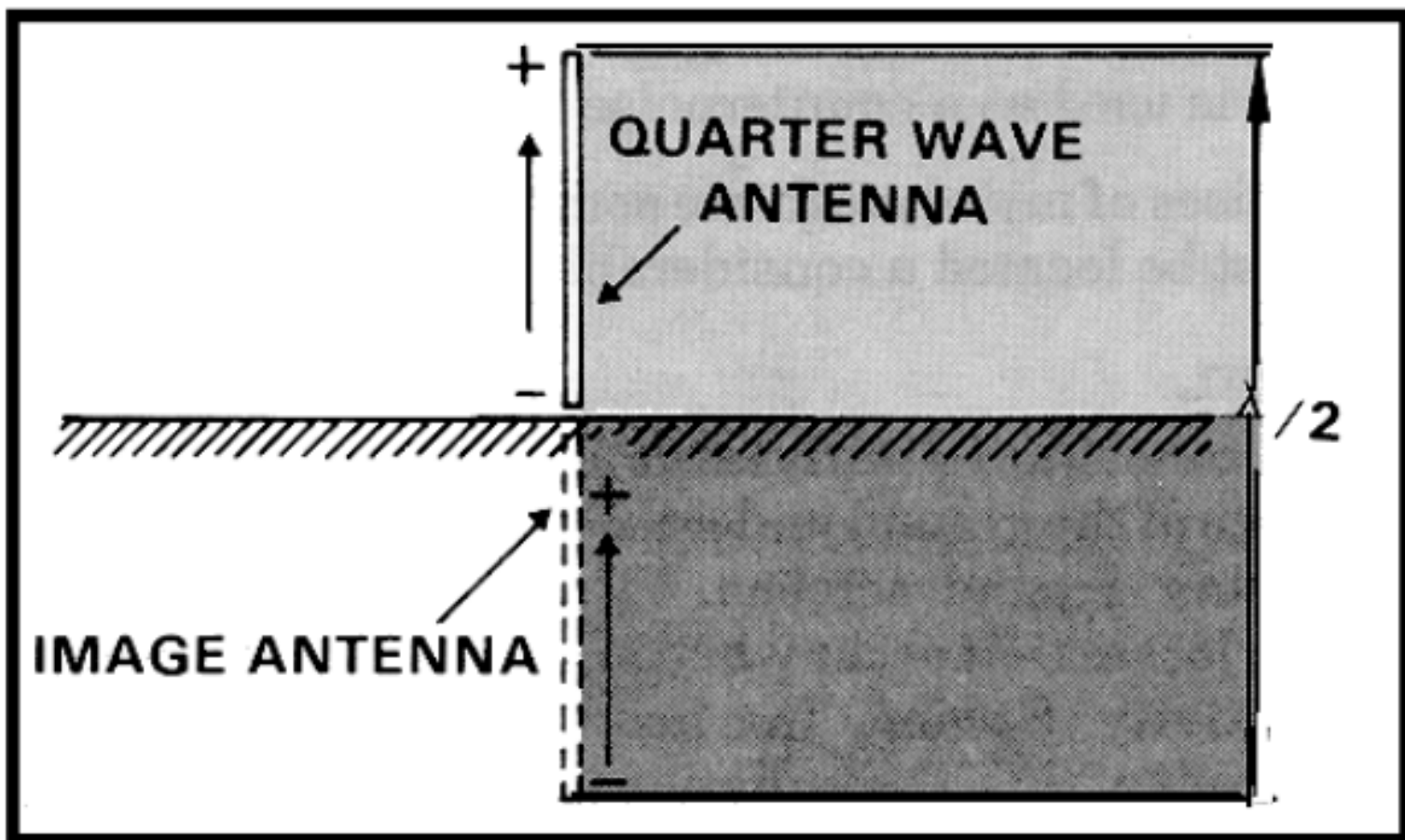
Figure 3-7. Quarter-wave antenna connected to ground.
