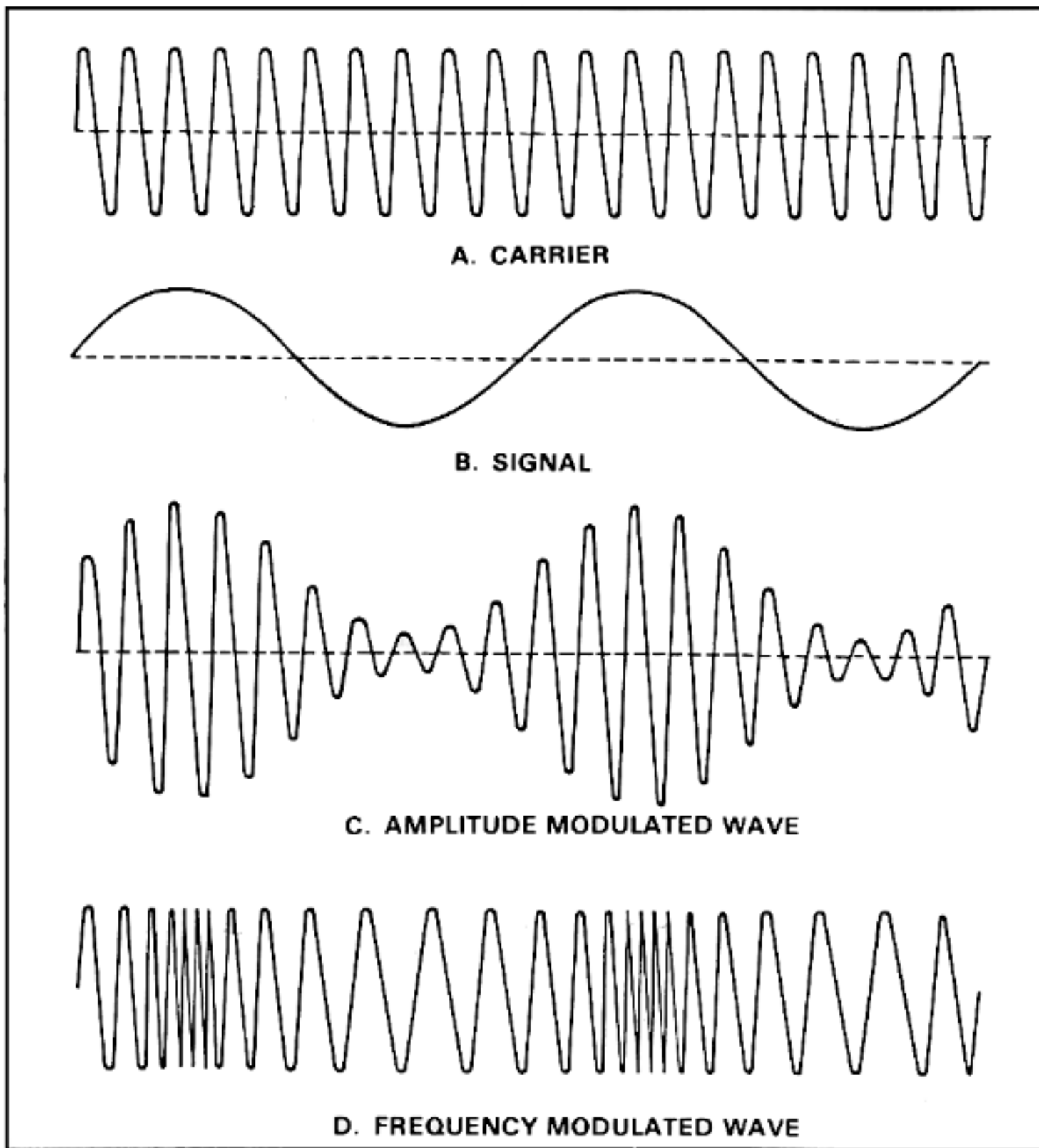
Figure 2-17. Wave shapes.
