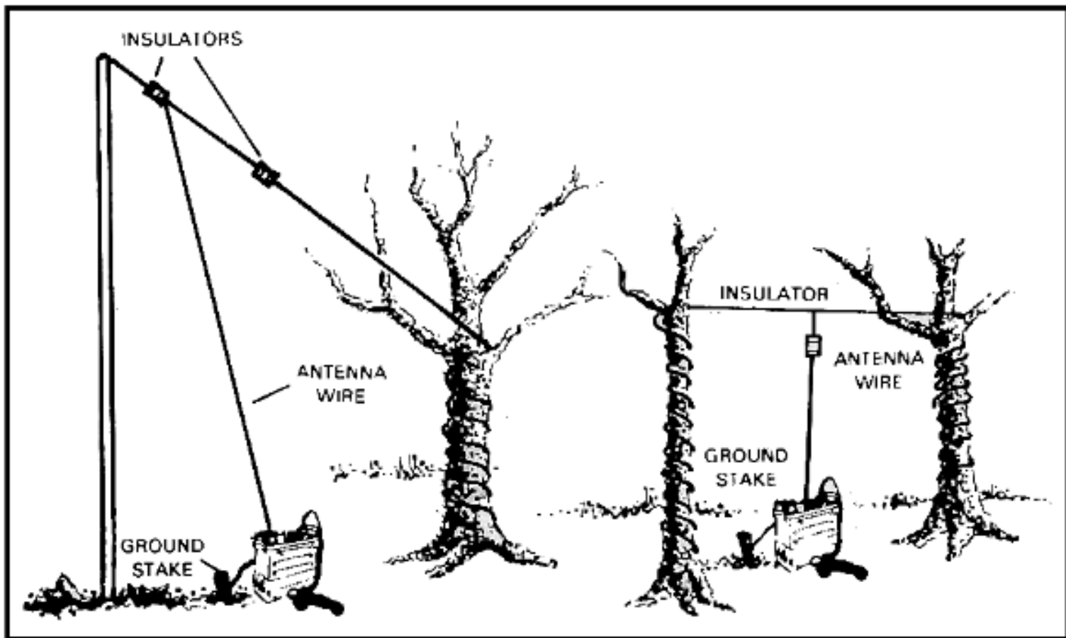
Figure 3-30. Additional means of supporting vertical wire antennas.
