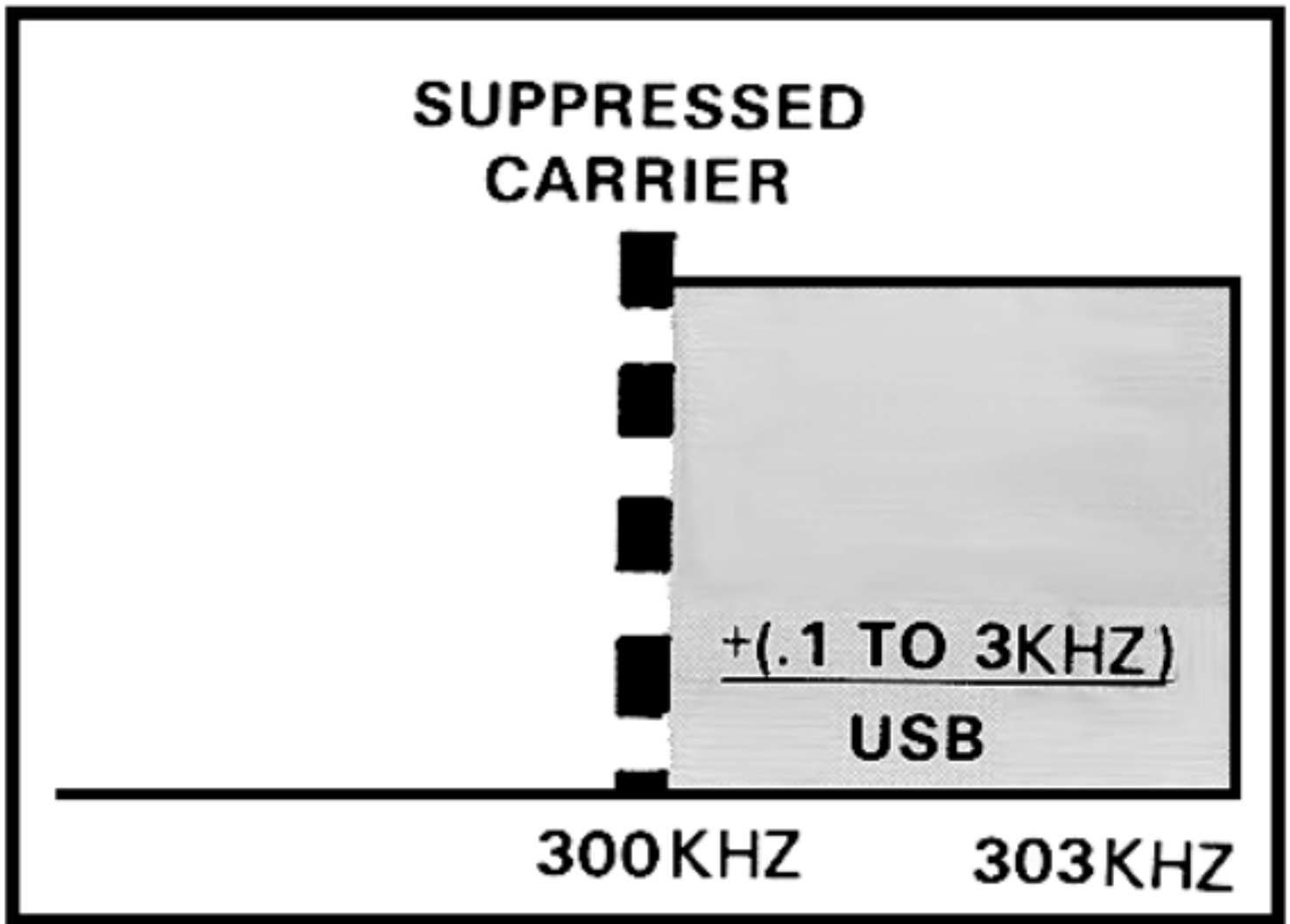
Figure 2-19. Single-sideband system.
