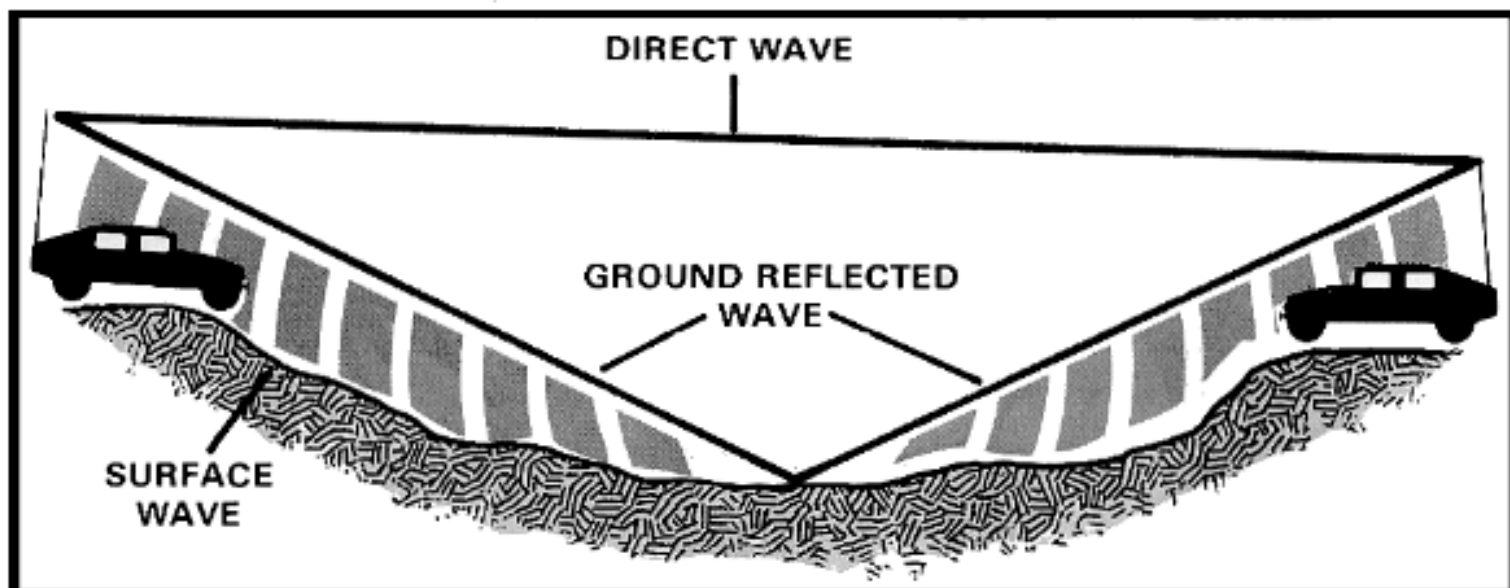
Figure 2-12. Possible routes for ground waves.
