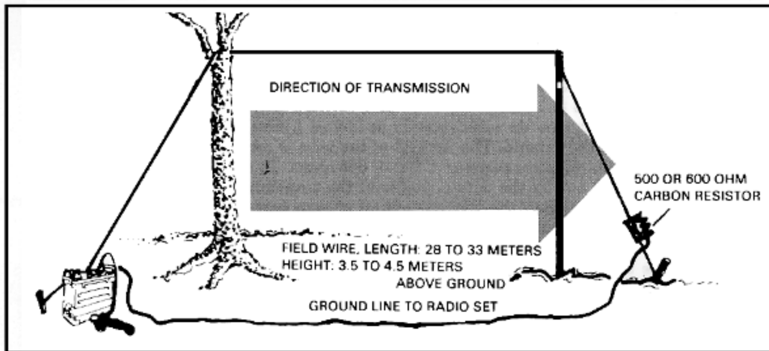
Figure 3-37. Long-wire antenna.
