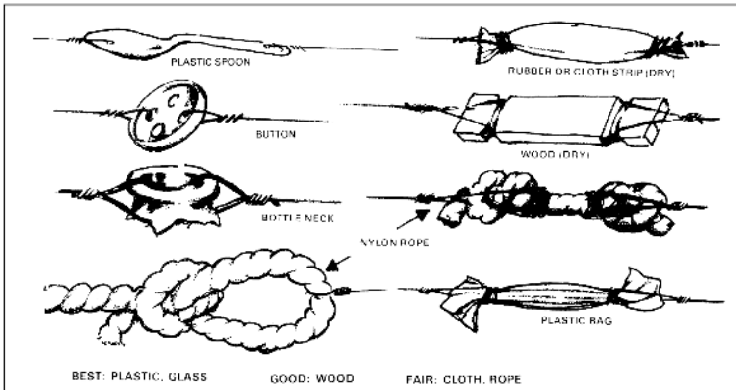
Figure 3-26. Improvised insulators.
