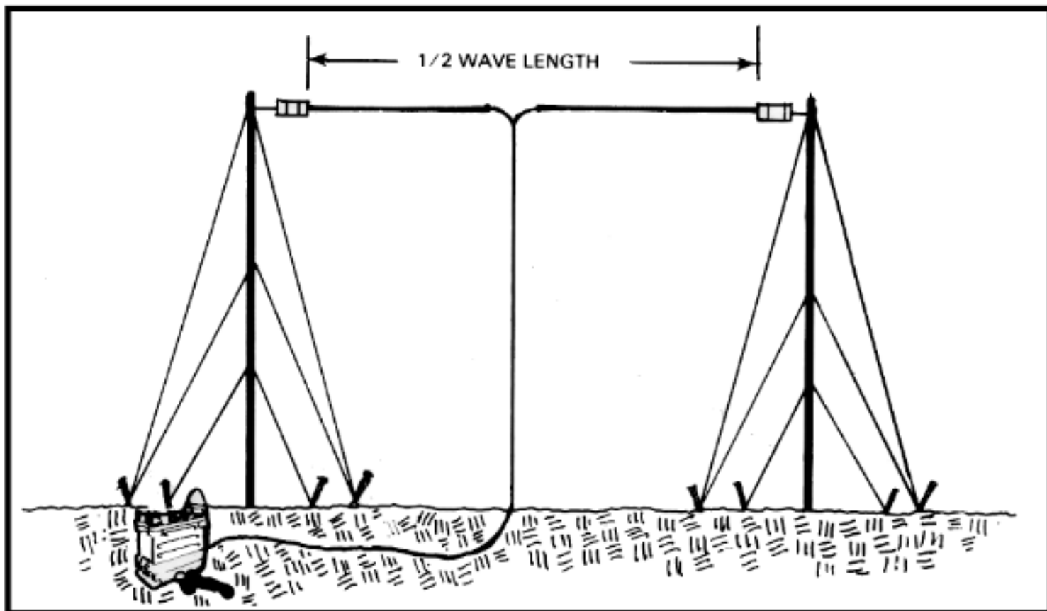
Figure 3-12. Center-fed Hertz antenna with two upright supports.
