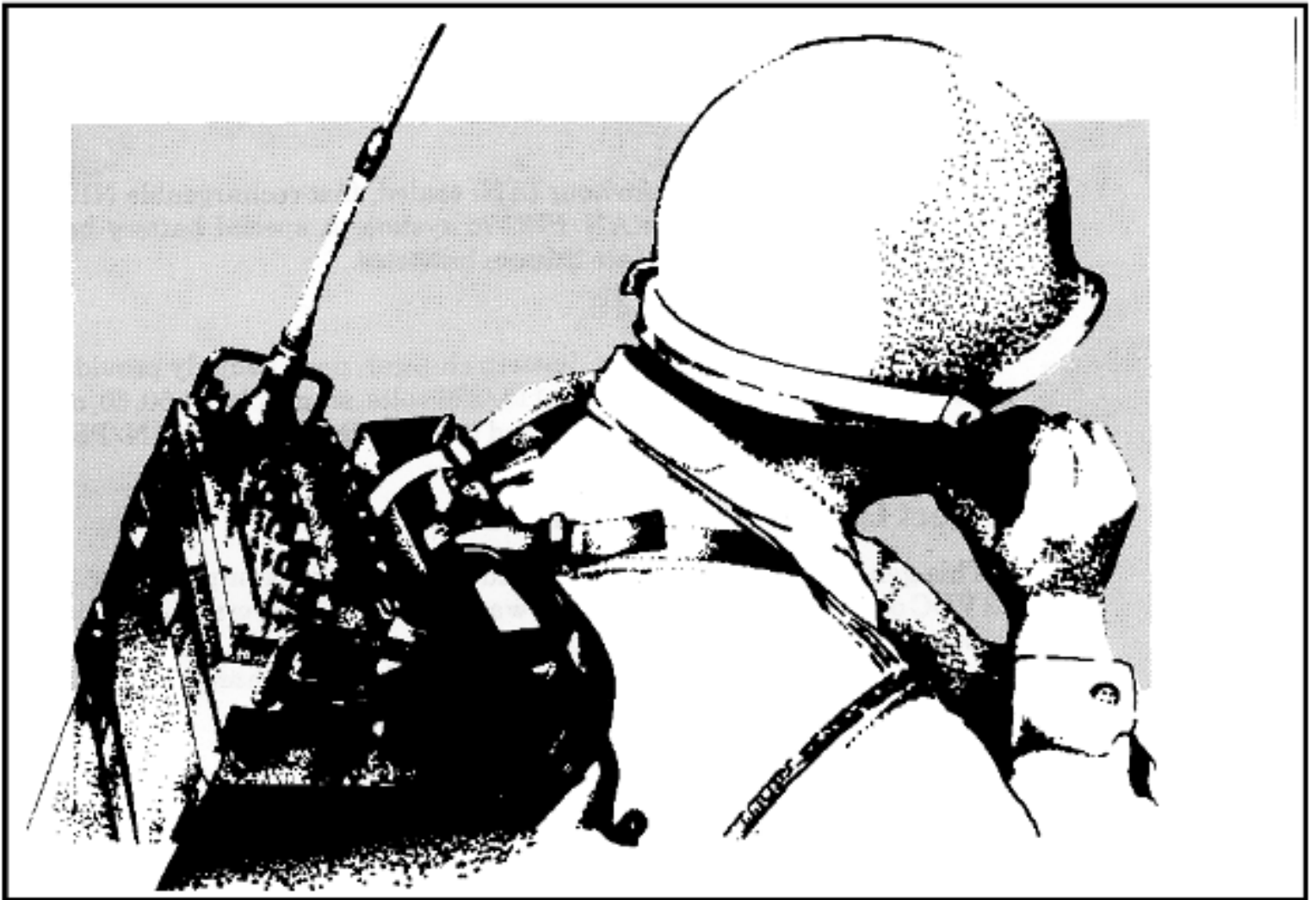
Figure C-1. AN/PRC-70 Manpack.
