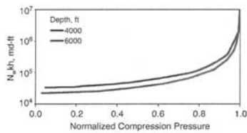
Fig. 2. Relationship between well count, permeability-thickness, and the compression pressure as a fraction of ΔP max for given relative permeability, ΔP max , and aquifer depth.
