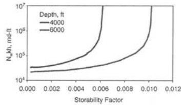
Fig. 3. Relationship between well count, permeability-thickness, and the storability factor for given relative permeability, ΔP max , and aquifer depth.
