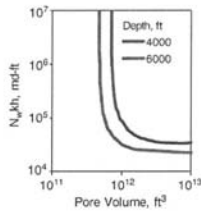
Fig. 1. Relationship between well count, permeability-thickness, and the required minimum pore volume for given relative permeability, ΔP max , and aquifer depth.
