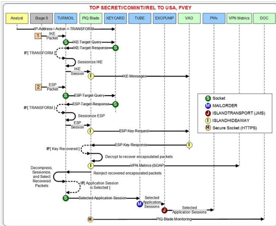
(TS//SI//ORCON//REL) VPN Decryption Sequence
