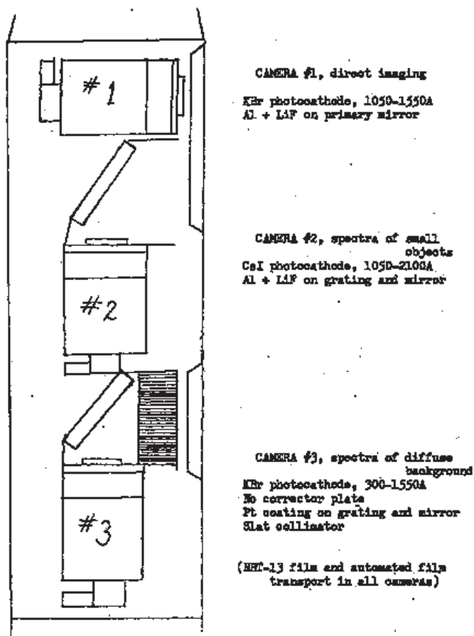
Figure 5. Cameras for Apollo-150 Trial Flight
