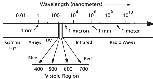
Electromagnetic Spectrum
