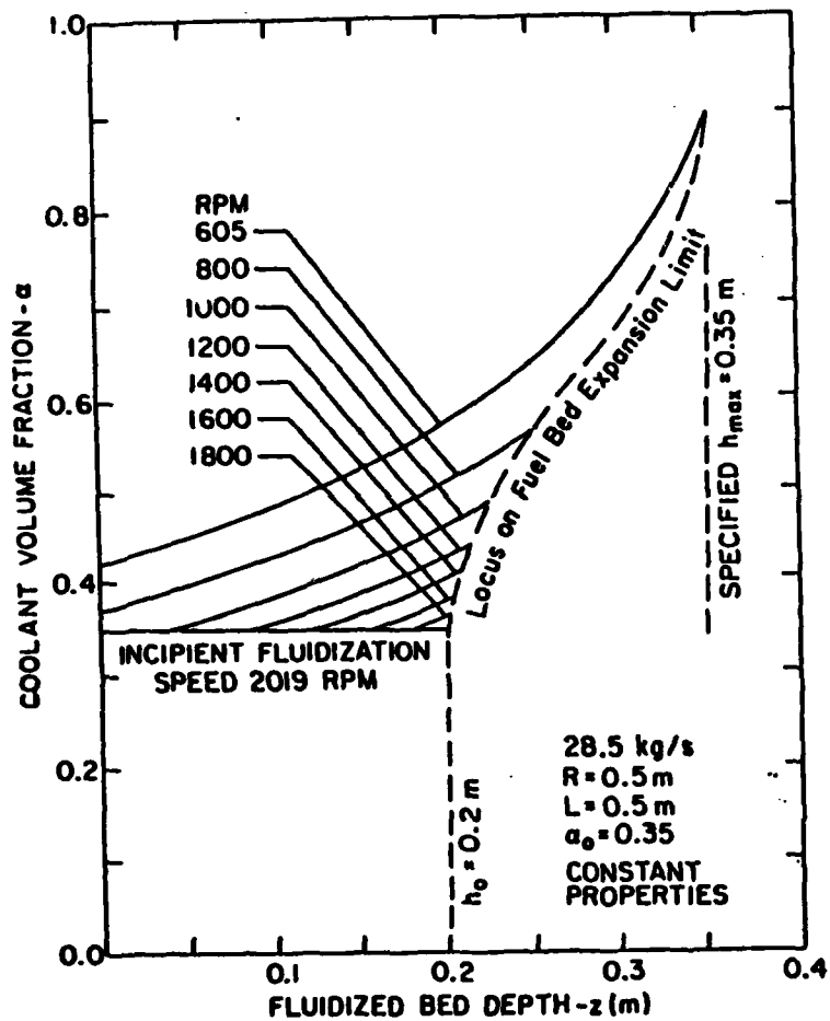
Figure 6 Calculated adiabatic thick bed expansion
