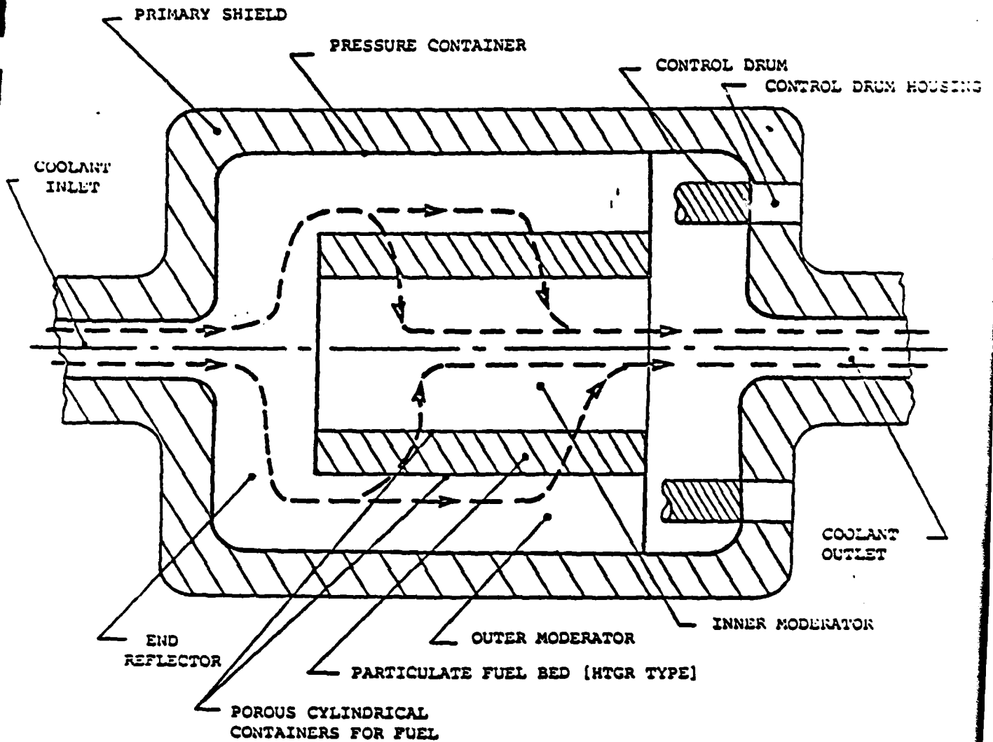
Figure 12: High Power Density Space Reactor ( H_2O or Gas Coolant). Note: Support ribs for the reactor are not shown. Outer and inner moderator regions also provide radial reflector zones which may be made of either H_2O or ZrH_2 . Control drums extend into the outer moderator/reflector region. The fuel bed dimensions are typically of the order of 45 cm in length and 30 cm in diameter.
