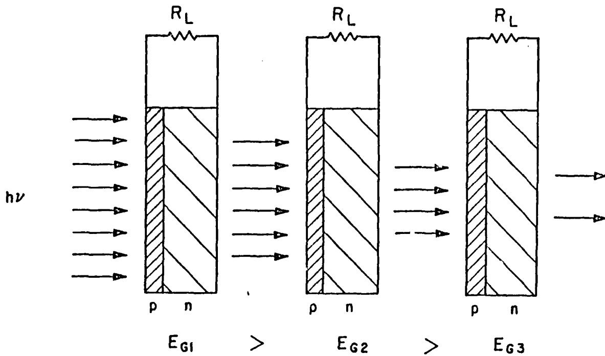
Fig. 1. Schematic representation of a three semiconductor tandem cell system.
