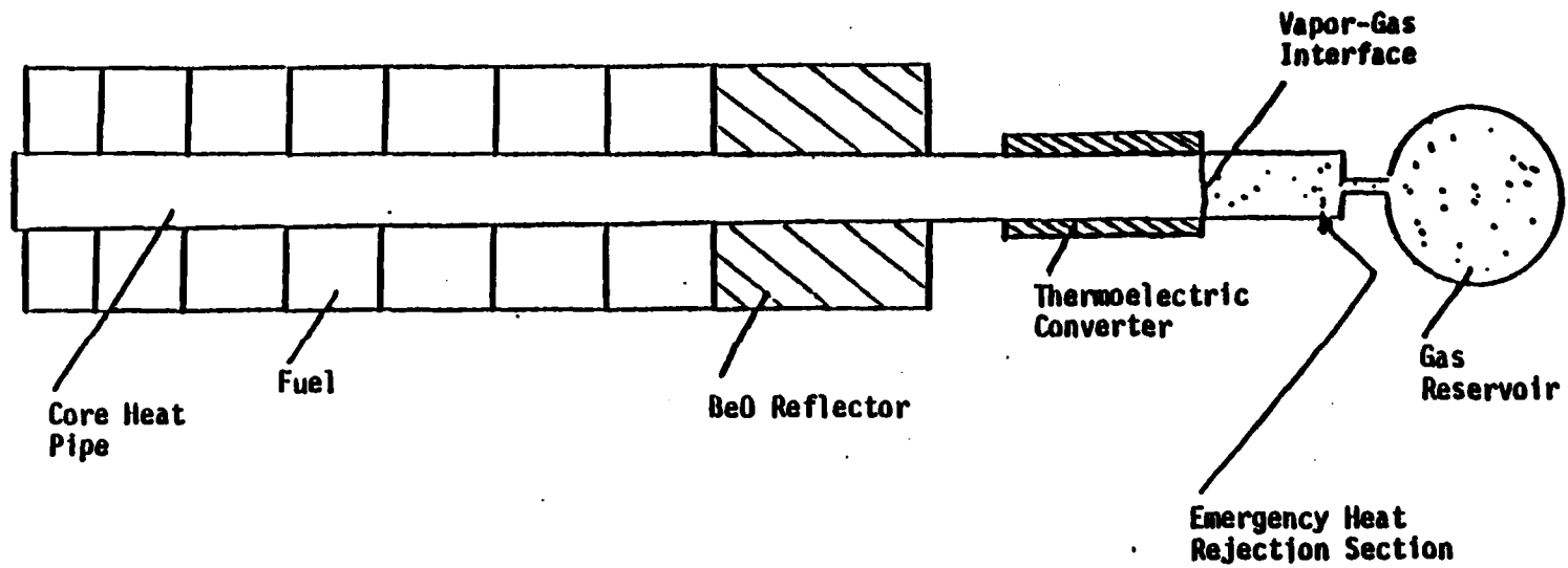
Figure 5. Heat pipe design for emergency cooldown of reactor core.
