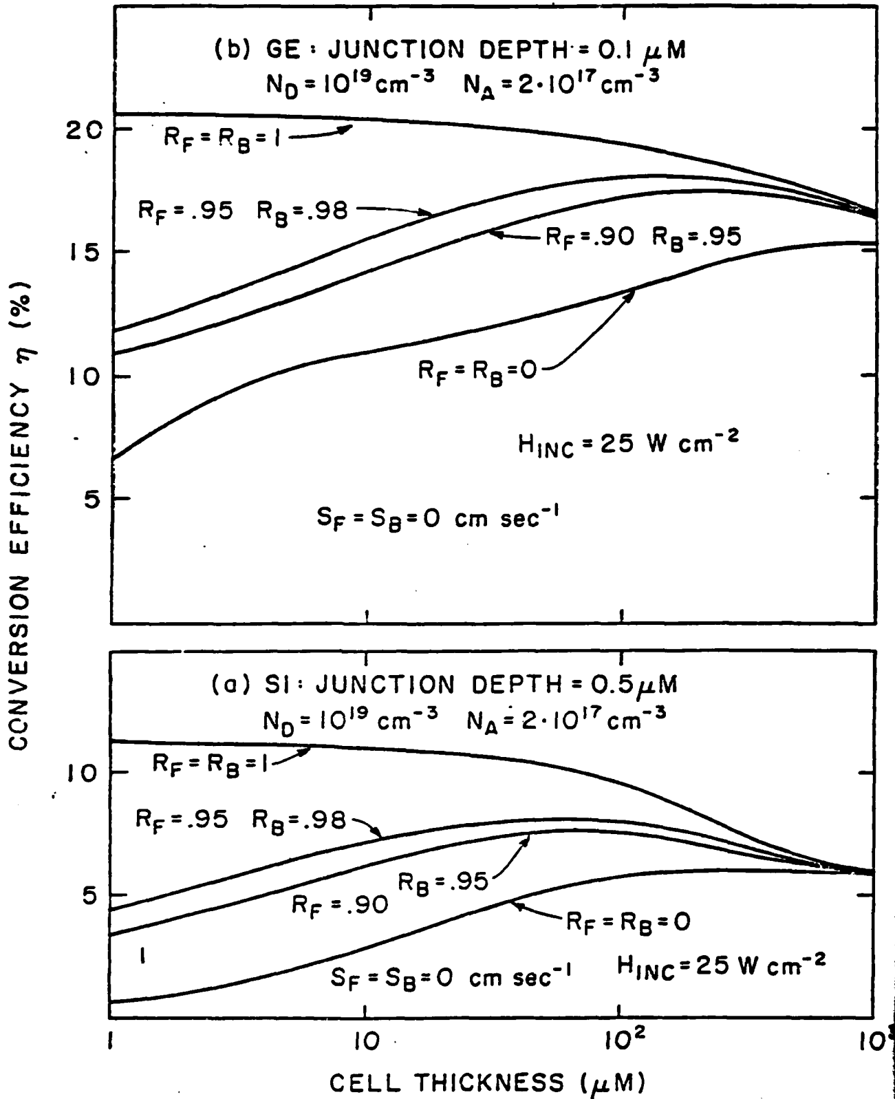
Calculated conversion efficiency versus cell thickness with reflectivity of the front ( R_F ) and reflectivity of the back ( R_B ) as parameters for: (a) silicon and (b) germanium p-n junctions.
