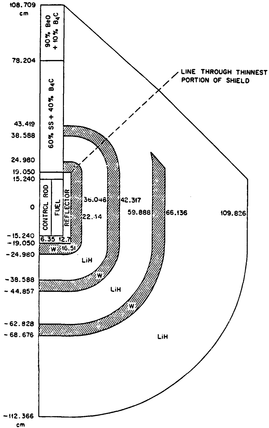
Preliminary configuration for asymmetric shield with a 90-deg. cone angle (450 kw).
