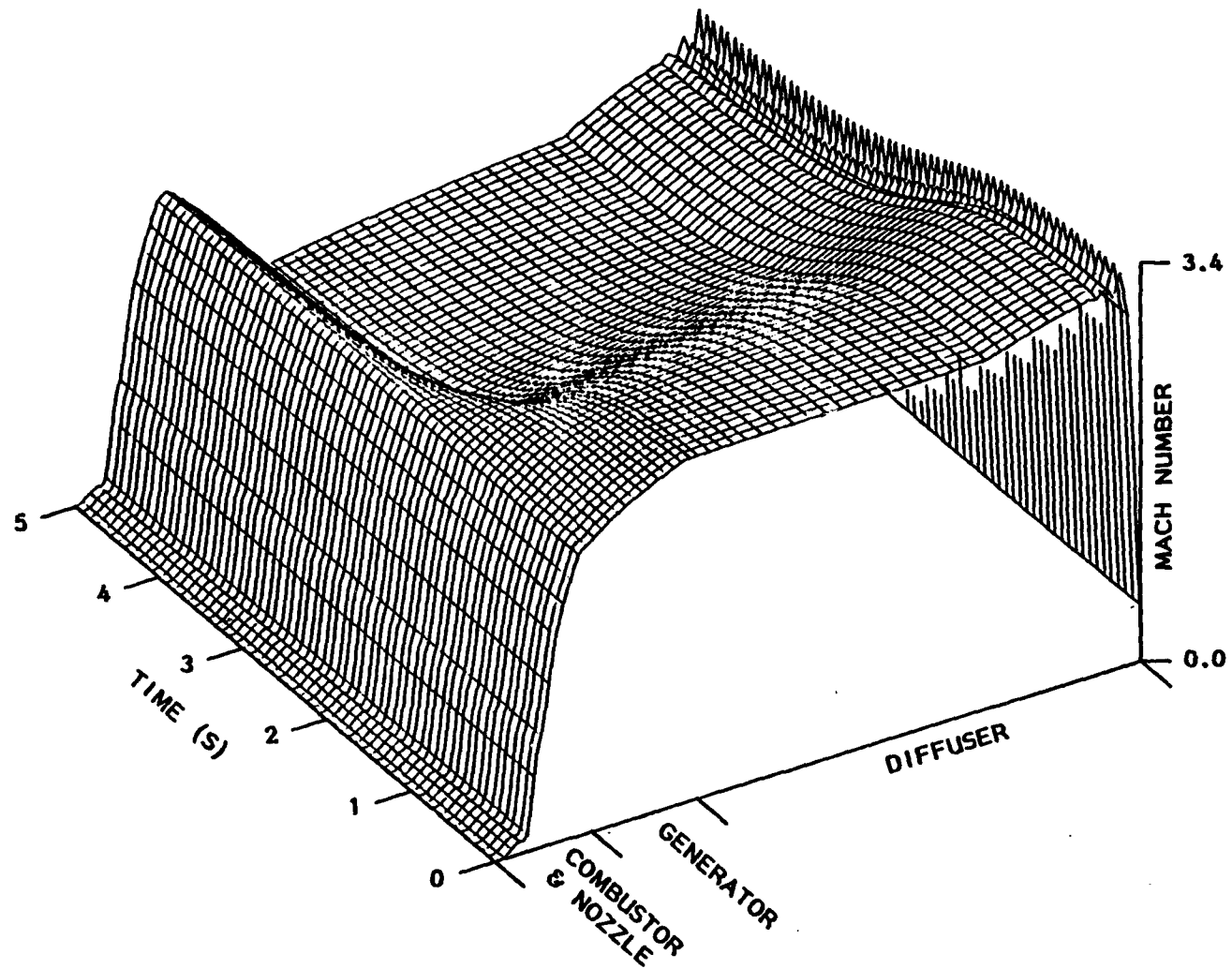
Fig. 21. Space and time variation of the Mach number M for optimum self-excitation of the split-load continuous electrode Faraday channel. Peak Mach Number is 3.4.
