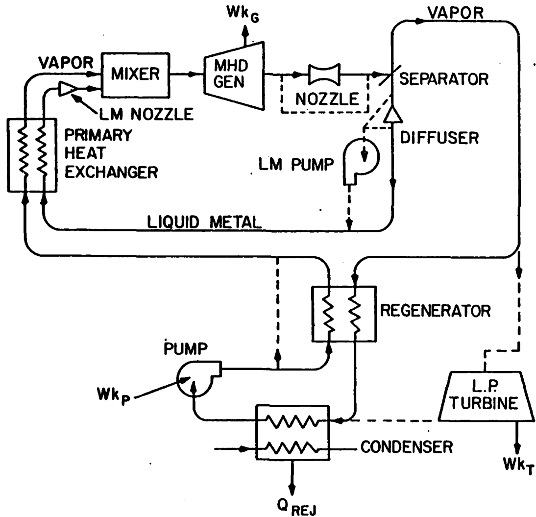
SCHEMATIC OF LMMHD RANKINE CYCLE
