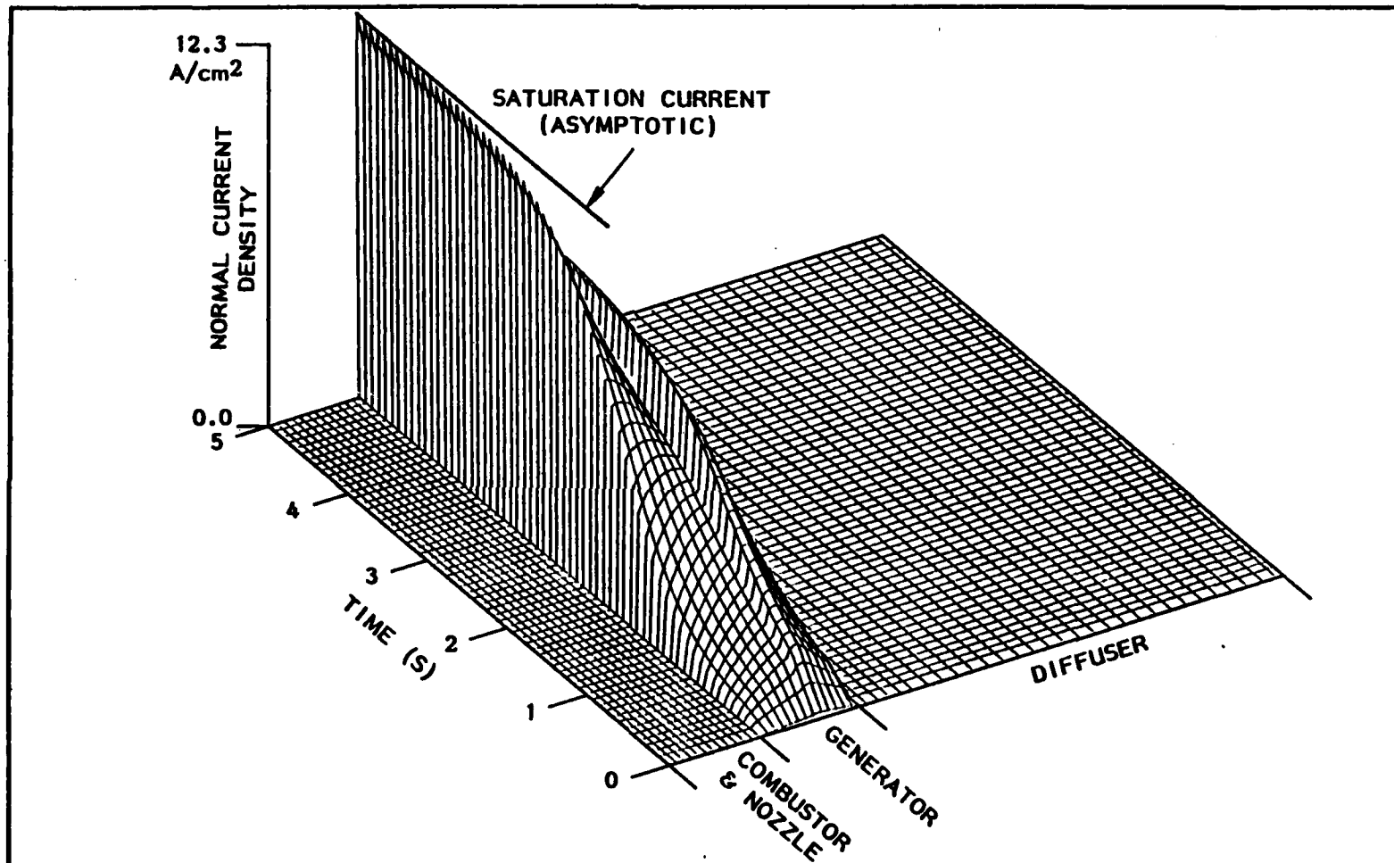
Fig. 20 . Space and time variation of the normal current density component J_y for optimum self-excitation of the split-load continuous electrode Faraday Channel, Peak current density is 12.3 A/cm 2 .
