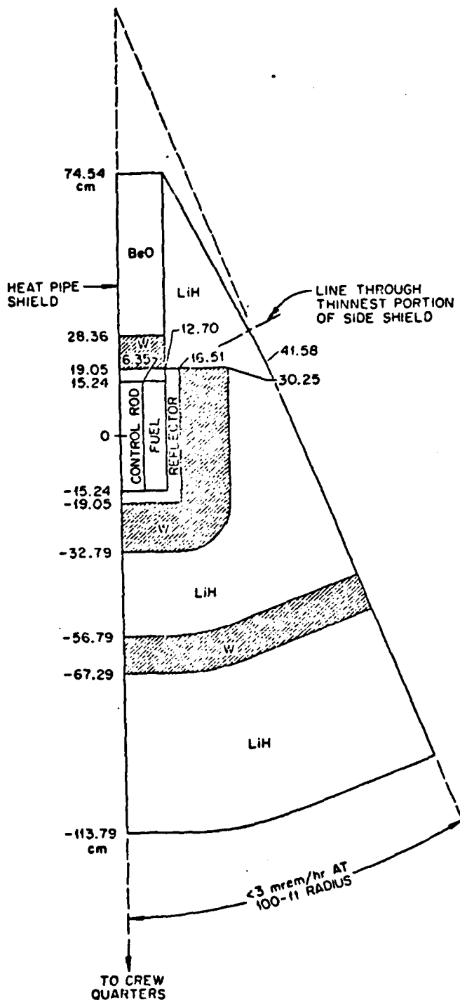
Fig. 10. Configuration for a Two-Cycle Asymmetric Shield with a 45-deg Cone Angle (450 kW).
