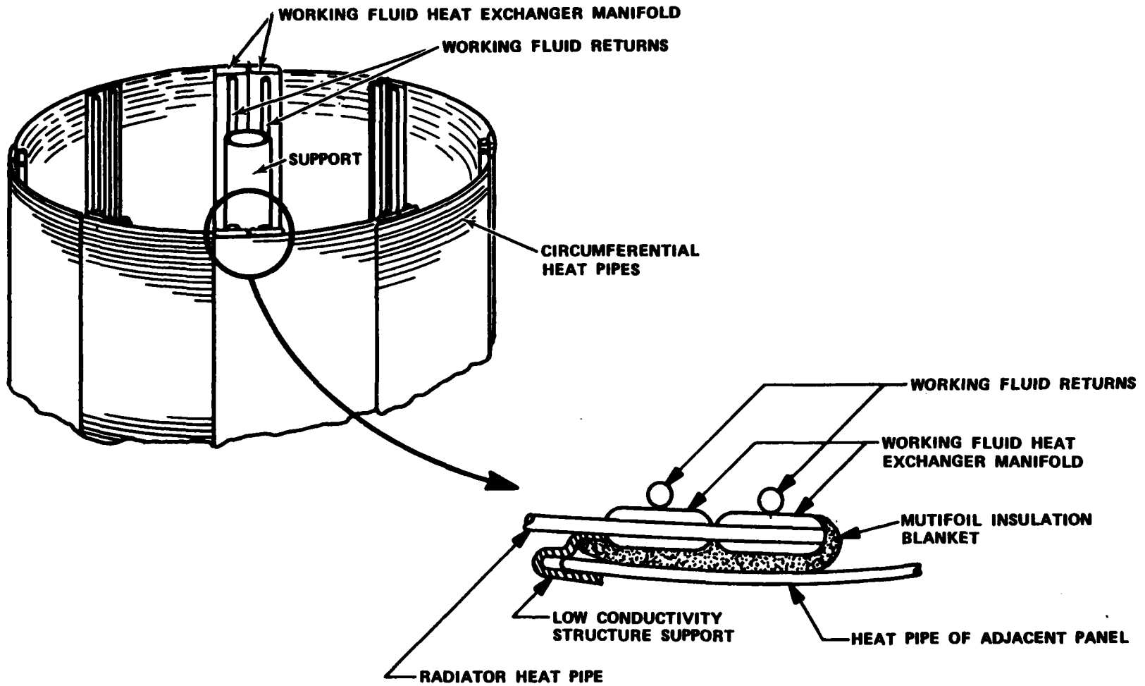
Cylindrical Heat Pipe Radiator Conceptual Design
