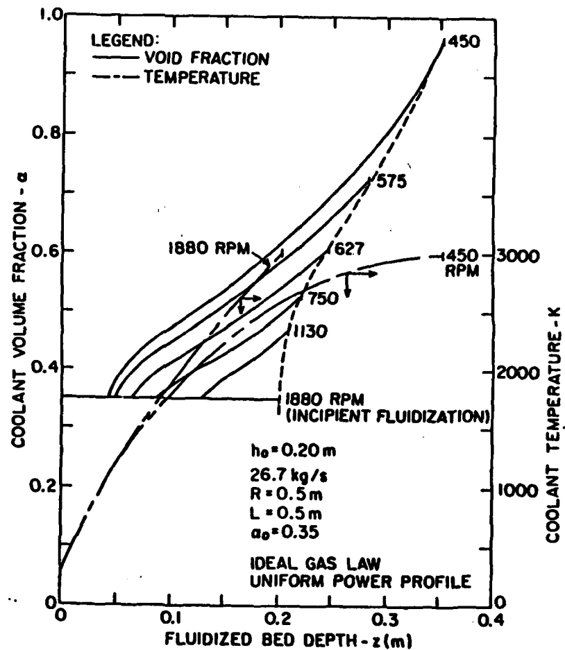
Figure 7 Calculated thick bed expansion for heated hydrogen
