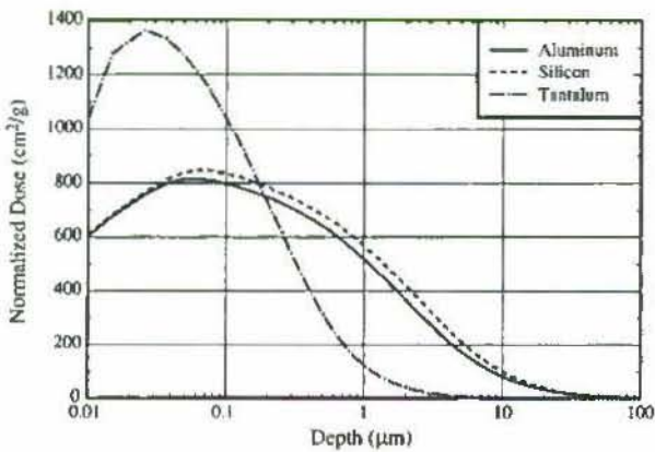
Figure VI.3(a). Normalized dose as a function of depth in Aluminum ( Z=13 ), Silicon ( Z=14 ) and Tantalum ( Z=73 ) for a 1 keV blackbody.
