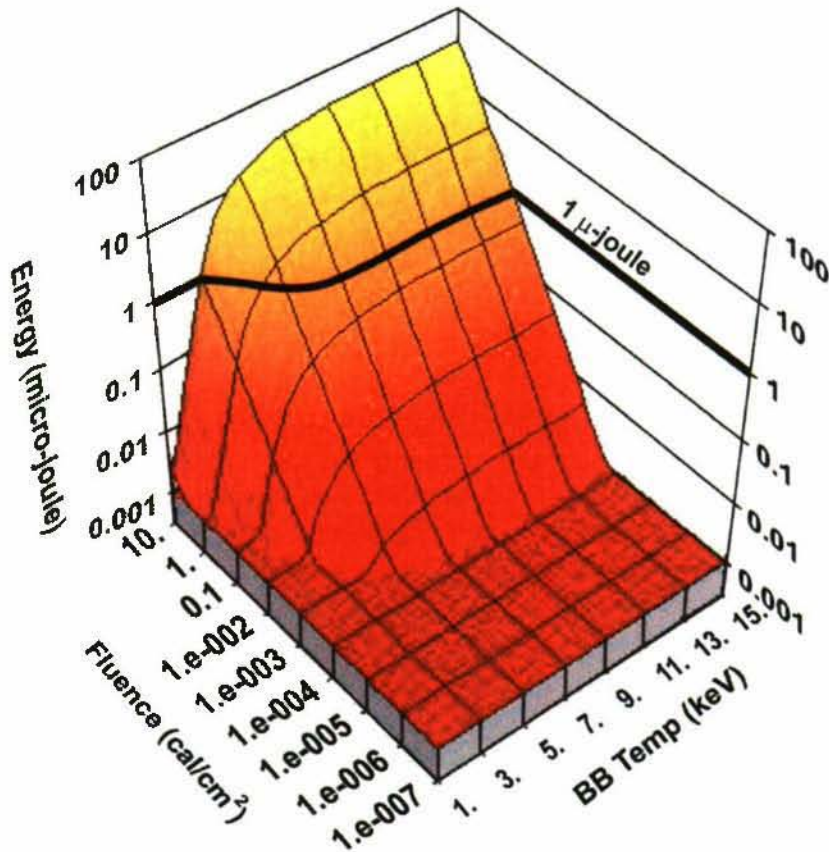
Figure VI.16. Box IEMP Burnout (Uncoated Circuit Board): Energy as function of blackbody temperature and fluence.
