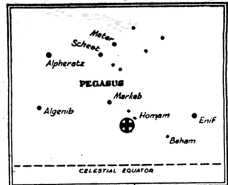
The New York Times APR. 13, 1965 FROM DEEP IN SPACE: Radio source called CTA-102 (cross), in direction of constellation Pegasus, may be sending intelligent radio emissions, Russian believes.
