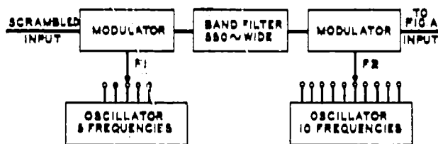
APPLICATION TO SPLIT BAND DECODING
