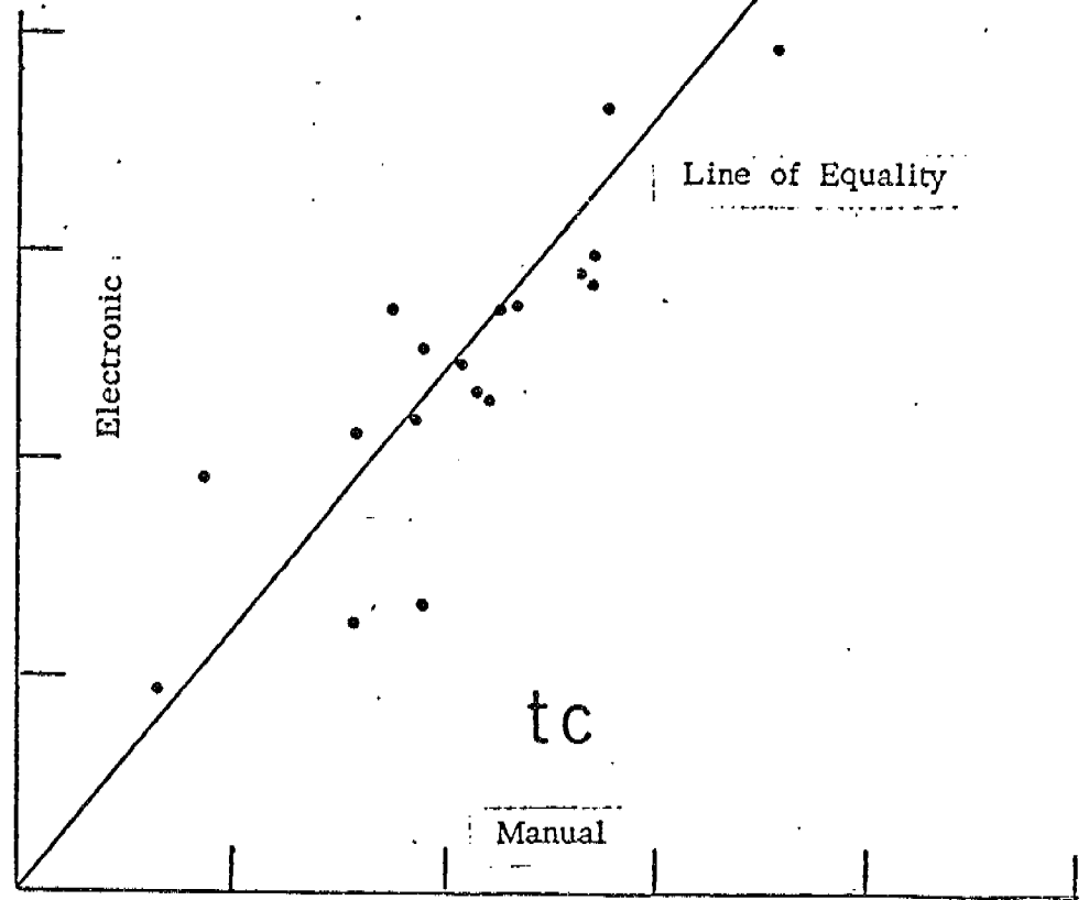
Figure 10. Comparison of manual and electronic measurement of peak first derivative amplitude and of tc .
