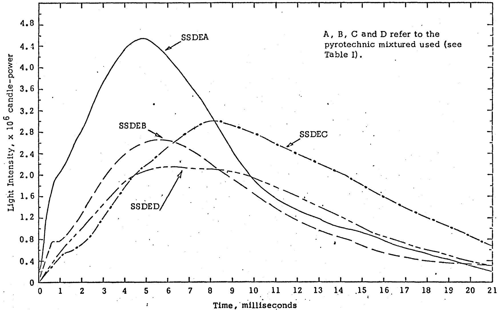
Figure 8. Light Output From Series SSDE Photoflash Units
