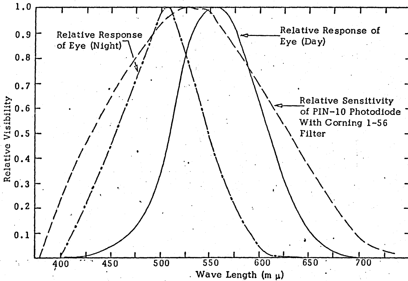
Figure 4. Comparison of Eye and Photodetector Sensitivity Curve.
