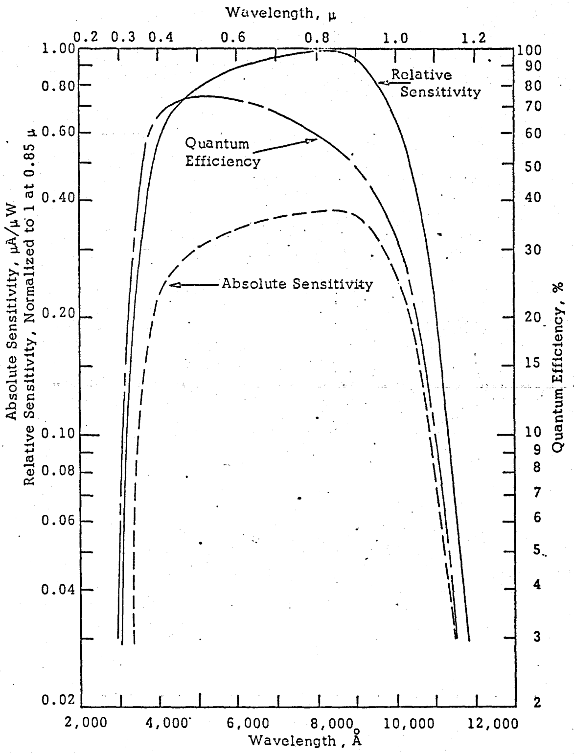
Figure 3. Spectral Characteristics of the United Technology PIN-10 Photodiode
