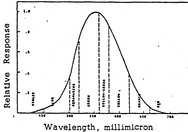
Figure 3. Standard Observer Curve
