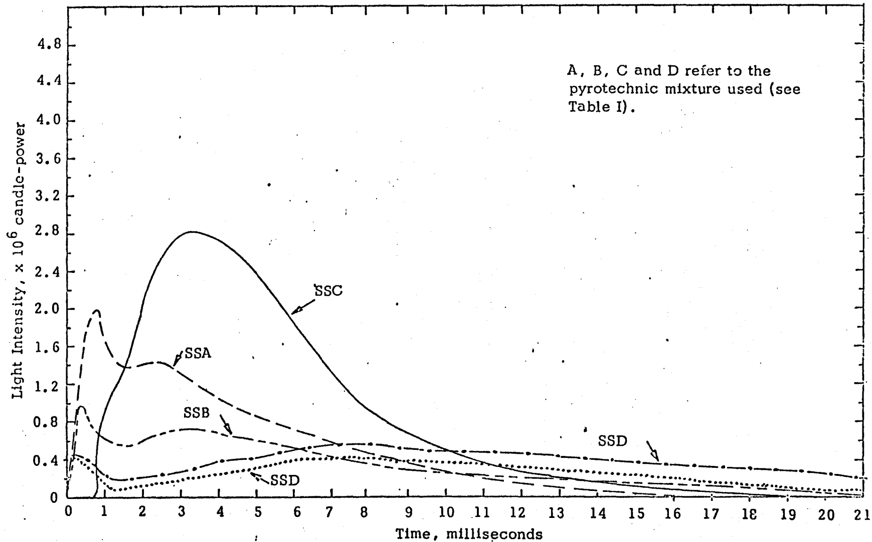
Figure 7. Light Output From Series SS Photoflash Units
