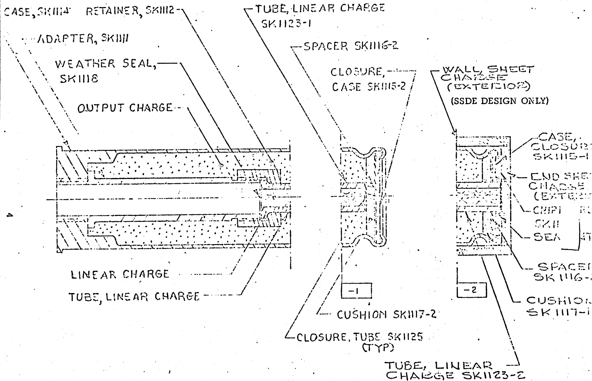
FIGURE 2. 0.83" PHOTOFLASH CARTRIDGE SCALE 2/1
