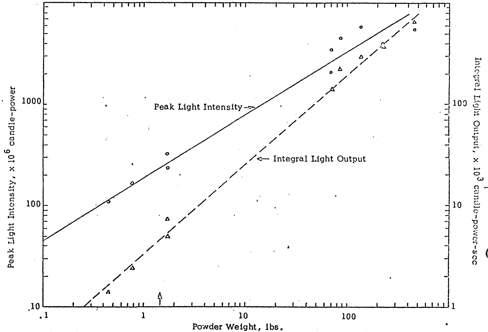
Figure 9. Peak Intensities Produced by Type III Photoflash Mixtures as a Function of Charge Weight 2 .
