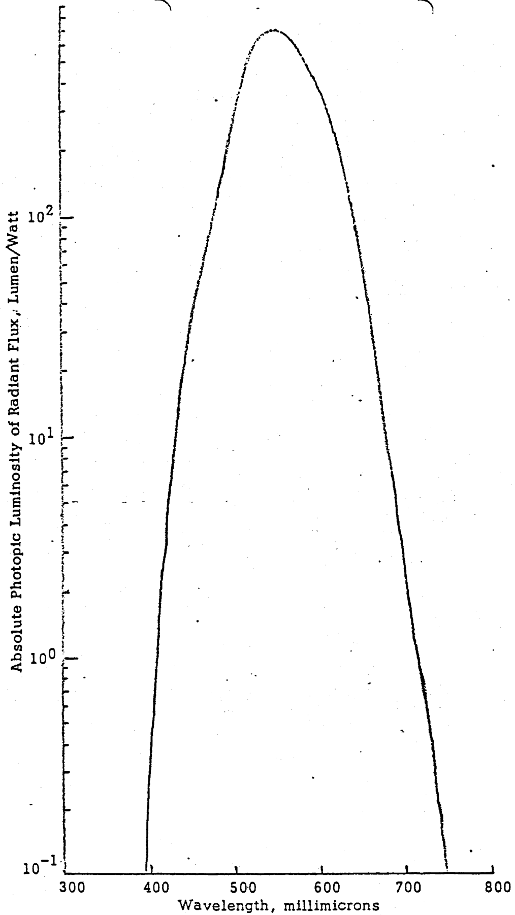
Figure 4. Visual Response Curve of the Human Eye, Spectral Dependence of Luminous Flux (Reference 3)
