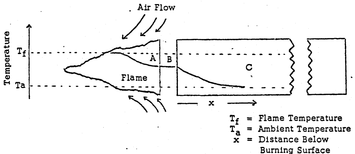
Figure 1. Profile of Combustion Zone
