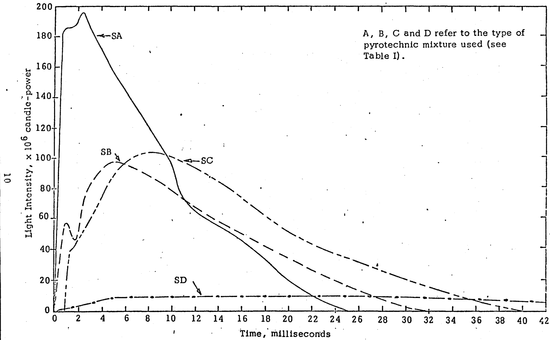
Figure 5. Light Output From Series S Photoflash Units
