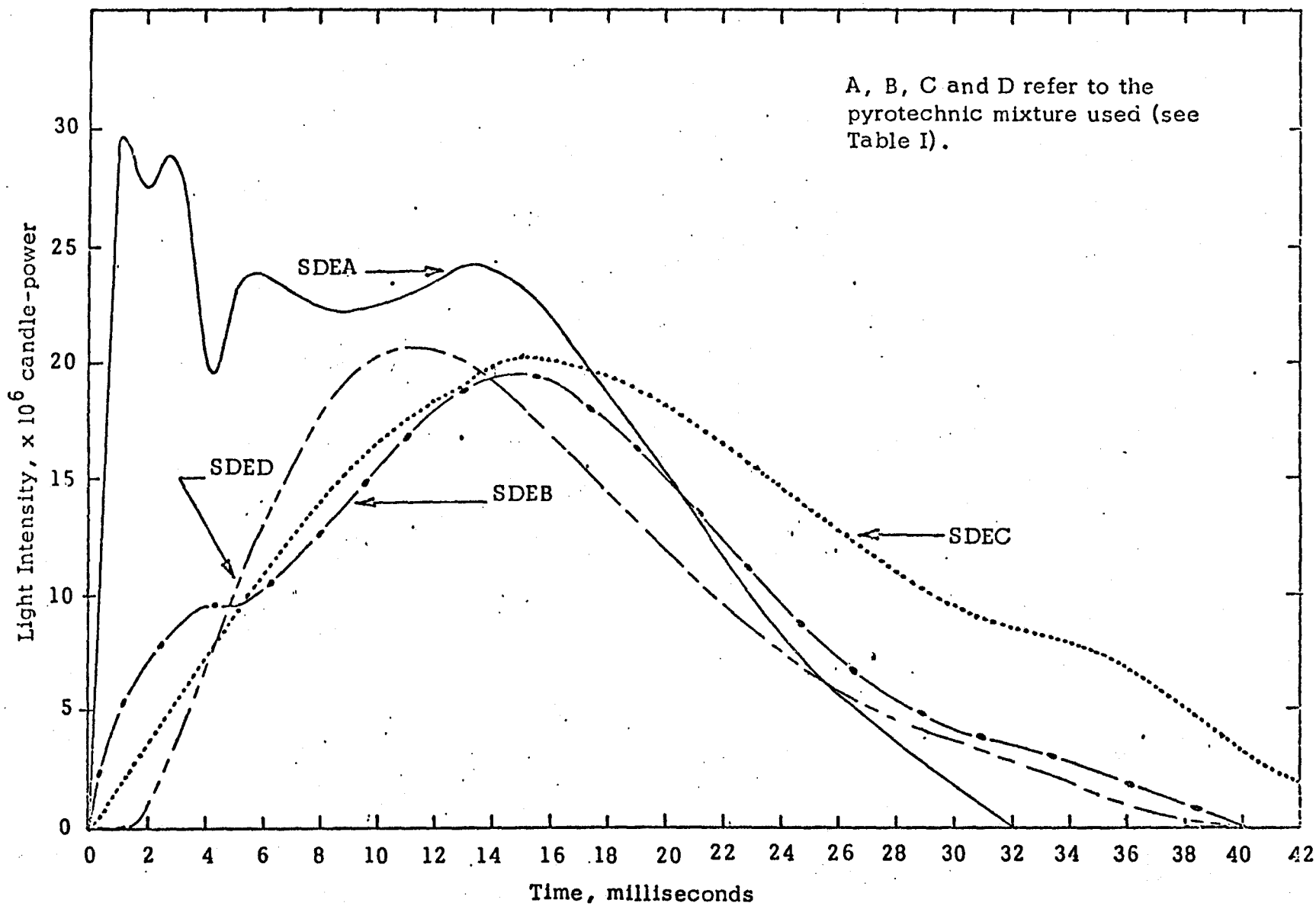
Figure 6 Light Output From Series SDE Photoflash units
