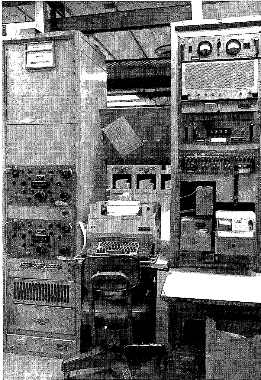
AG-22 - Configured Morse Position at [redacted] (R-390 receivers are in the left-hand rack; MOD-35 in the center; and tape unit on the right)
