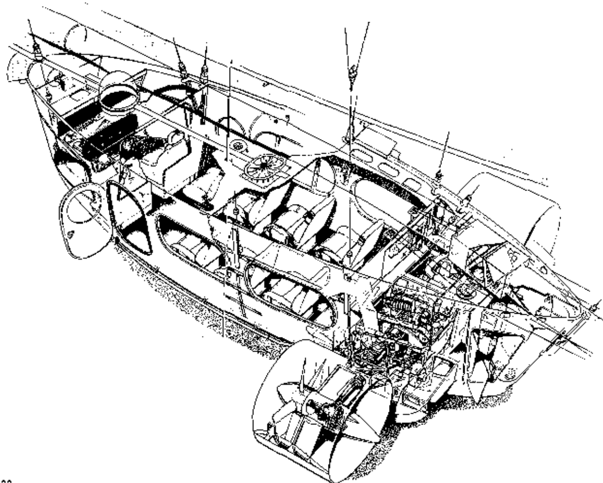
21, section of cockpit—controls above the pilot are for the admission and release of air into the ballonets. 22, gondola of Skyship 500; the only significant metal parts are those making up the Porsche engines and Lynx helicopter transmission. The rest of the structure is made of new generation materials.
