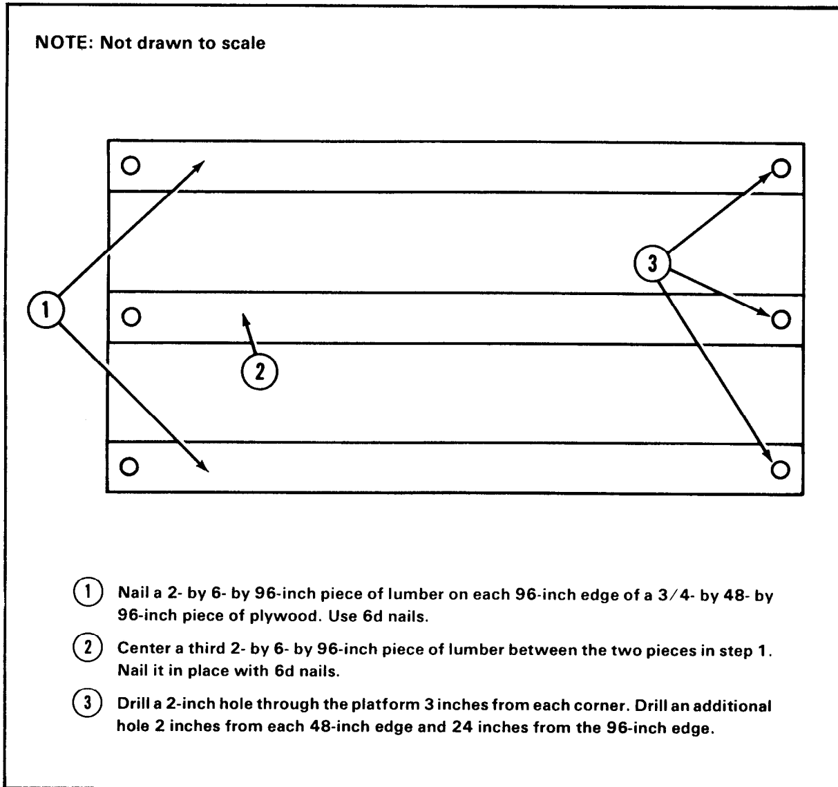
Figure 3-14. Construction details for parachute stowage platform.
