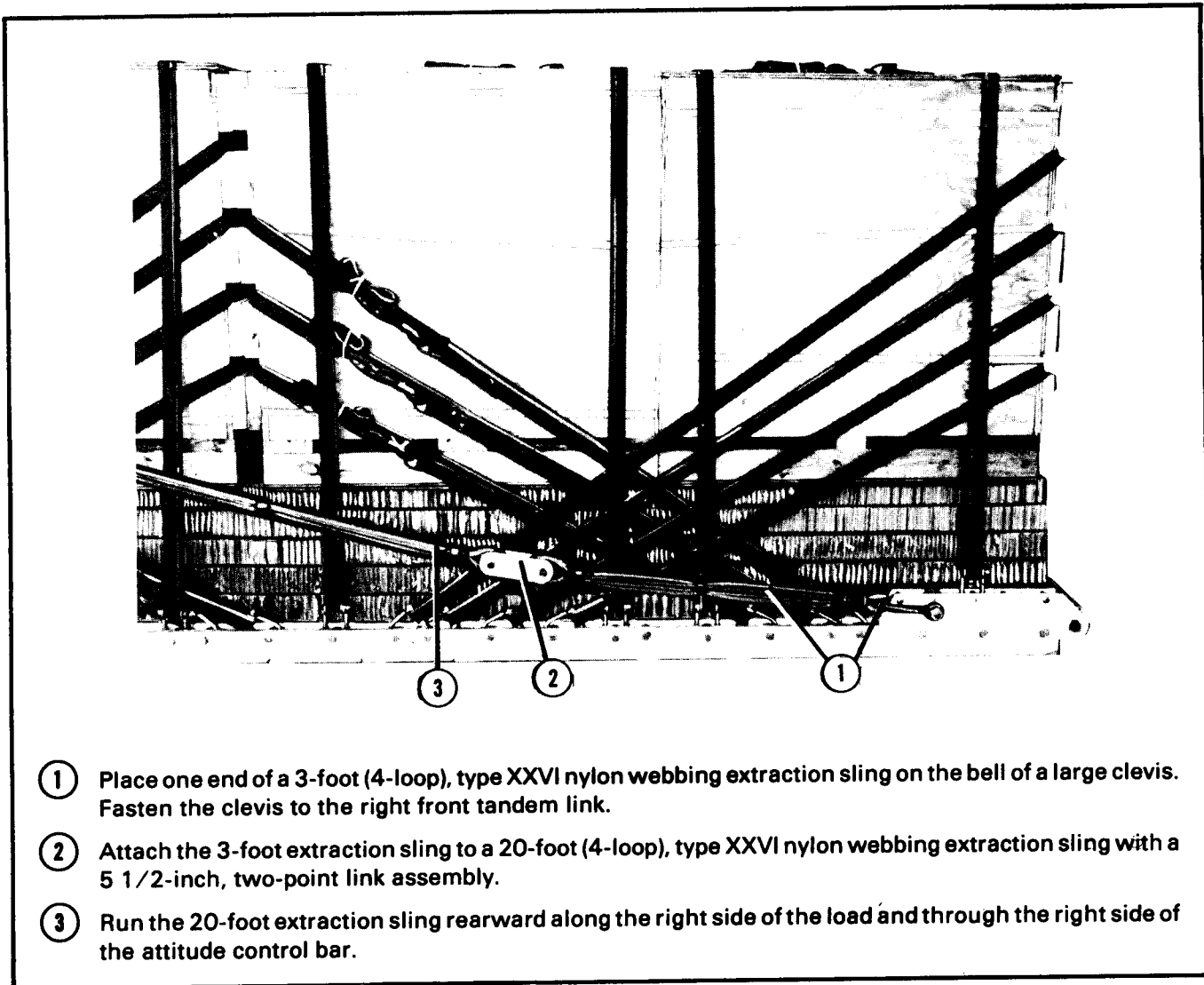
Figure 2-20. Extraction system installed
