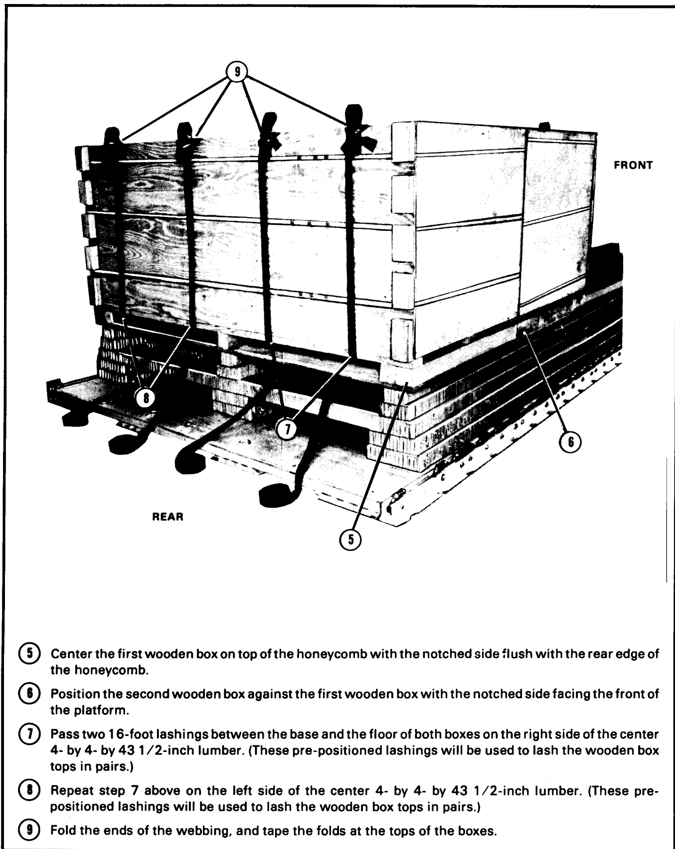
Figure 3-4. Wooden boxes positioned and lashed (continued)
