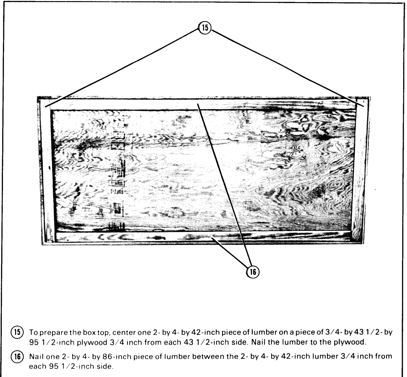
Figure 2-4. Wooden box prepared (continued)
