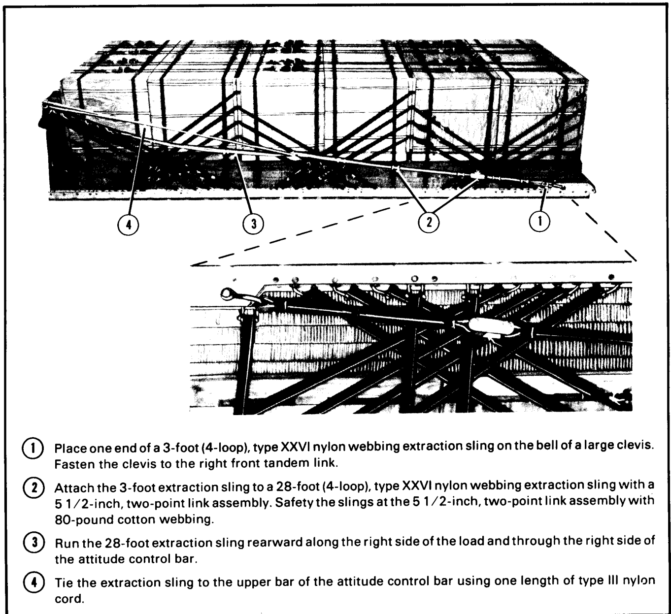
Figure 3-8. Extraction system installed
