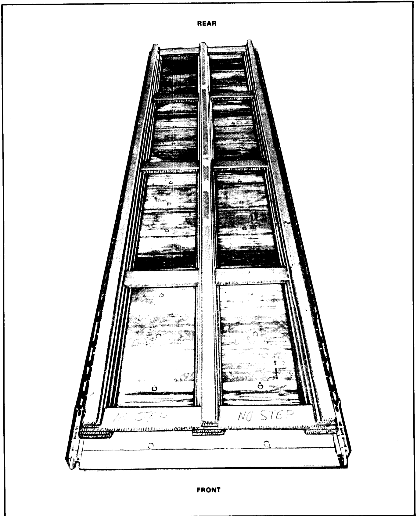
Figure 4-3. Front view of honeycomb layers placed on platform
