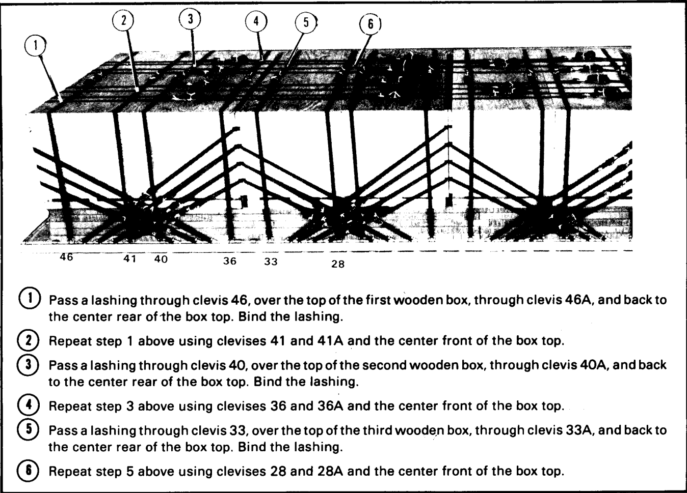
Figure 4-6. Vertical lashings positioned and fastened
