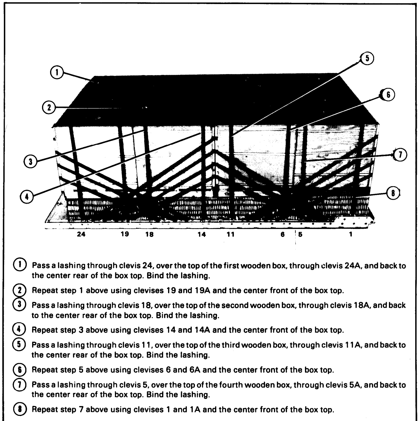
Figure 2-18. Vertical lashings positioned and fastened
