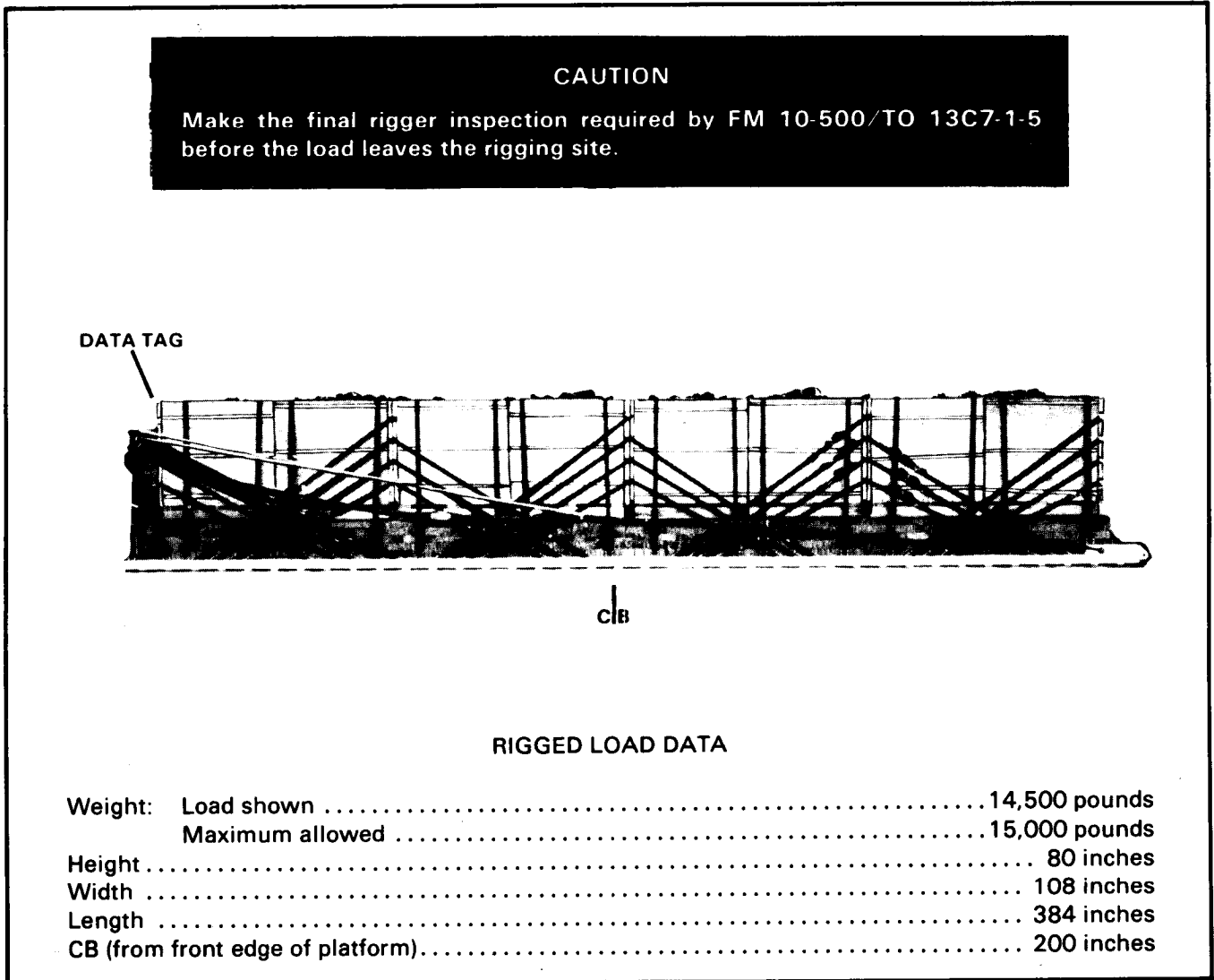
Figure 4-9. Whole blood rigged for LAPE airdrop on a type V airdrop platform
