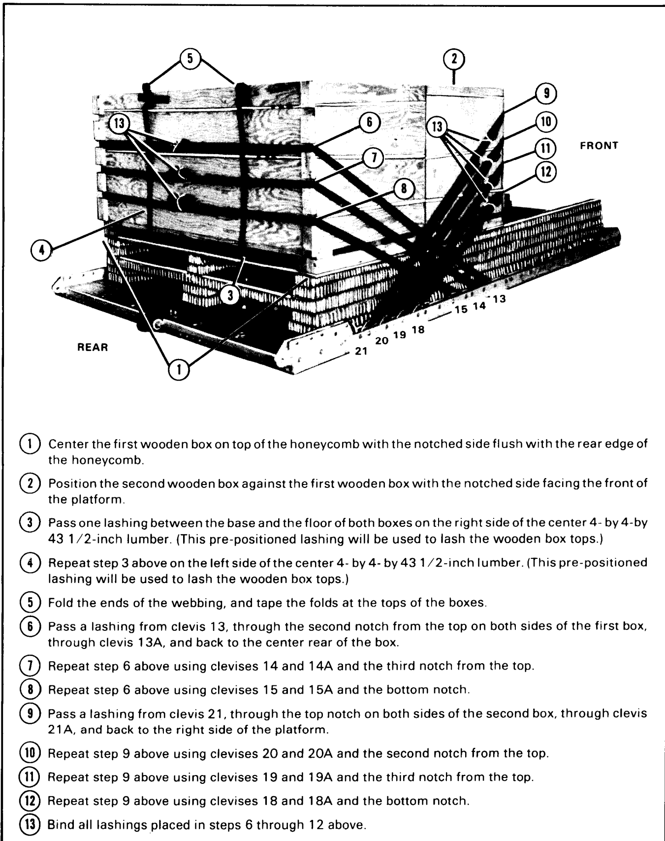
Figure 2-5. Wooden boxes positioned and lashed
