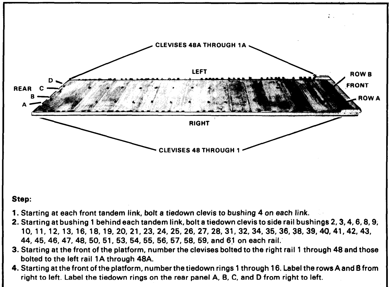
Figure 4-1. Platform prepared
