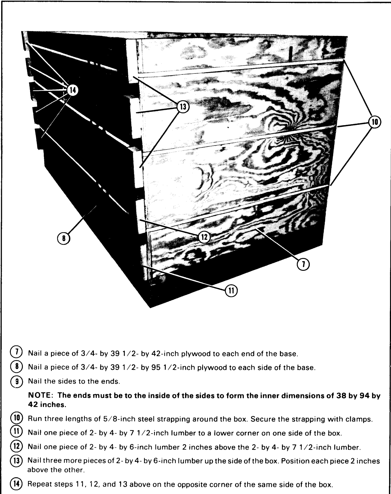
Figure 2-4. Wooden box prepared (continued)
