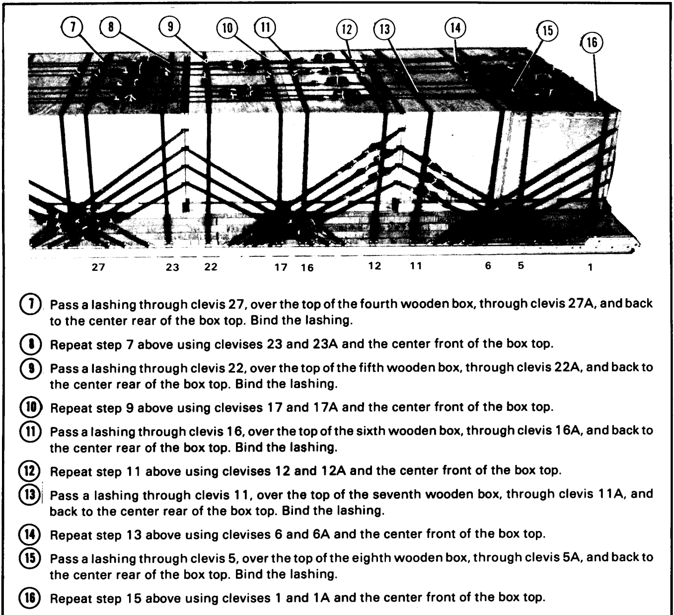
Figure 4-6. Vertical lashings positioned and fastened (continued)
