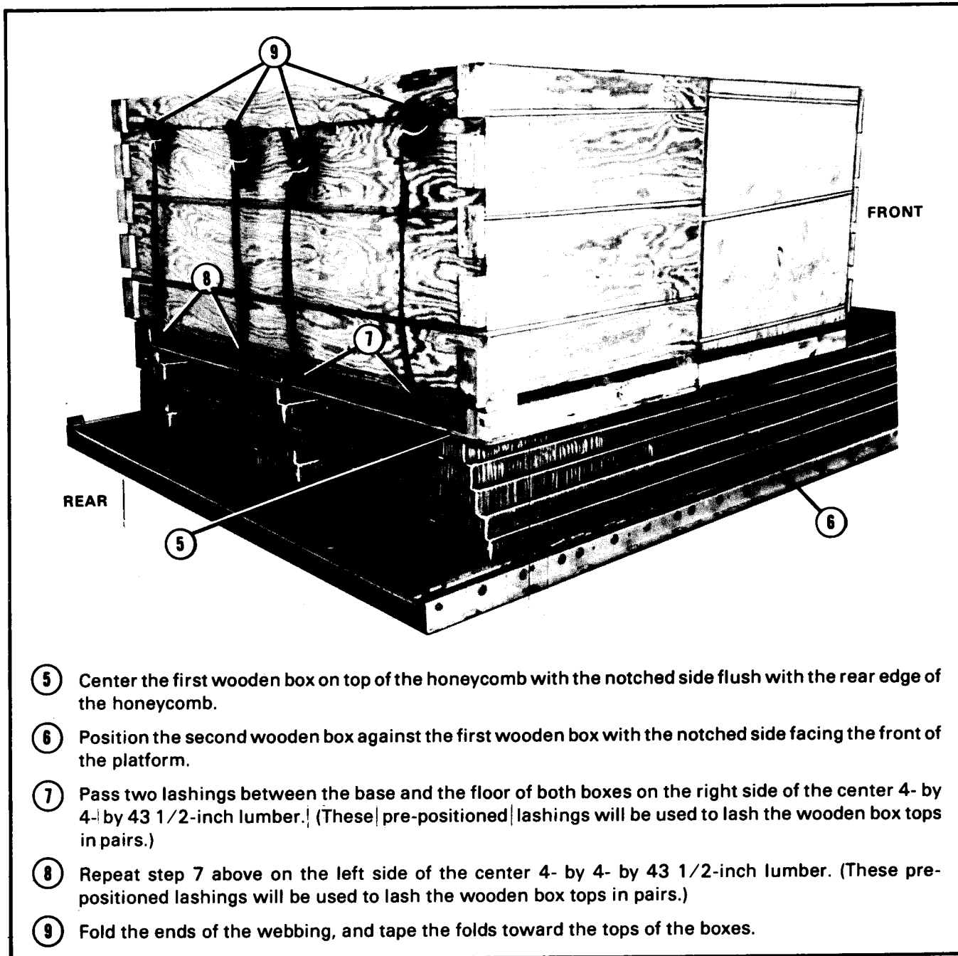
Figure 2-16. Wooden boxes positioned and lashed (continued)
