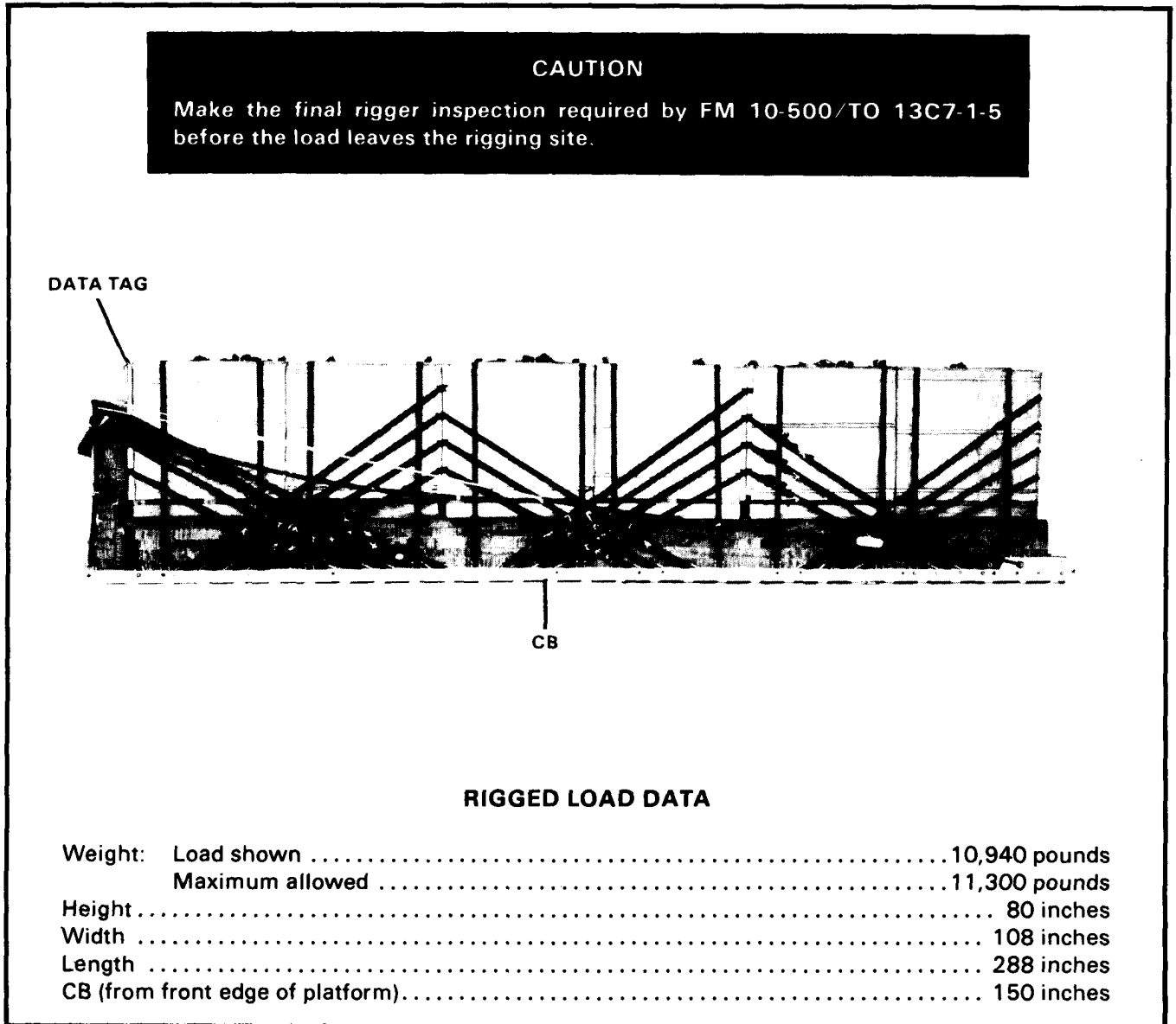
Figure 3-9. Whole blood rigged for LAPE airdrop on a type V airdrop platform
