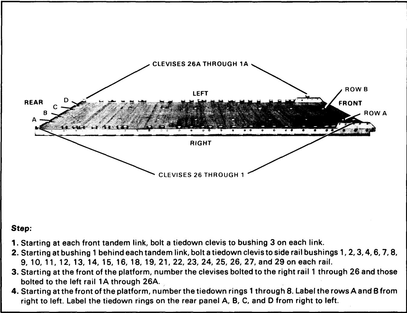
Figure 2-15. Platform prepared
