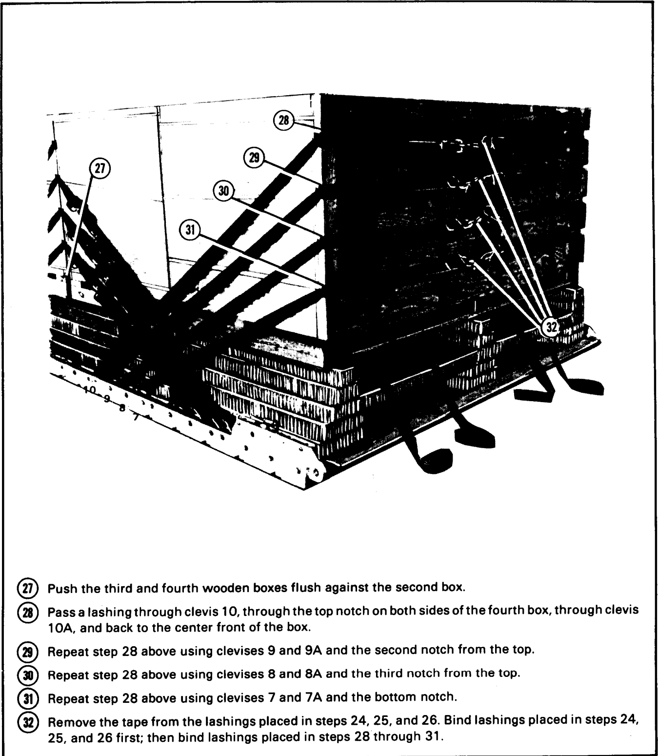
Figure 2-16. Wooden boxes positioned and lashed (continued)
