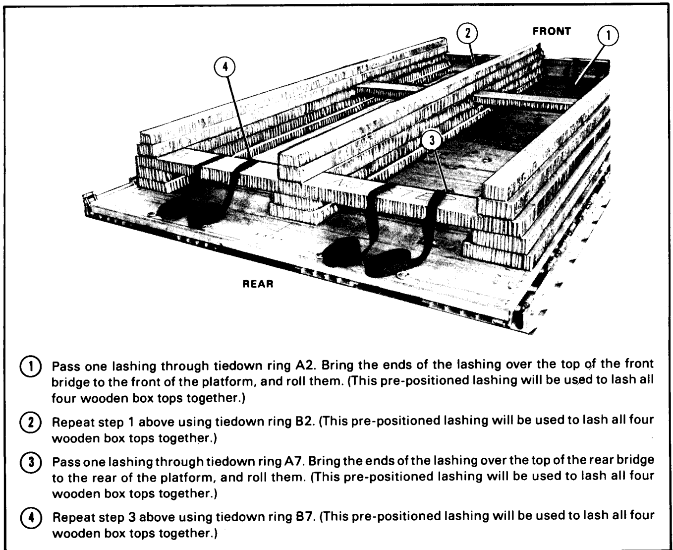
Figure 2-16. Wooden boxes positioned and lashed
