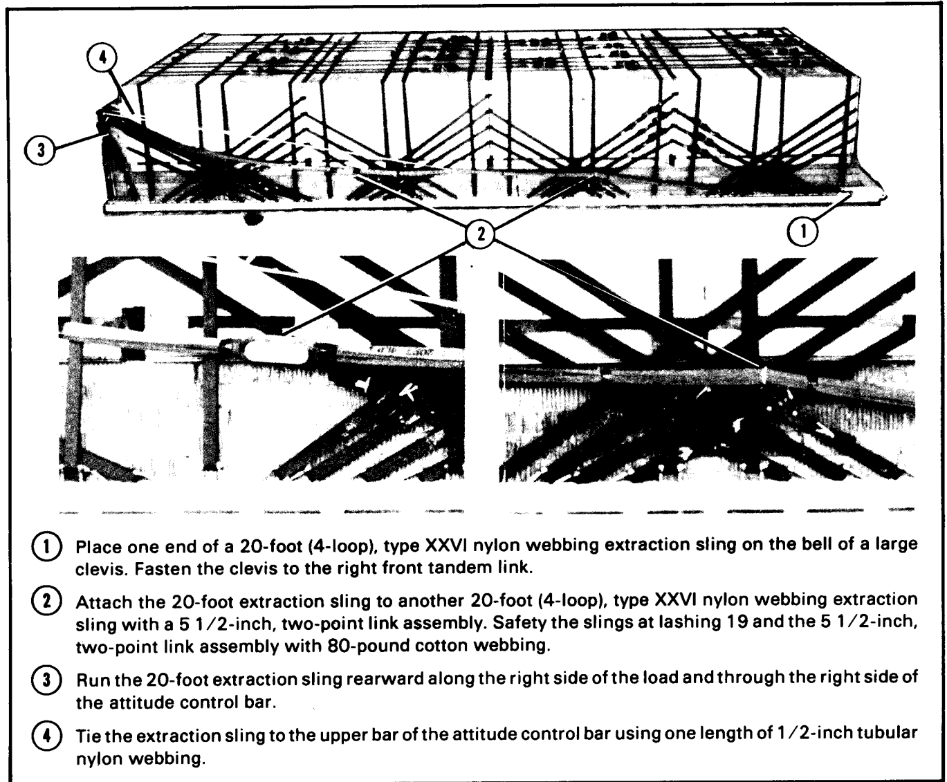
Figure 4-8. Extraction system installed
