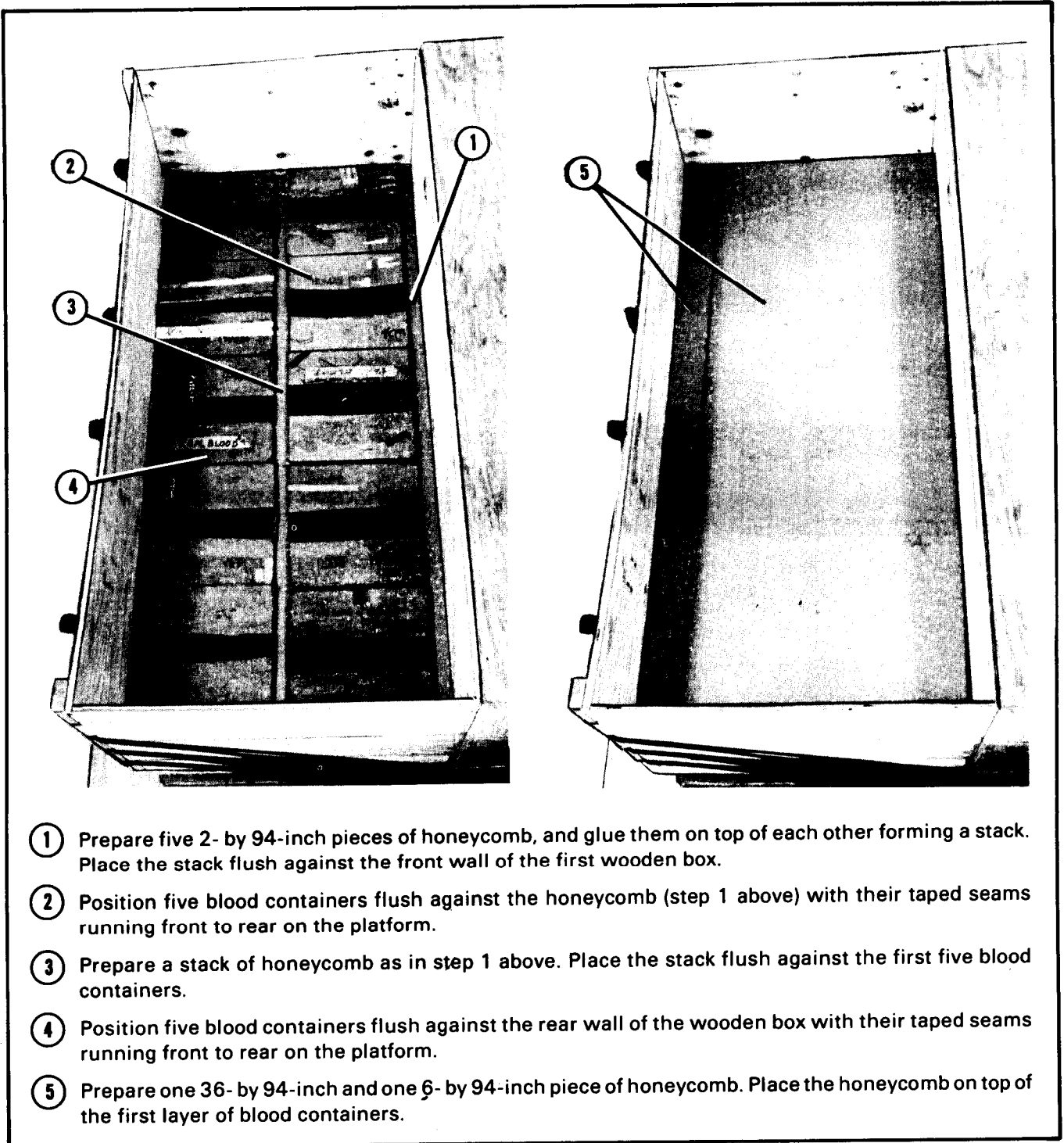
Figure 2-7. Wooden box filled with blood containers
