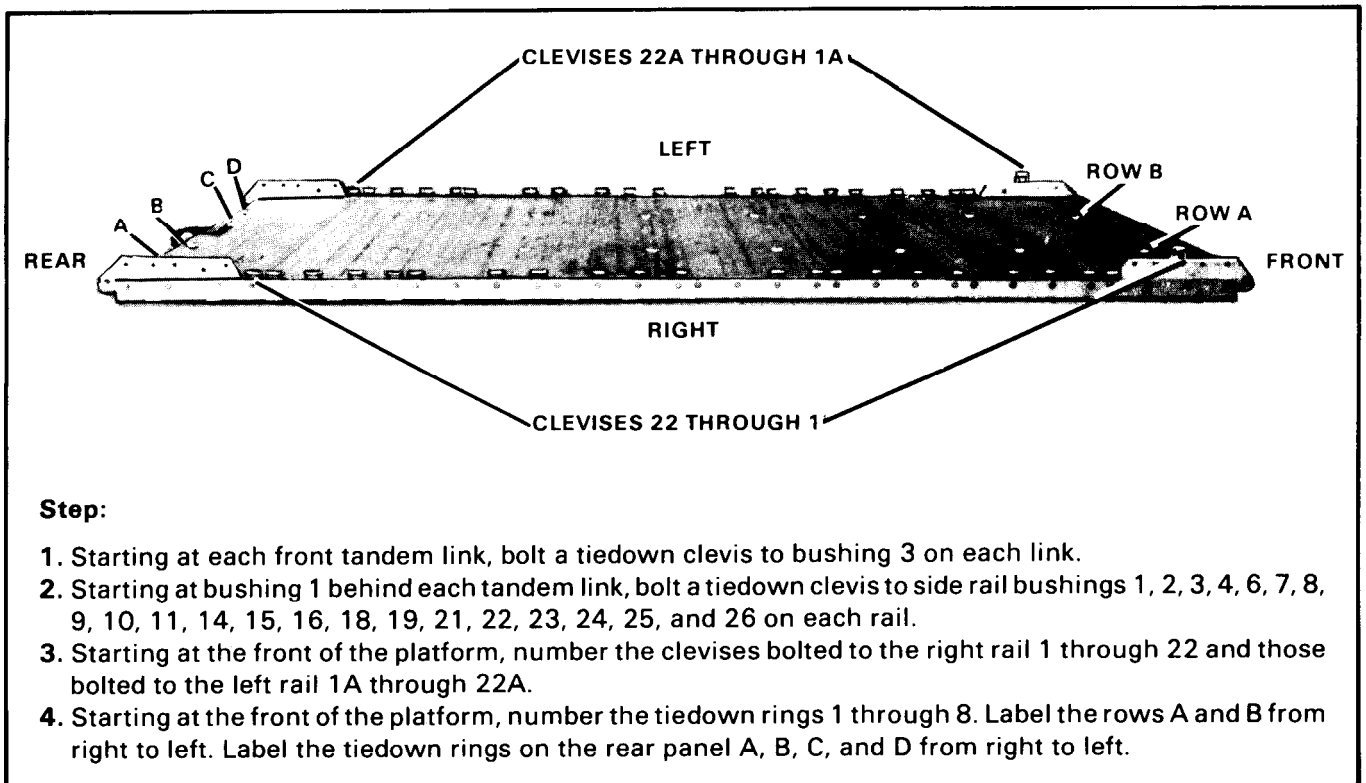
Figure 2-1. Platform prepared
