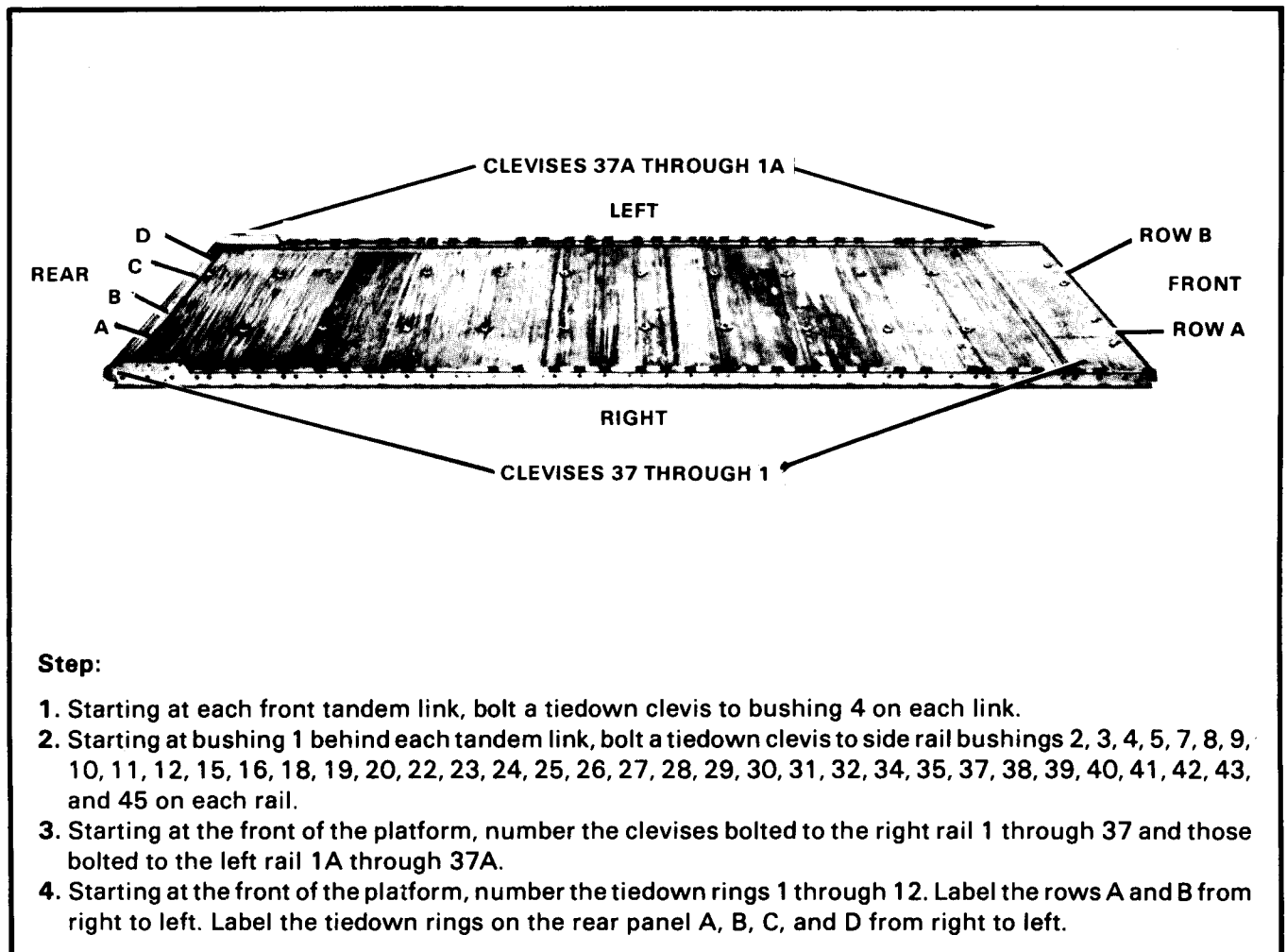
Figure 3-1. Platform prepared
