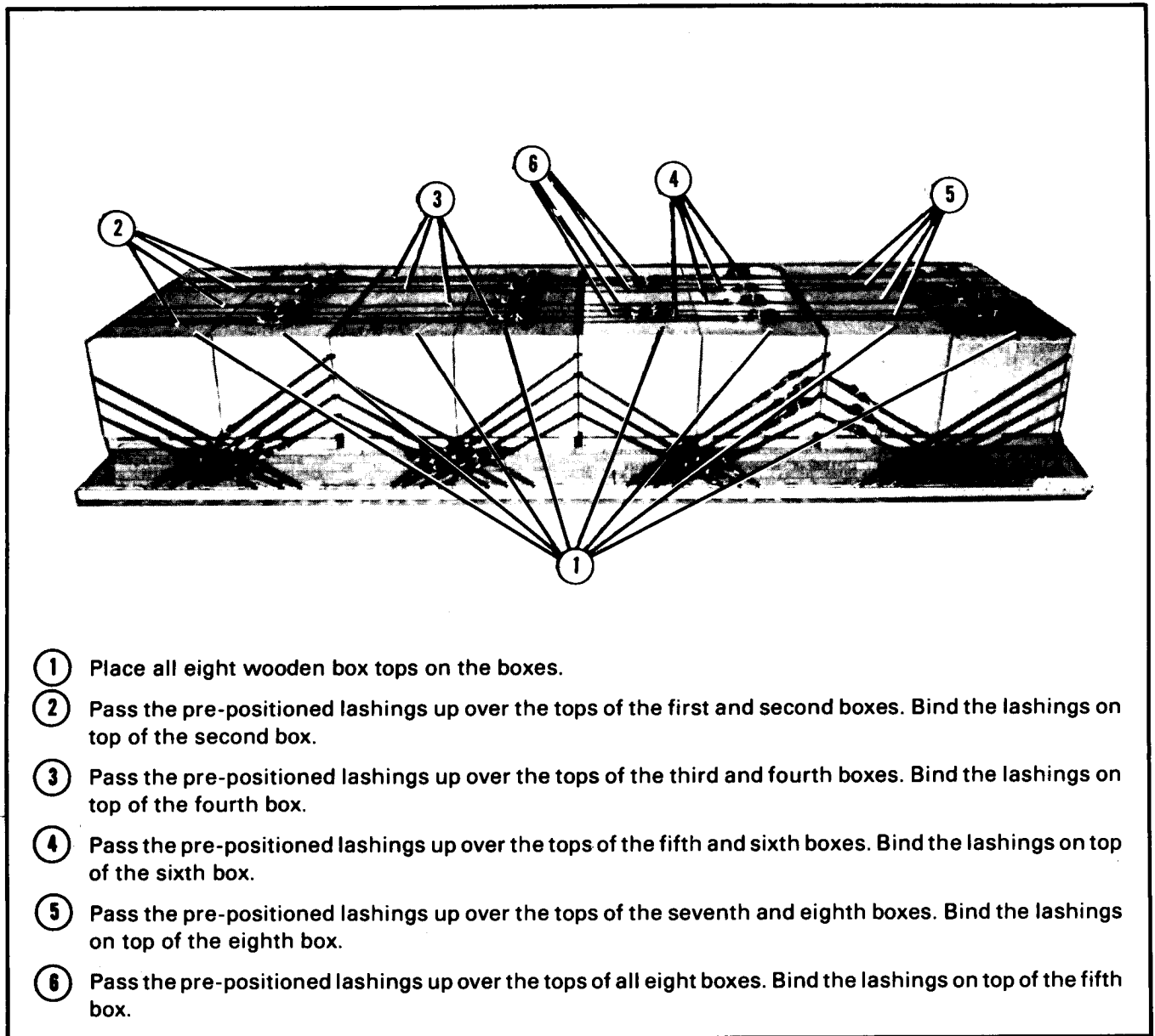
Figure 4-5. Wooden box tops positioned and lashed
