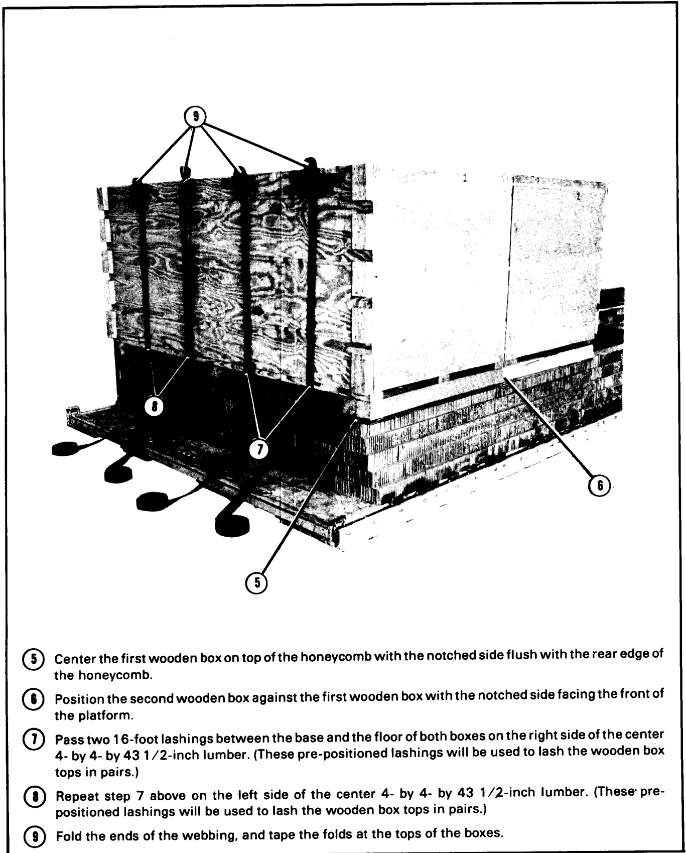
Figure 4-4. Wooden boxes positioned and lashed (continued)
