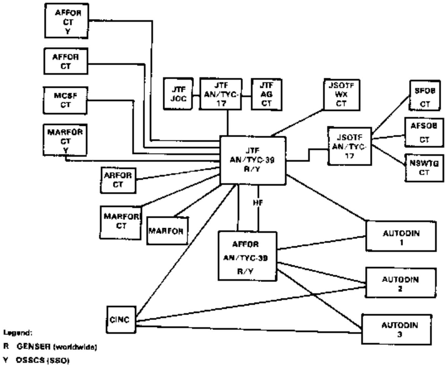
Figure 1-2. Joint message switching network at EAC.
