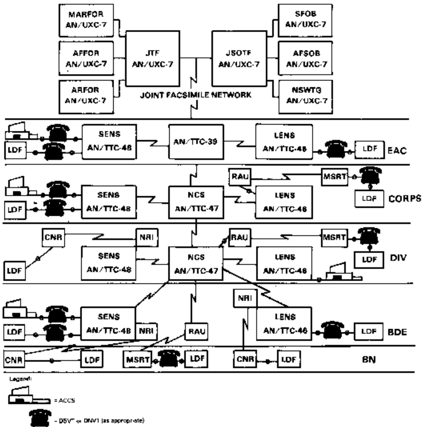
Figure 8-1. Informal TRTS architecture (circuit switched network).
