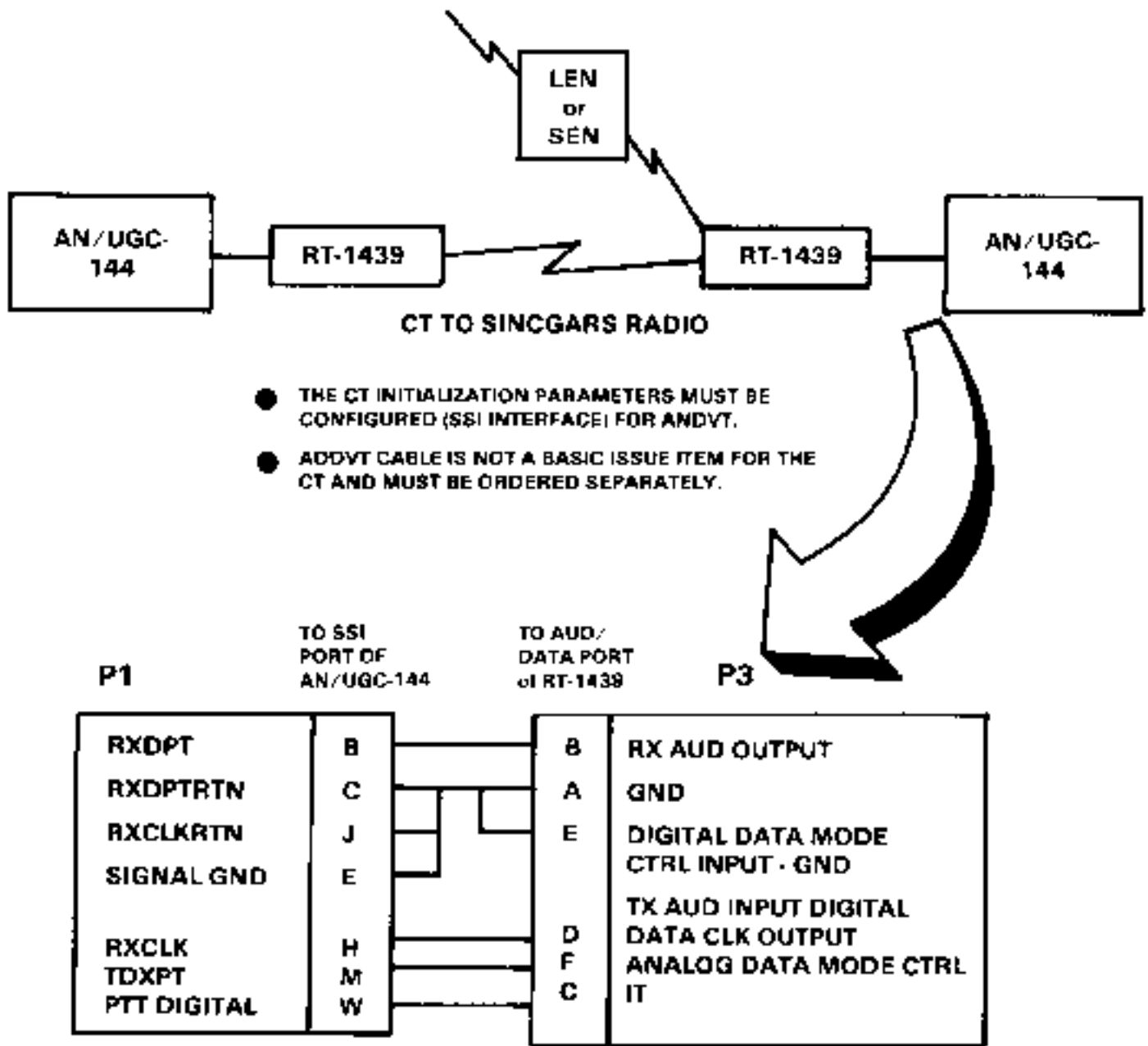
Figure 8-3. CT to SINGARS radio.
