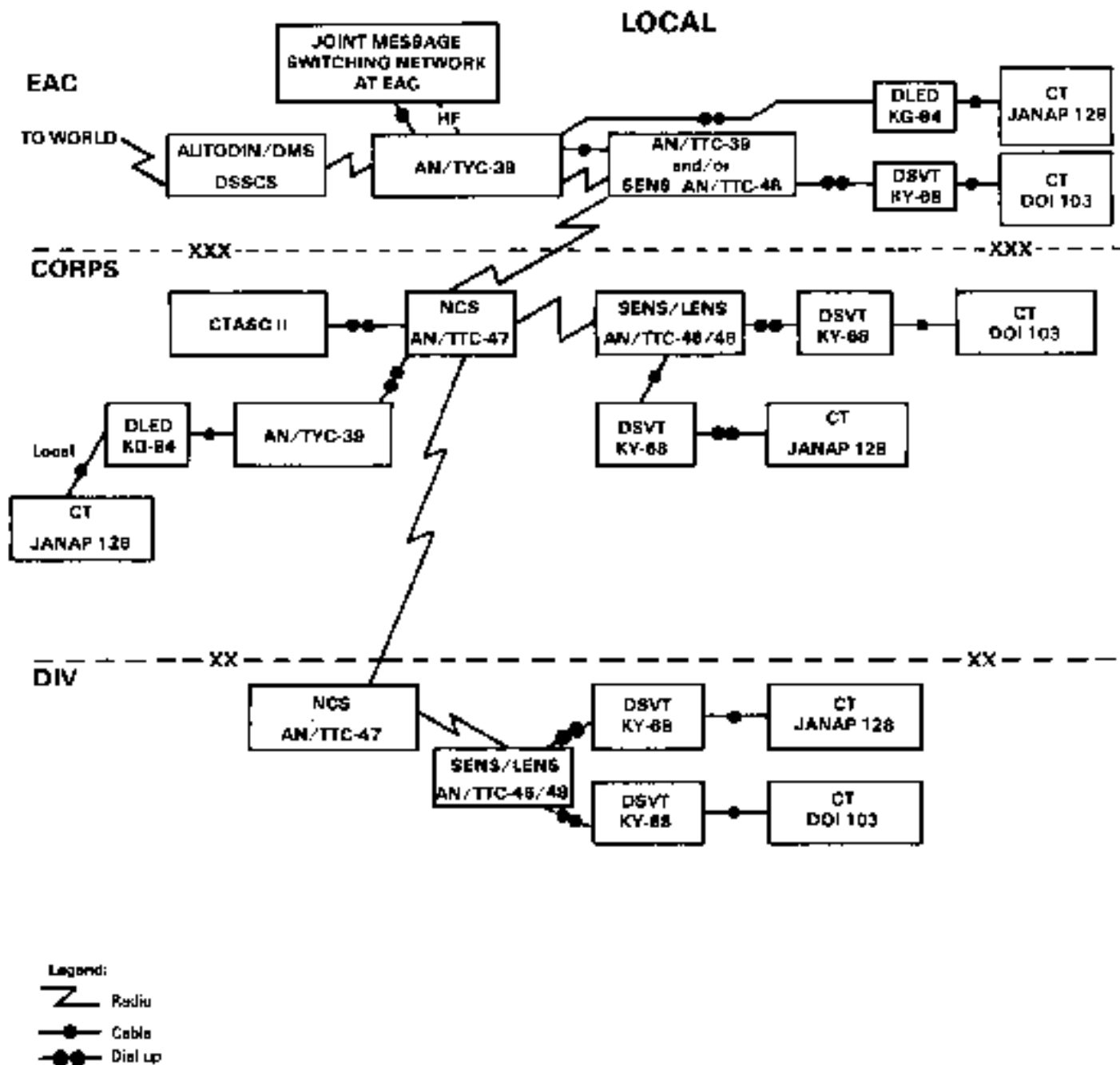
Figure 1-1. Formal TRTS architecture.
