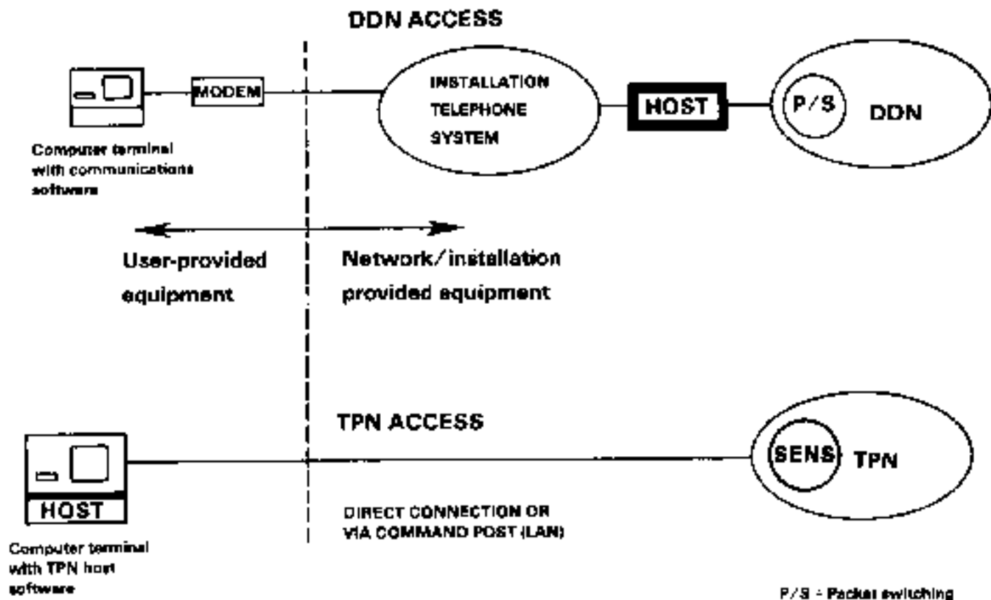
Figure 8-5. Comparison of DDN vs TPN access.
