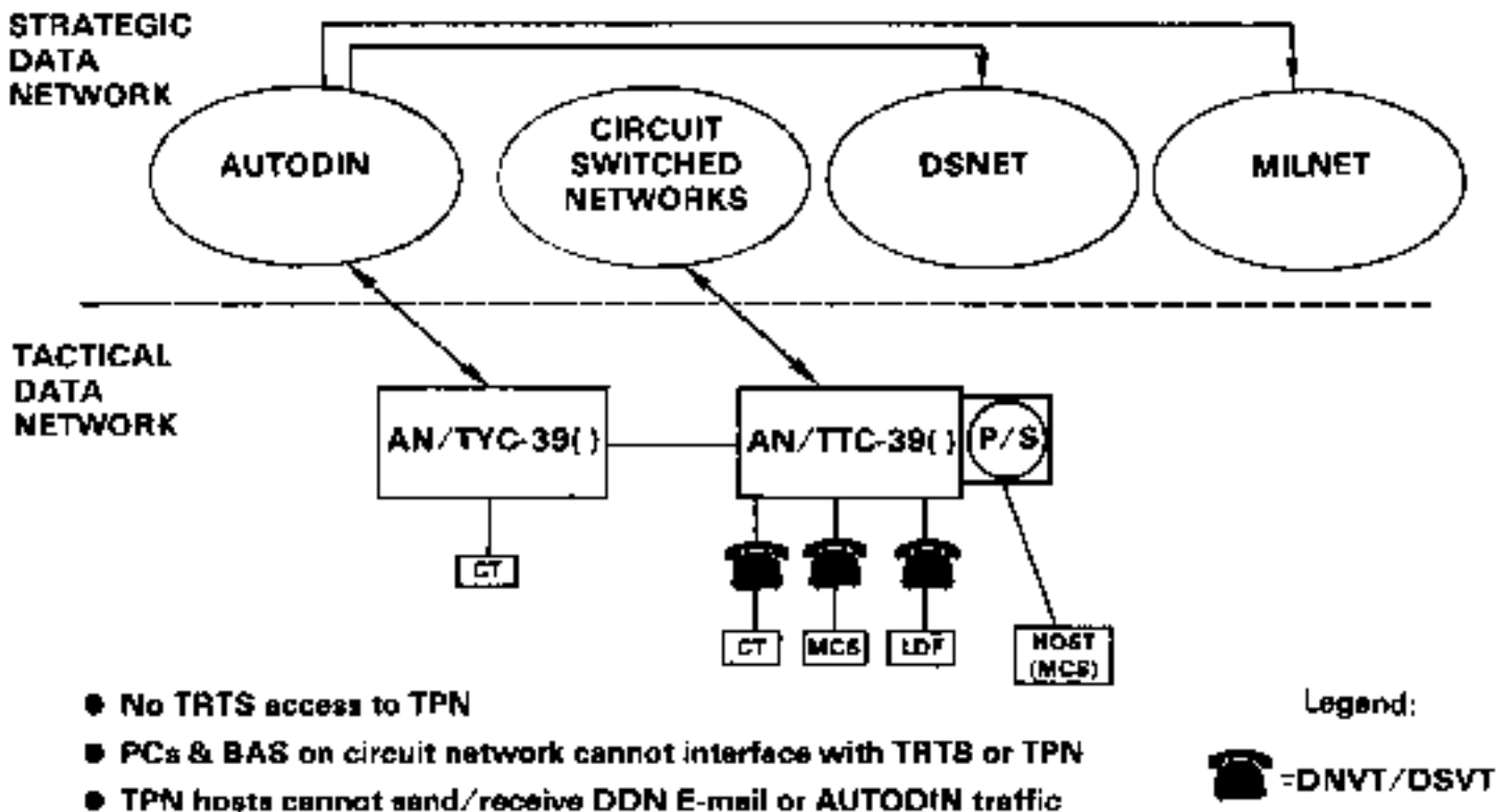
Figure 8-6. Network interconnectivity.
