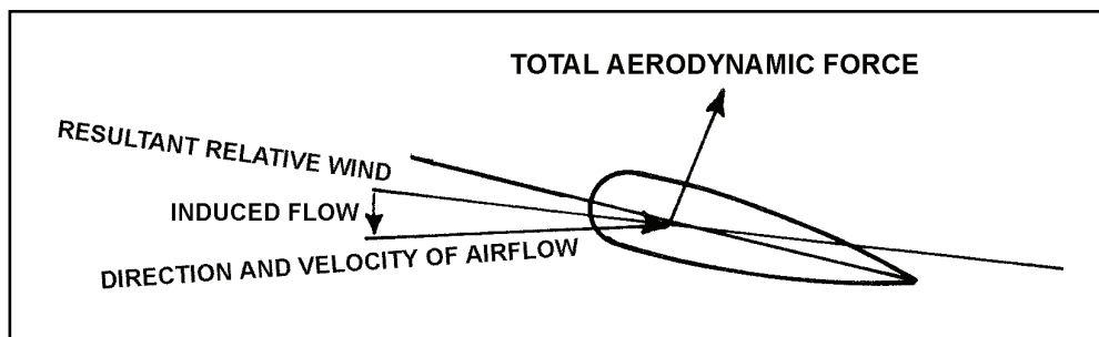
Figure 1-38. Total aerodynamic force
