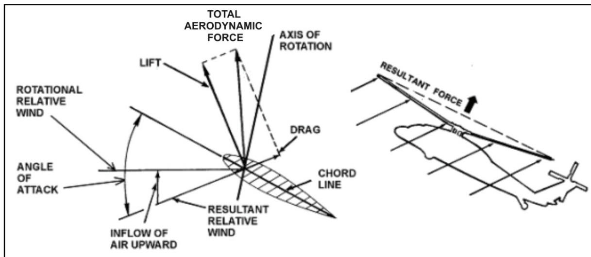
Figure 1-67. Autorotative deceleration
