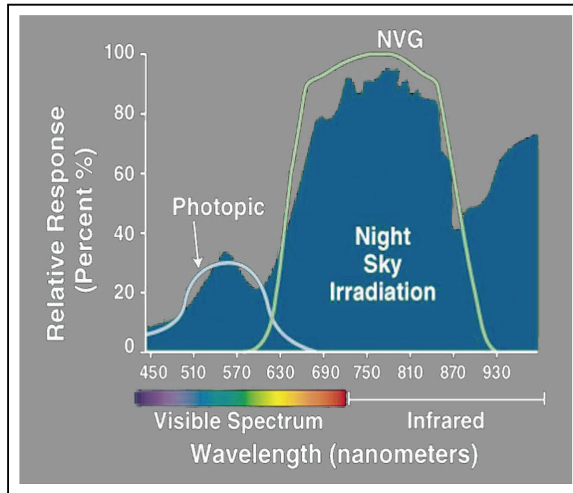
Figure 4-5. Electromagnetic Spectrum
