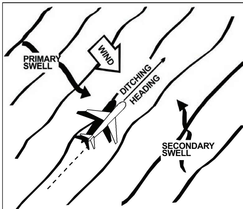
Figure 8-7. Single swell
