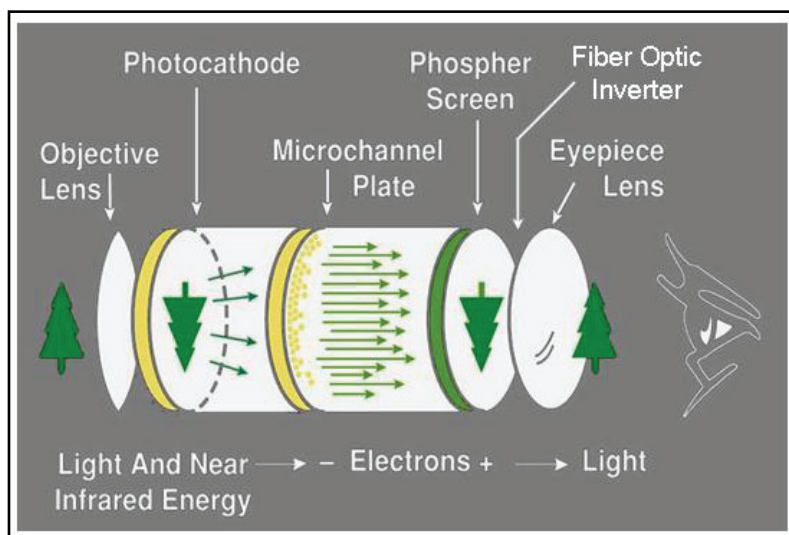
Figure 4-7. Image intensifier
