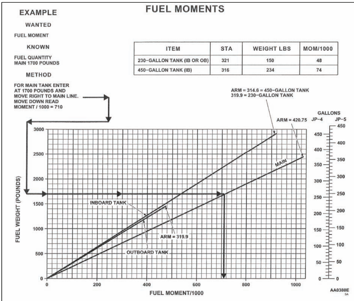
Figure 2-4. Fuel moments
