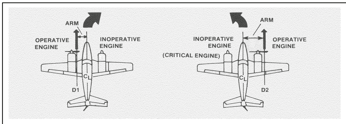
Figure 7-59. Forces created during single-engine operation
