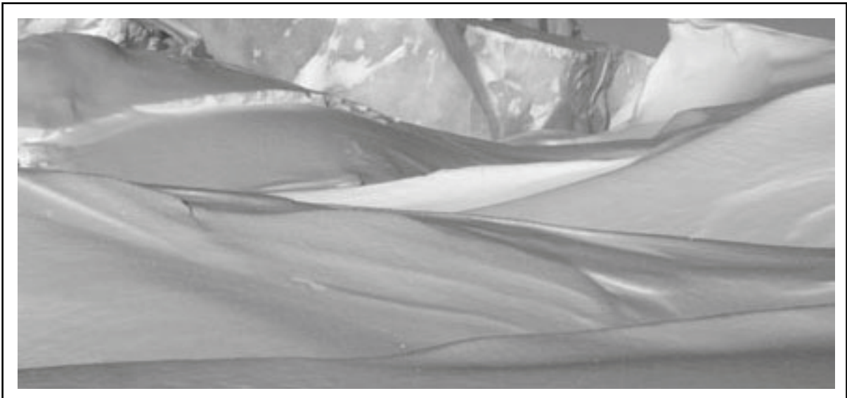
Figure 3-3. Depth perception
