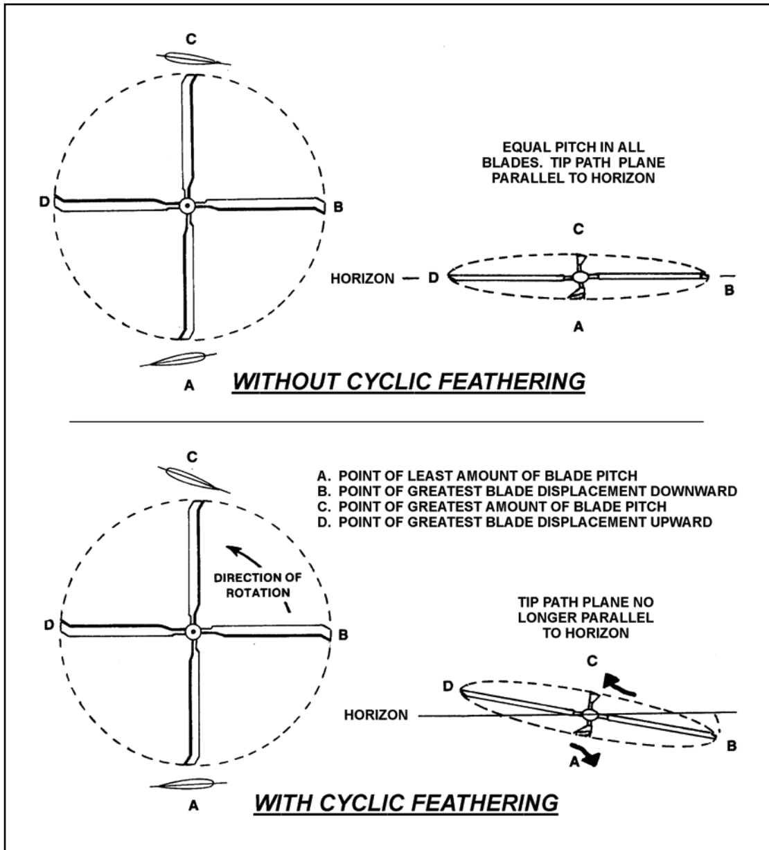
Figure 1-31. Cyclic feathering
