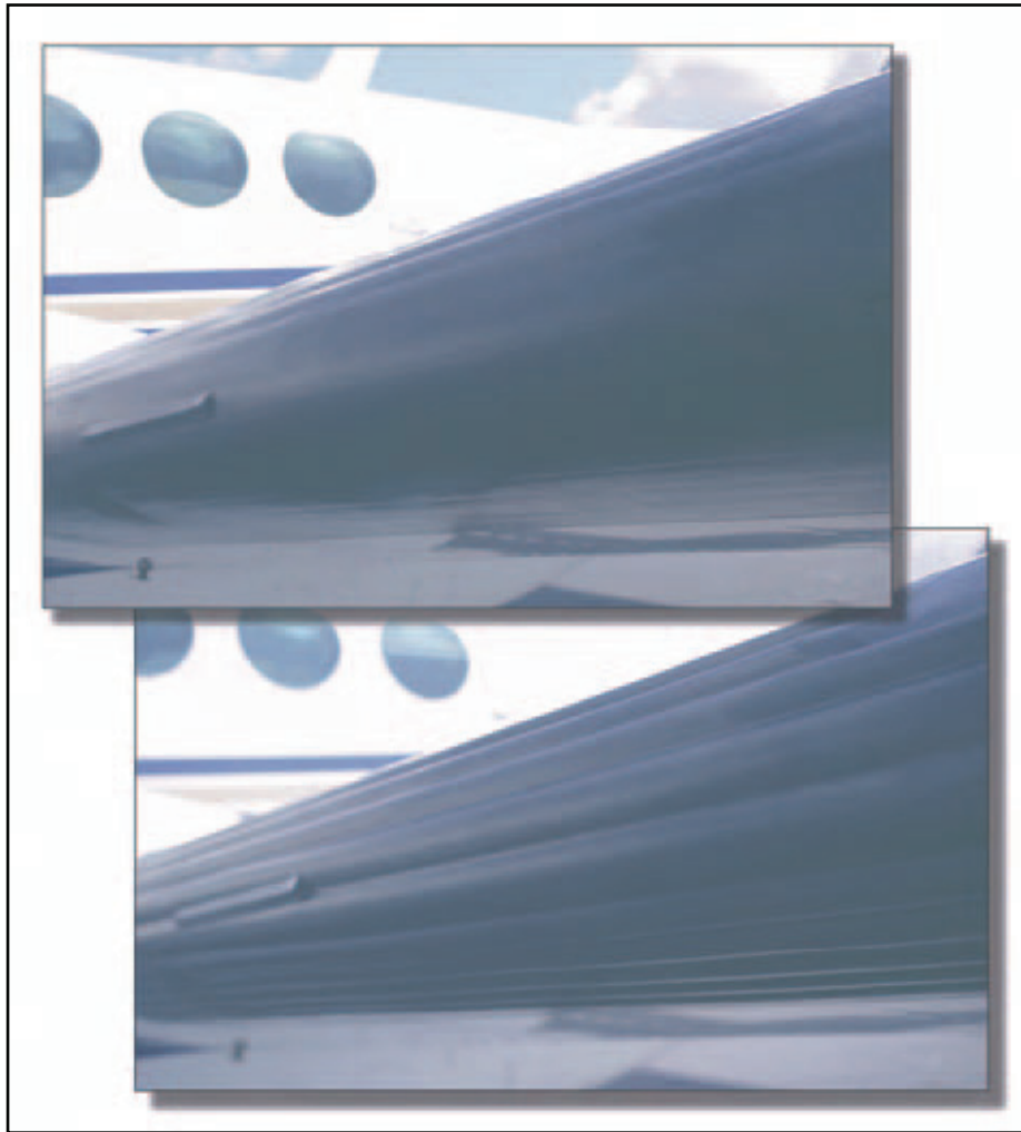
Figure 8-4. Pneumatic boots
