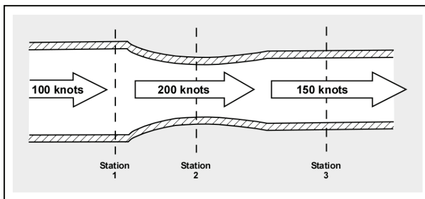
Figure 1-2. Venturi effect
