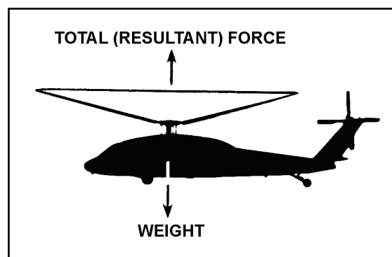
Figure 1-44. Balanced forces; hovering with no wind
