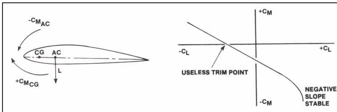
Figure 7-8. Positive longitudinal stability of a positive-cambered airfoil
