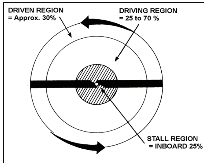
Figure 1-61. Blade regions in vertical autorotation descent
