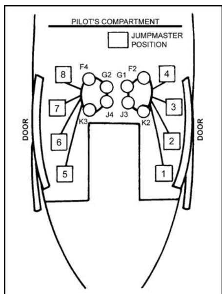
Figure 17-4. UH-1 seating configuration, expedient anchor line system.
