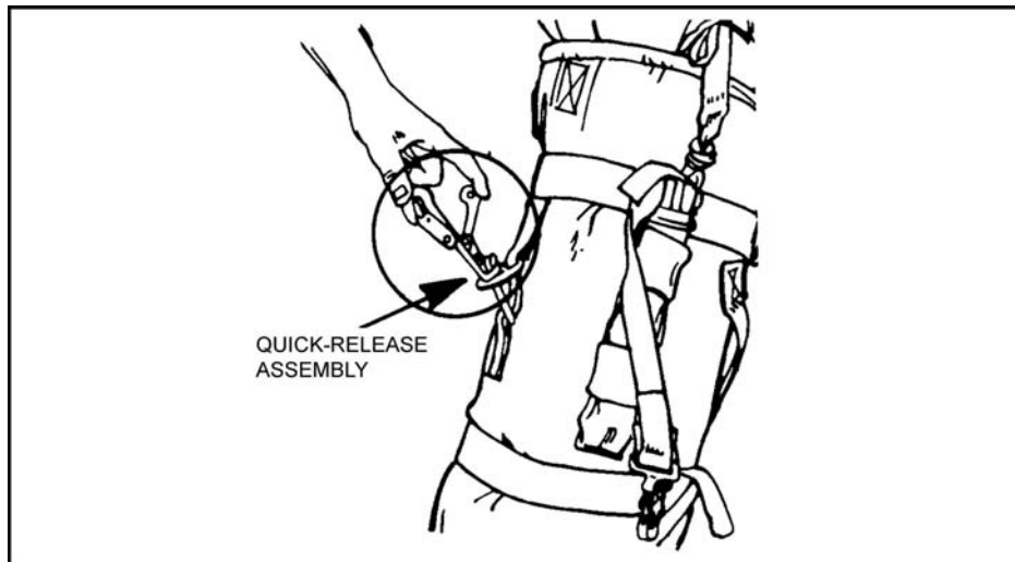
Figure 12-37. Quick-release assembly.
