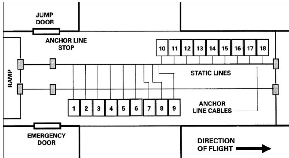
Figure 19-5. Seating configuration.
