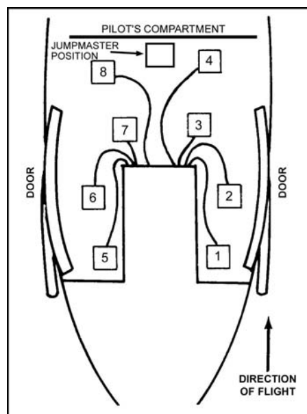
Figure 17-5. UH-1 seating configuration, overhead anchor line system.
