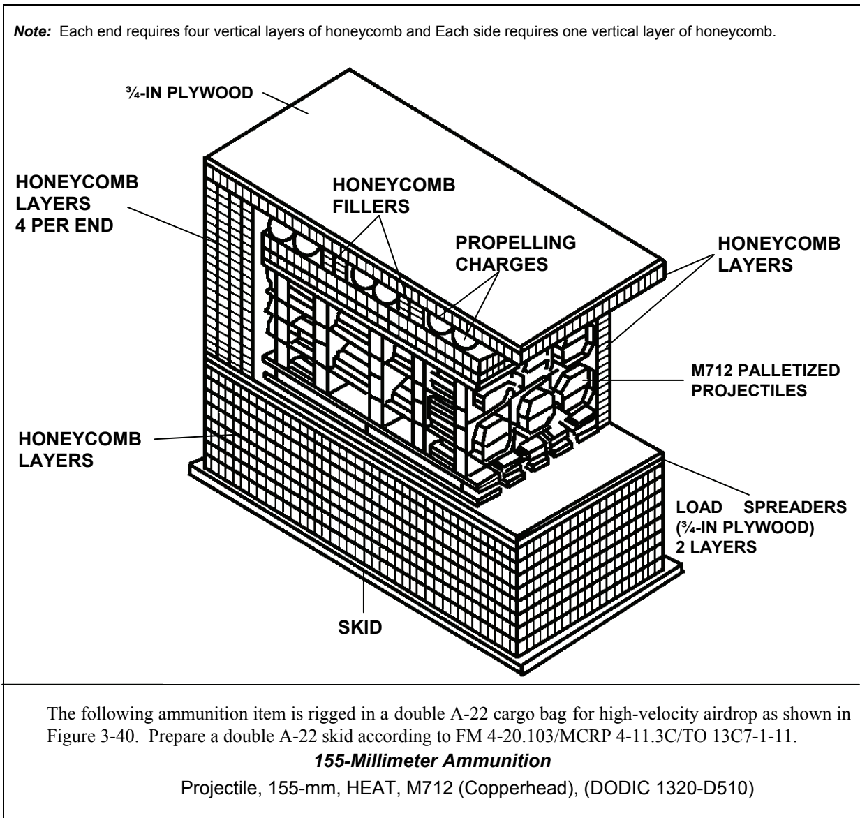
Figure 3-40. Ammunition Layout in a Double A-22 Cargo Bag for High-Velocity Airdrop
