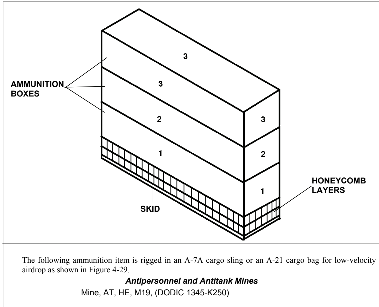
Figure 4-29. Ammunition Layout in an A-7A Cargo Sling or an A-21 Cargo Bag for Low-Velocity Airdrop
