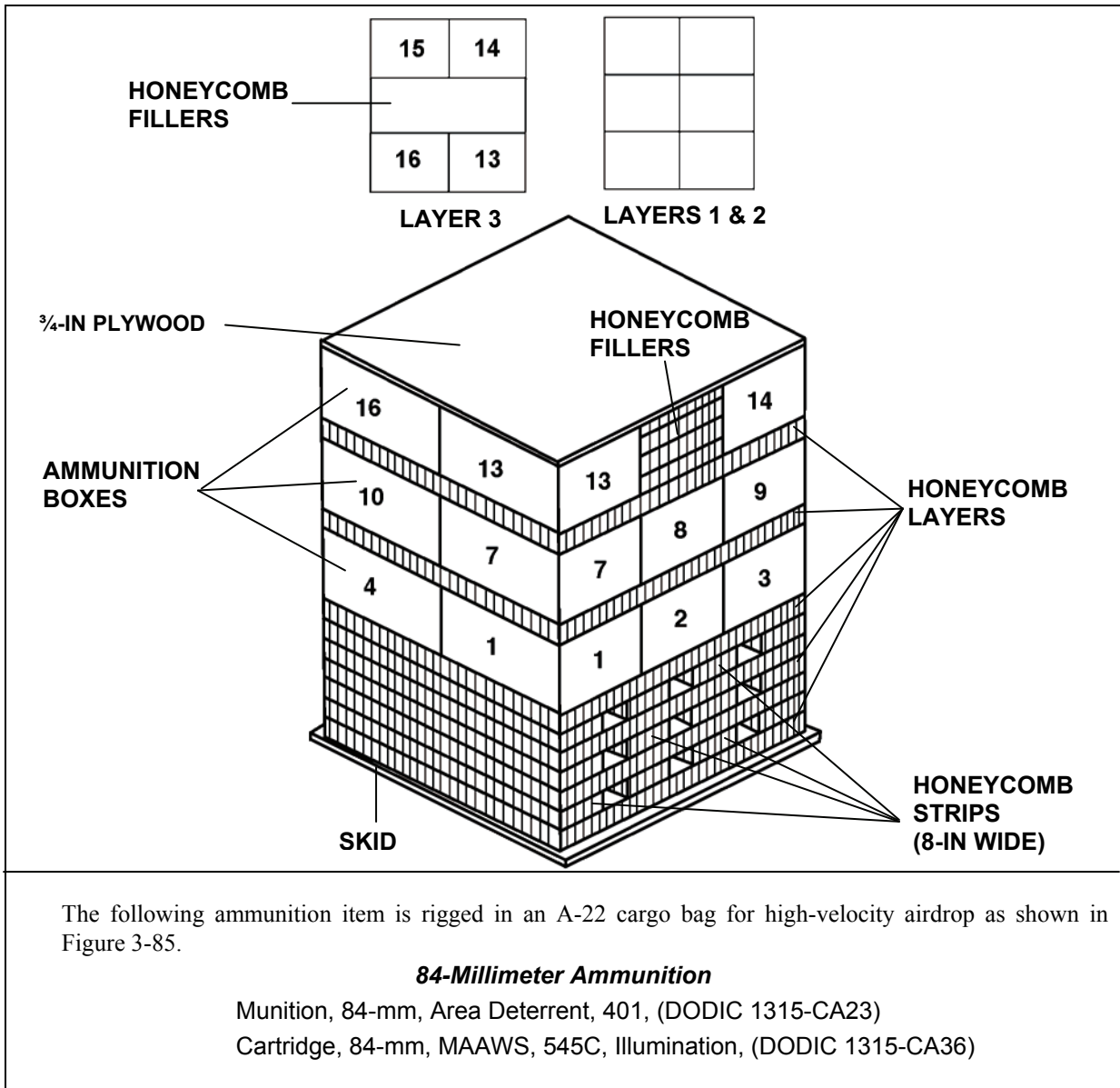
Figure 3-85. Ammunition Layout in an A-22 Cargo Bag for High-Velocity Airdrop
