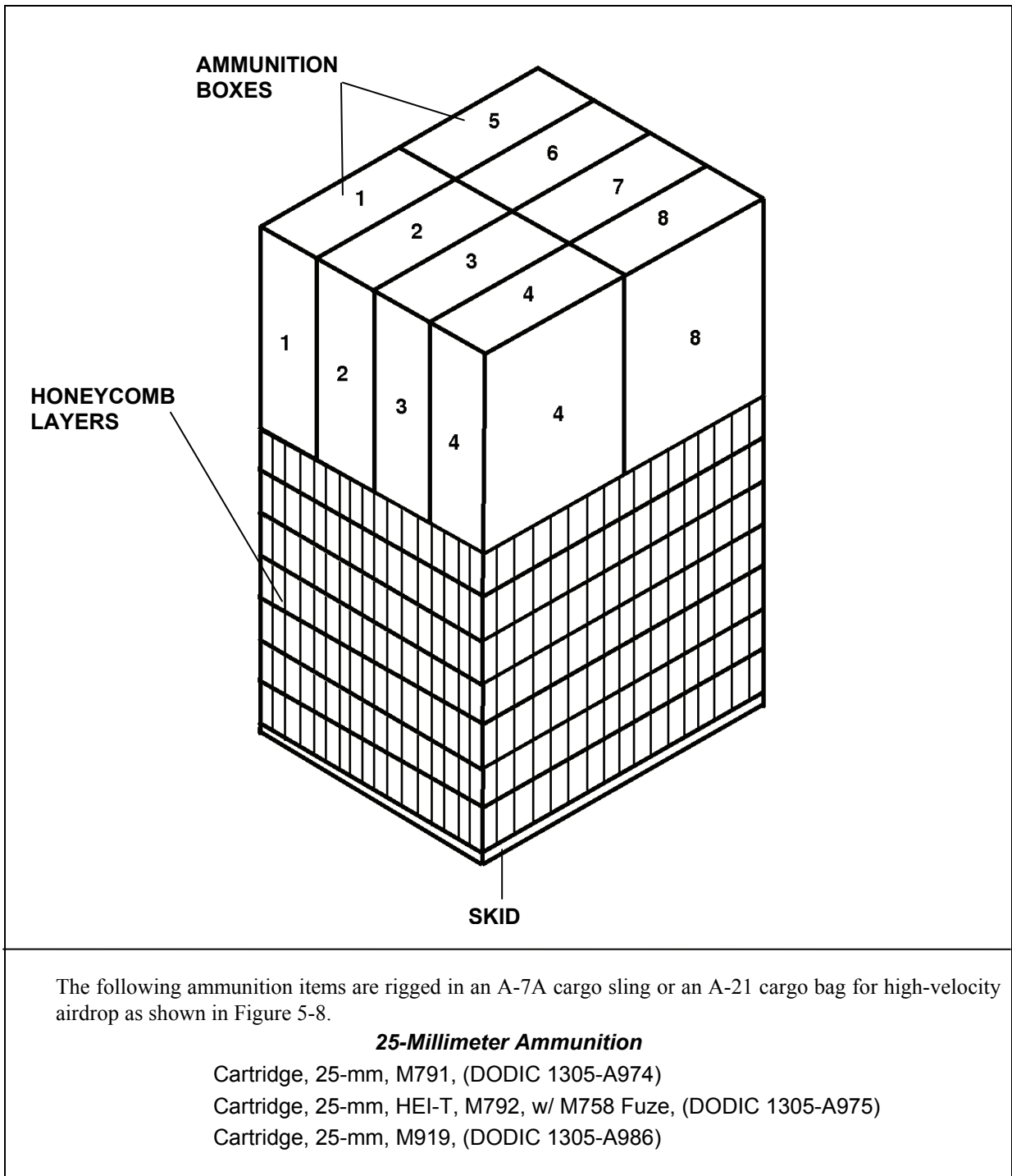
Figure 5-8. Ammunition Layout in an A-7A Cargo Sling or an A-21 Cargo Bag for High-Velocity Airdrop
