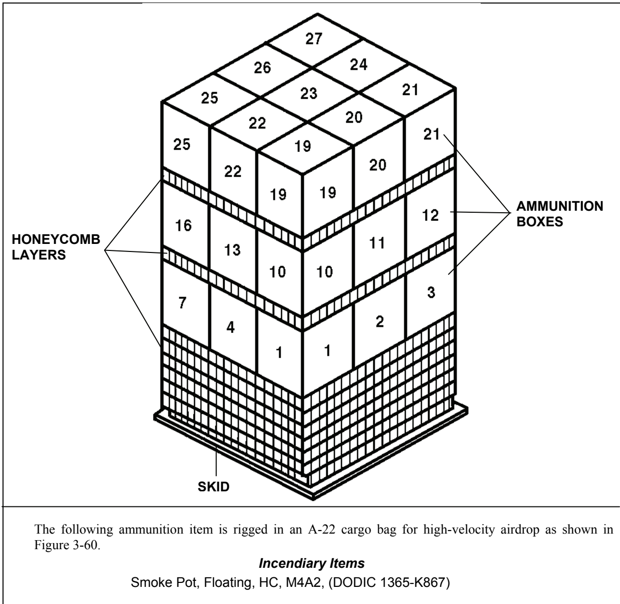
Figure 3-60. Ammunition Layout in an A-22 Cargo Bag for High-Velocity Airdrop
