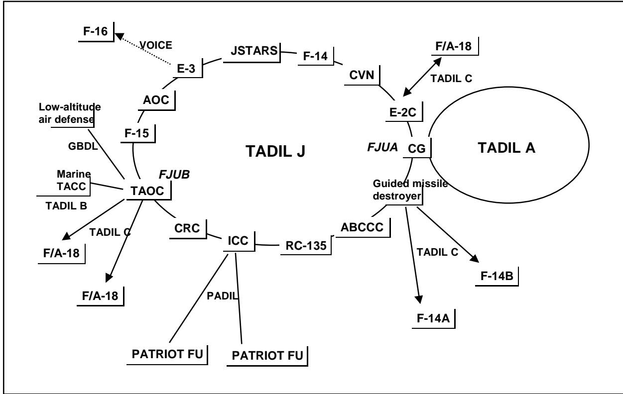
Figure II-4. Combined Theater Architecture
