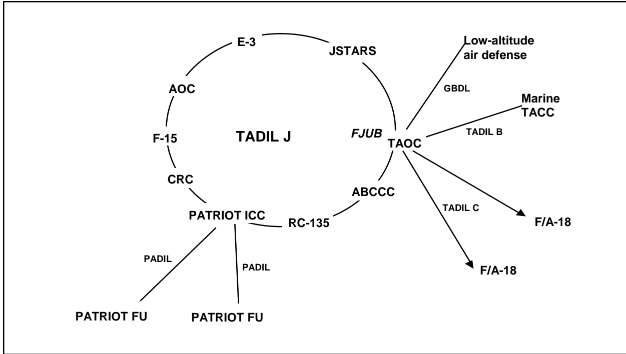
Figure II-3. Joint Architecture Ashore
