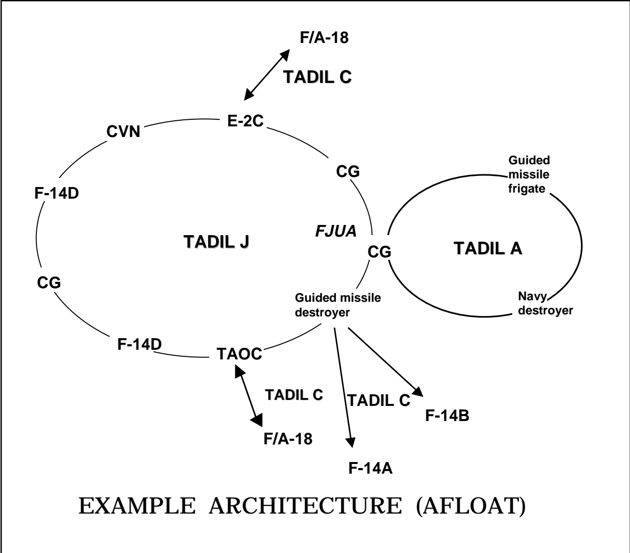
Figure II-2. Navy Architecture Afloat
