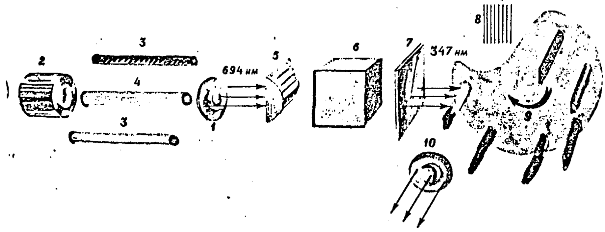
Fig. 2: diagram of an optical quantum generator "rainbow" (1) ruby laser resonator mirrors (2) Q-value modulator of ruby (Q-switch) (3) impulse flash lamps (4) ruby crystal (5) cylindrical lens (6) nonlinear crystal doubling the frequency of the radiation of the ruby laser (7) filter absorbing the constant frequency
