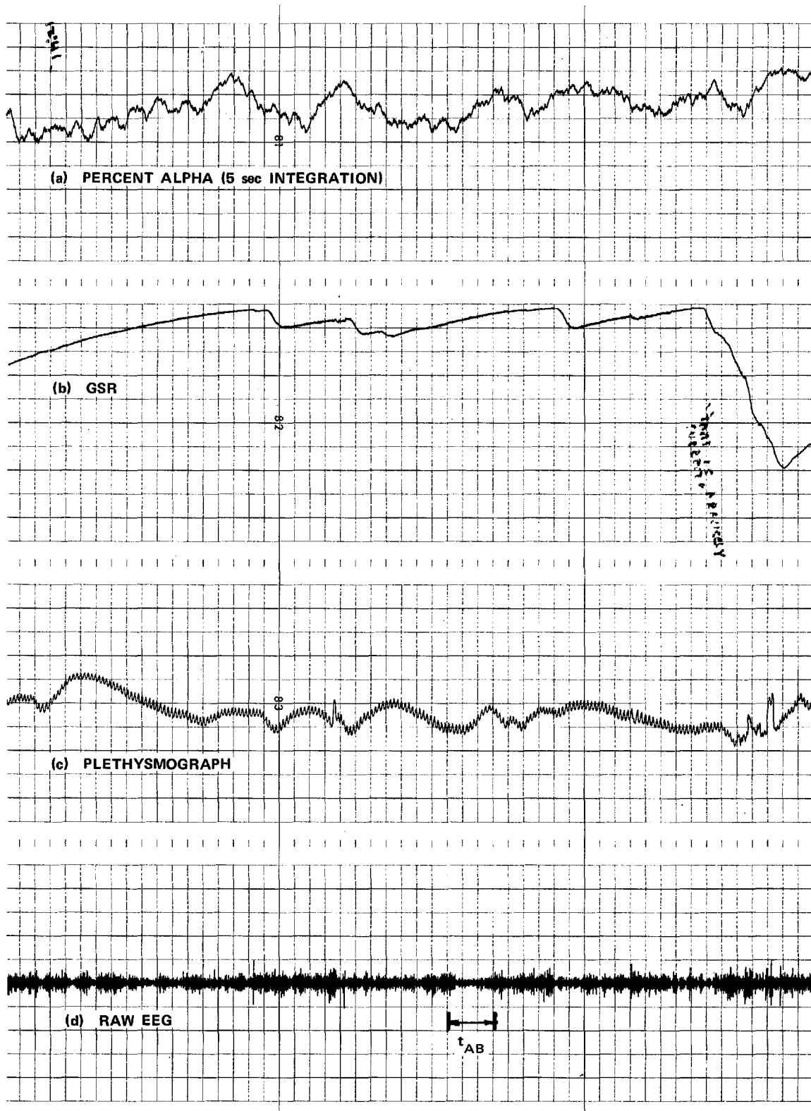
FIGURE 8 POLYGRAPH DATA
