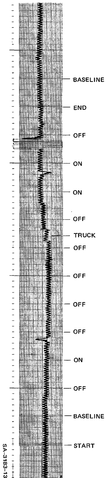
FIGURE 10 GRADIOMETER DATA
