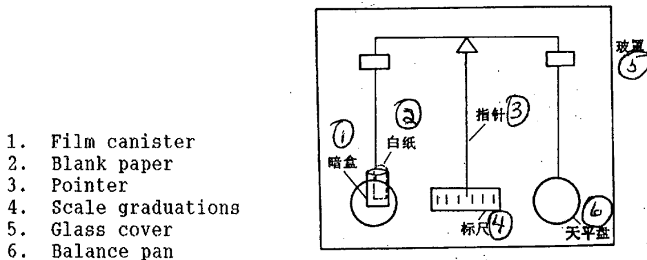
ILLUSTRATION ONE: DIAGRAM OF THE MECHANICAL BALANCE
