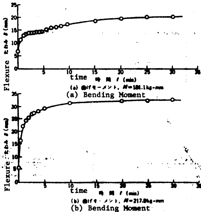
Diagram 9: Flexure-Time Relationship (Dynamic Creep Curve)
