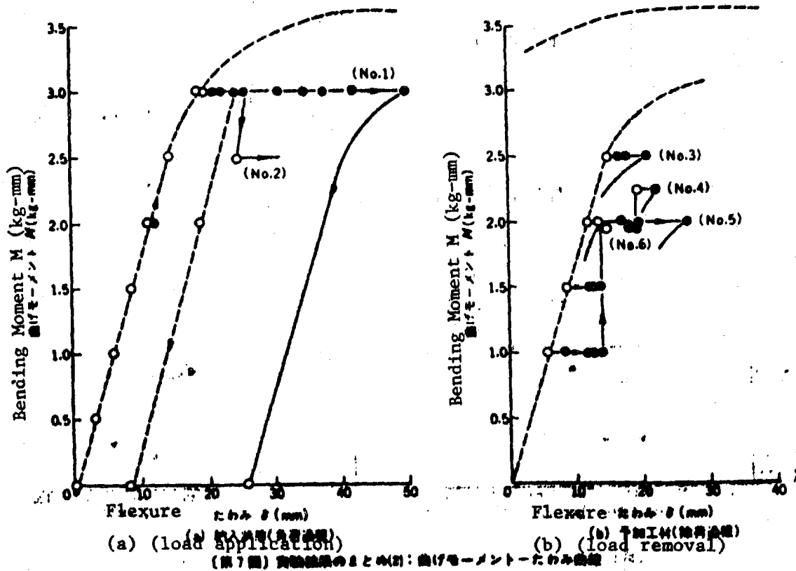
Diagram 7: Compiled Results (2): Bending Moment-Flexure Curve
