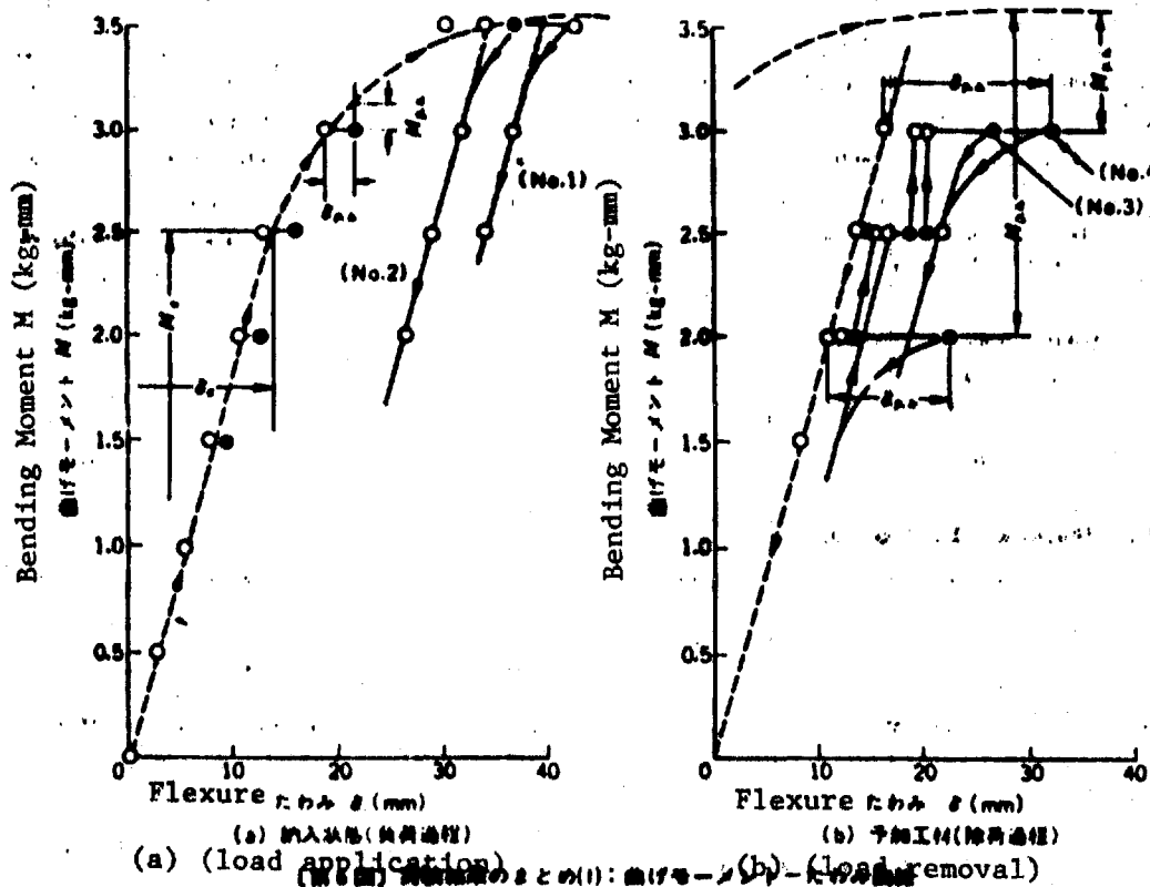
Diagram 6: Compiled results (1): Bending Moment- Flexure Curve
