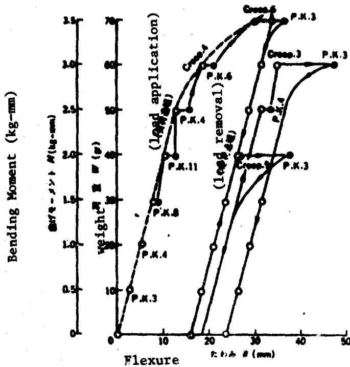
Diagram 3: Load (bending moment)-Flexure curve; example 1
