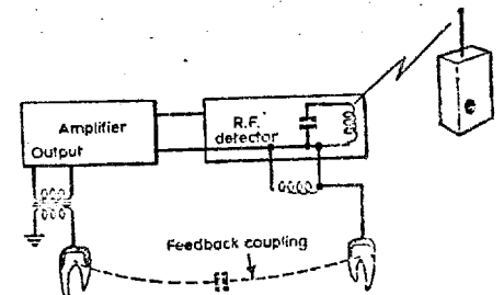
Figure 4 An alternative amplifier system uses two teeth. Based on
