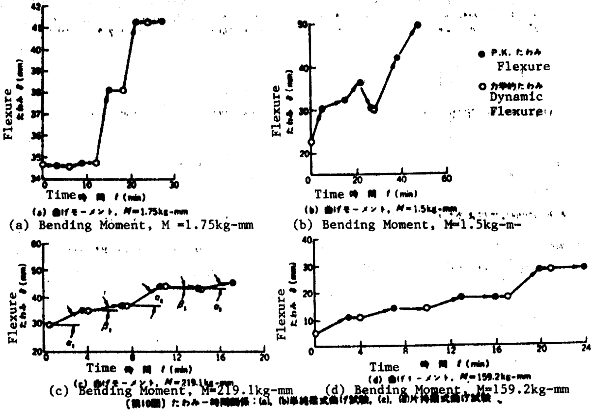
Diagram 10: The Flexure- Time Relationship. (a) and (b): simple beam structure bending test; (c) and (d) cantilever type bending test
