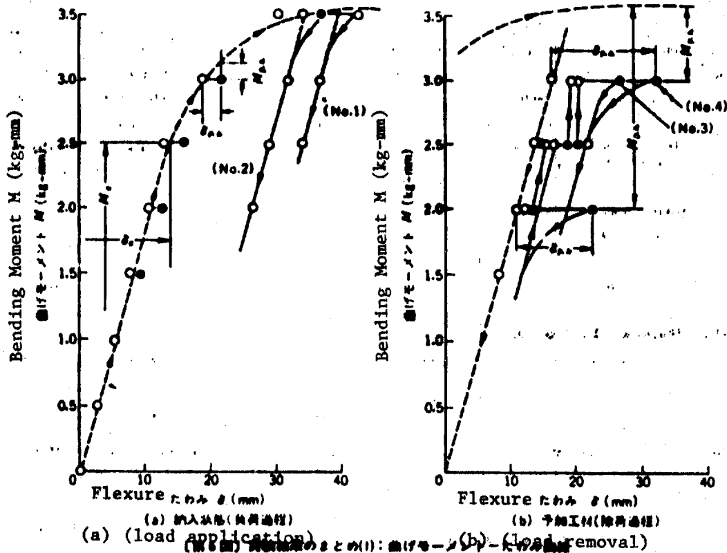
Diagram 6: Compiled results (1): Bending Moment- Flexure Curve
