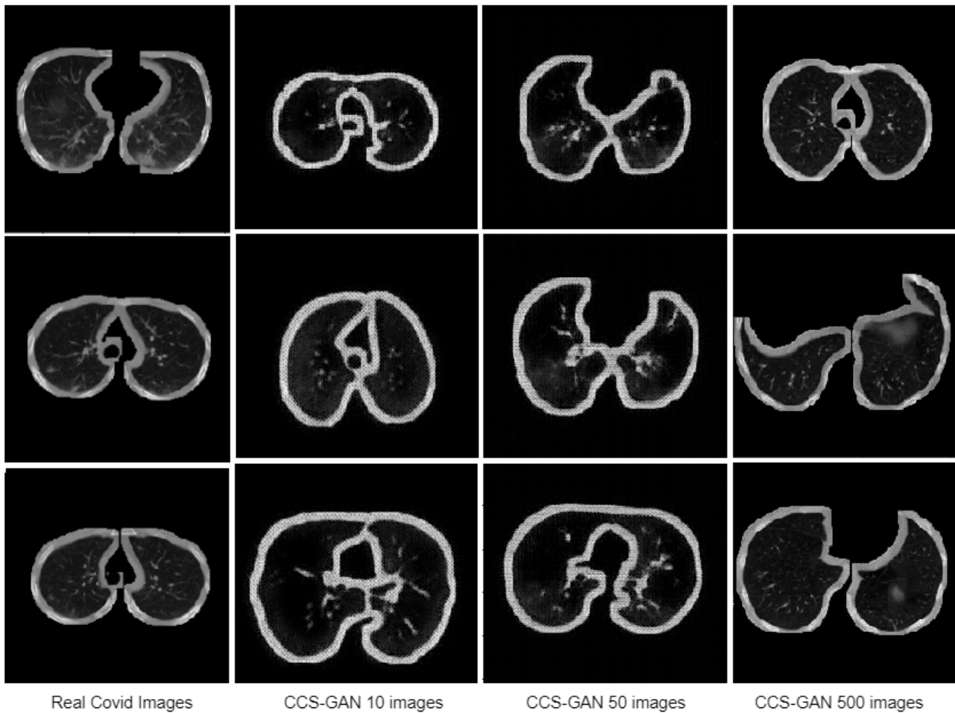
Fig. 5: Results
