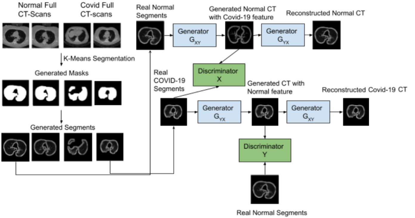
Fig. 1: CCS-GAN Approach
