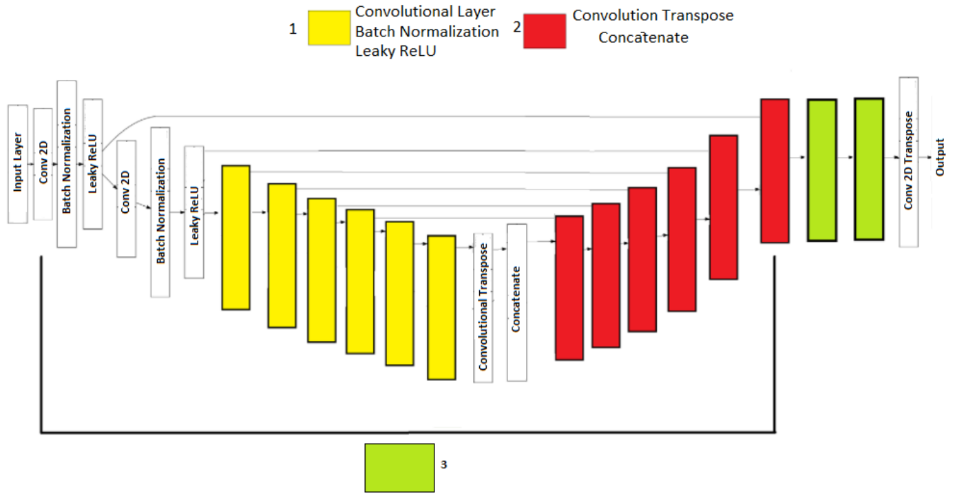
Fig. 3: Generator Architecture
