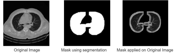
Fig. 2: Pulmonary Segmentation
