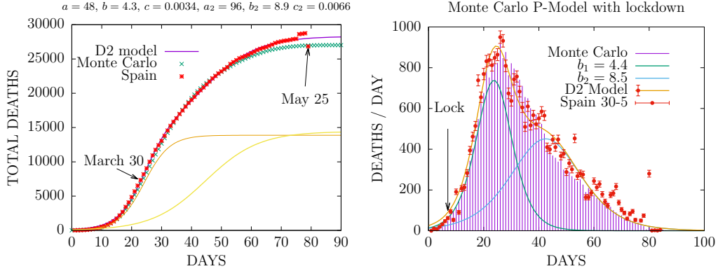
Figure 1: Fit of the P-model to the cumulative deaths and deaths per day by COVID-19 in Spain during the first wave. The red points are the data compiled up to May 25, 2020. The two yellow lines in the left panel are the two D-functions appearing in the D2 model, Eq. (7).
