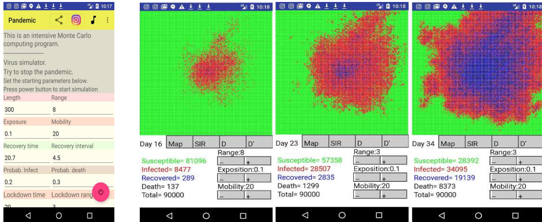
Figure 4: Monte Carlo Plank model simulator for Androids illustrating how the pandemic spreads in a lattice of length L = 300 – which corresponds to a population of L^2 = N = 90000 – as a function of time.
