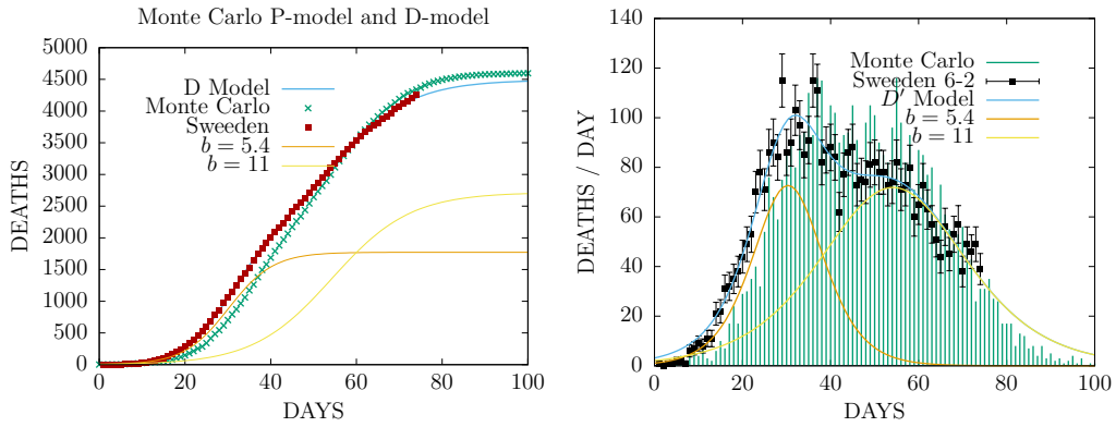
Figure 2: Fit of the P-model to the cumulative deaths and deaths per day by COVID-19 in Sweden during the first wave.
