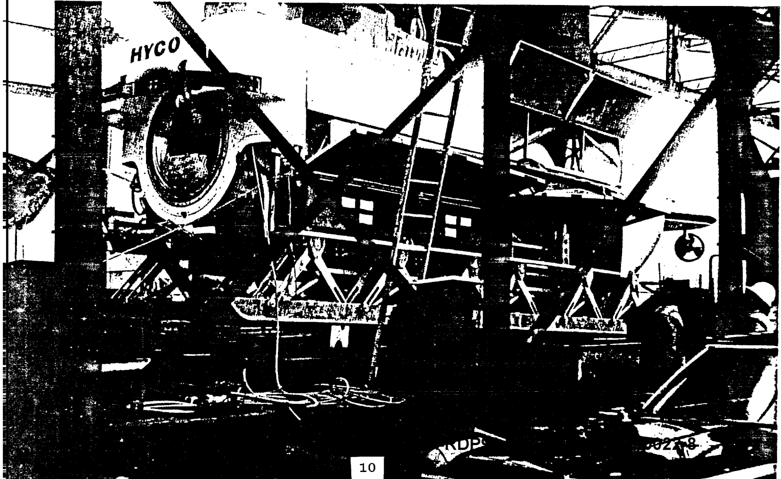
Frontal view of TAURUS engaged in dry transfer of oilmen into a seabed equipment chamber.
